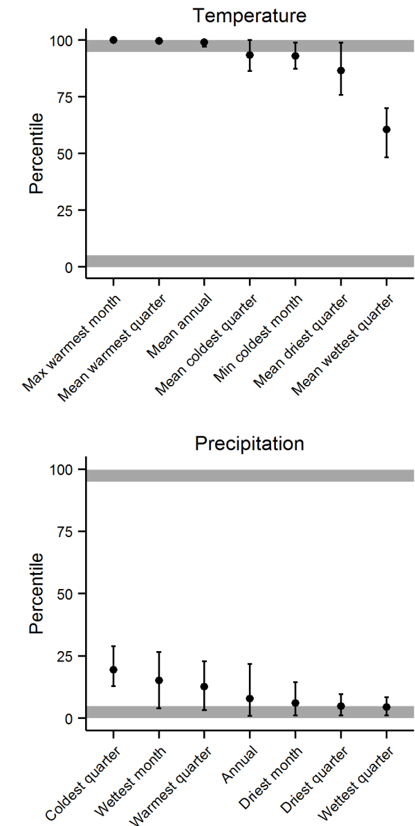
Figure 2. Recent temperature and precipitation percentiles at Petrified Forest National Park (including areas within 30-km [18.6-mi] of the park’s boundary). Black dots indicate average recent percentiles across the 10, 20, and 30-year intervals (moving windows). Variables are considered “extreme” if the mean percentiles are <5 th percentile or >95 th percentile (i.e., the gray zones, where recent climate is pushing the limits of all observed climates since the year 1901). Black bars indicate the range of recent percentiles across 10, 20, and 30-year moving windows (larger bars indicate higher sensitivity to moving window size).
