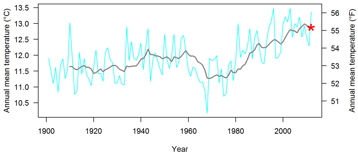
Figure 1. Time series used to characterize the historical range of variability and most recent percentile for annual mean temperature at Petrified Forest National Park (including areas within 30-km [18.6-mi] of the park’s boundary). The blue line shows temperature for each year, the gray line shows temperature averaged over progressive 10-year intervals (10-year moving windows), and the red asterisk shows the average temperature of the most recent 10-year moving window (2003–2012). The most recent percentile is calculated as the percentage of values on the gray line that fall below the red asterisk (see results of most recent percentiles for all temperature and precipitation variables in Figure 2).
