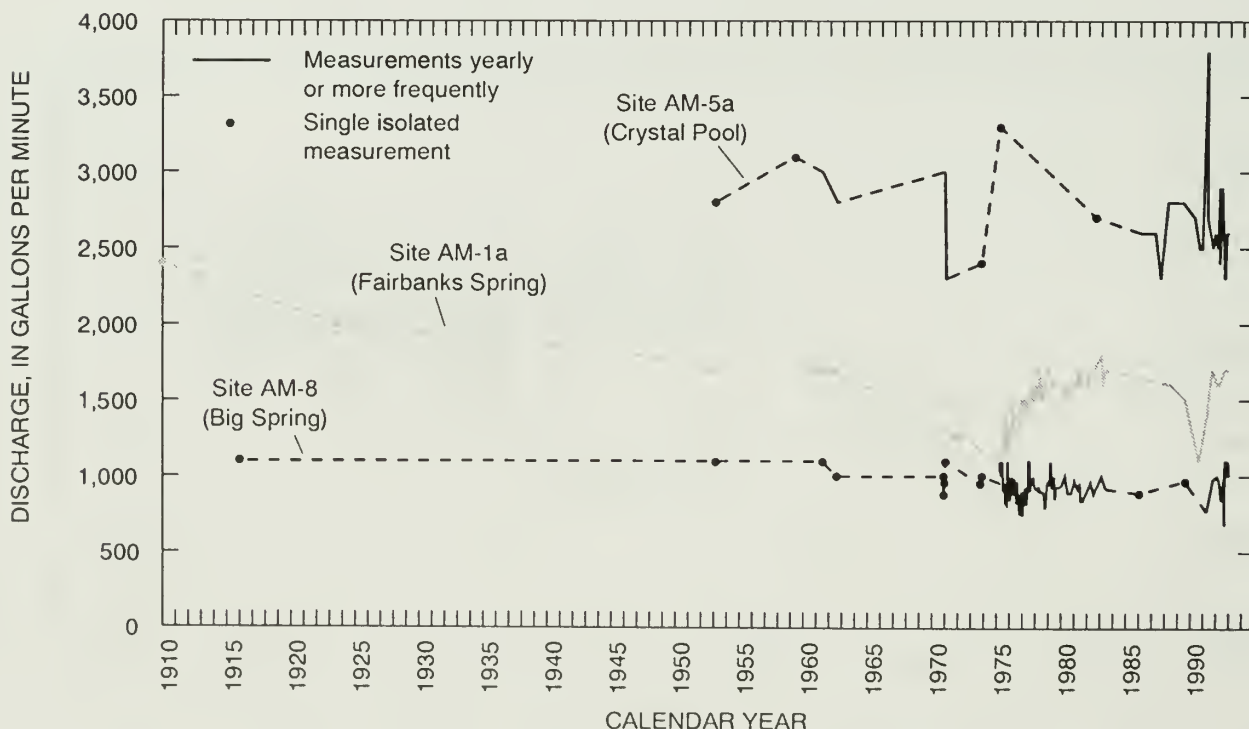
Figure 7. Discharge at sites AM-1a (Fairbanks Spring), AM-5a (Crystal Pool), and AM-8 (Big Spring) through 1992. Lines connect discrete data listed in table 5, and are dashed where measurements were not available for consecutive calendar years
