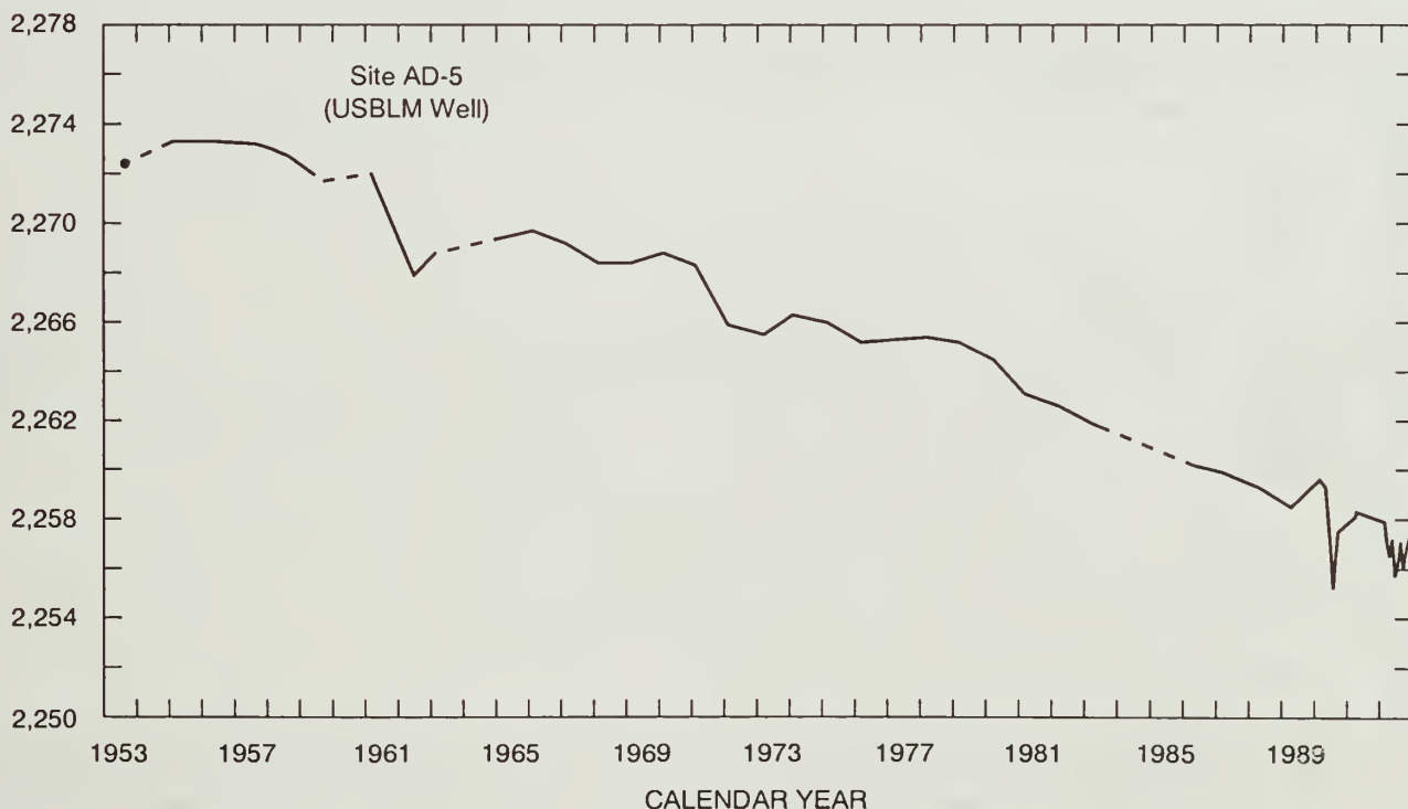
Figure 3. Water-level altitude through 1992 for selected wells at which primary contributing units are valley fill. Lines connect discrete data listed in table 2, and are dashed where measurements were not available for consecutive calendar years. Data noted with water-level status of P, R, S, and I have been excluded, as those data may represent transient conditions at a site.
