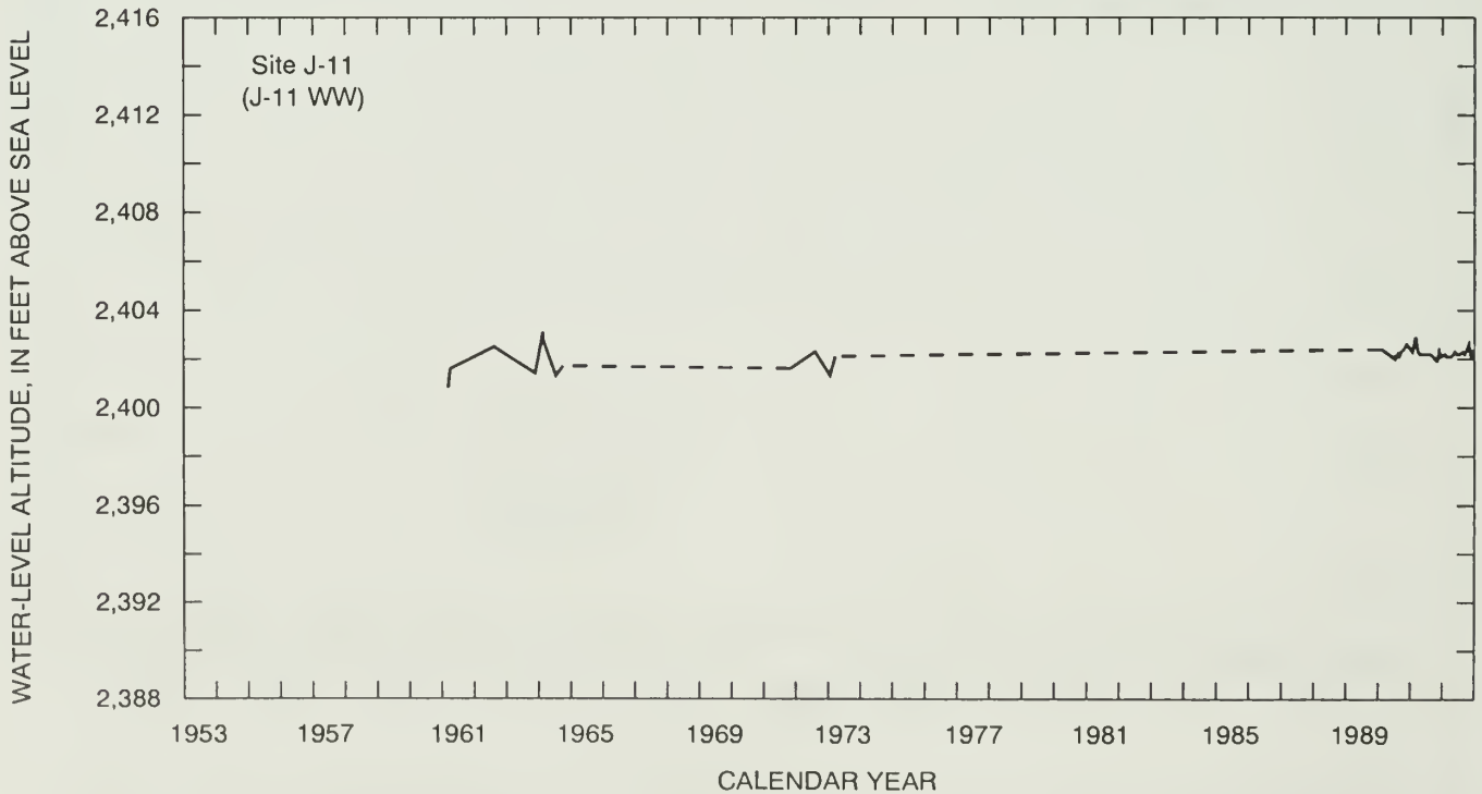
Figure 2 Water-level altitude through 1992 for selected wells at which primary contributing units are volcanic rock. Lines connect discrete data listed in table 2, and are dashed where measurements were not available for consecutive calendar years.
