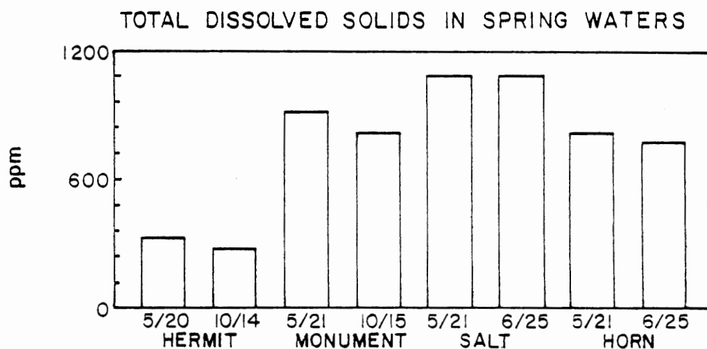
Figure 8.-TDS in spring waters during study (1983).
