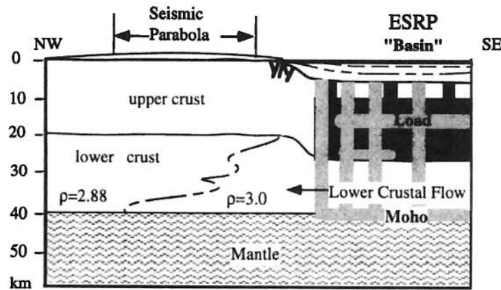
Figure 16. Summary Figure of ESRP and Basin and Range depicting features and timing of downwarping. These include (1) an extensive midcrustal load emplaced at ~10 Ma (solid area); (2) a post-Neogene load related to the volcanic rift zones (VRZ) (shaded area); (3) 5-8 km of downwarped Basin and Range crust; (4) a NE striking fault set due to flexure of the crust [Zentner, 1989b]; (5) an angular unconformity between the downwarped fold hinges and Heise volcanic rocks (dashed lines); (6) flat Moho; and (7) lower crustal flow from beneath the ESRP to the extending Basin and Range (seismic parabola).
