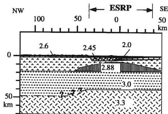
Figure 6. Crustal and upper mantle model of the ESRP and adjacent Basin and Range from seismic and gravity surveys after Sparlin et al. [1982]. There is no vertical exaggeration. Densities are in \text{g cm}^{-3} .
