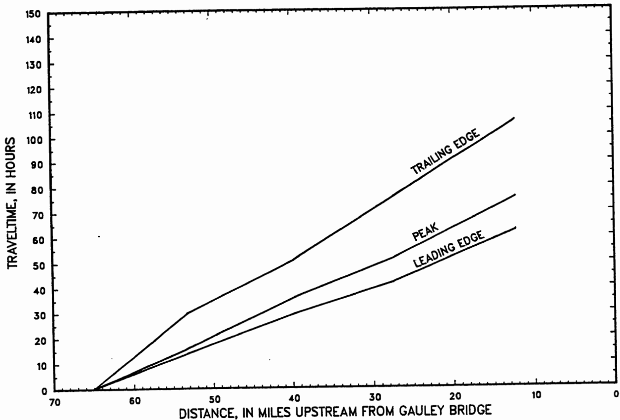
Figure 5.--Traveltime-distance relations for river flow of 2,200 cubic feet per second.
