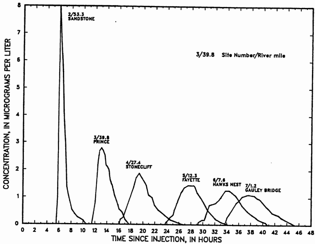
Figure 4.--Observed time-concentration curves for the May 1986 study.
