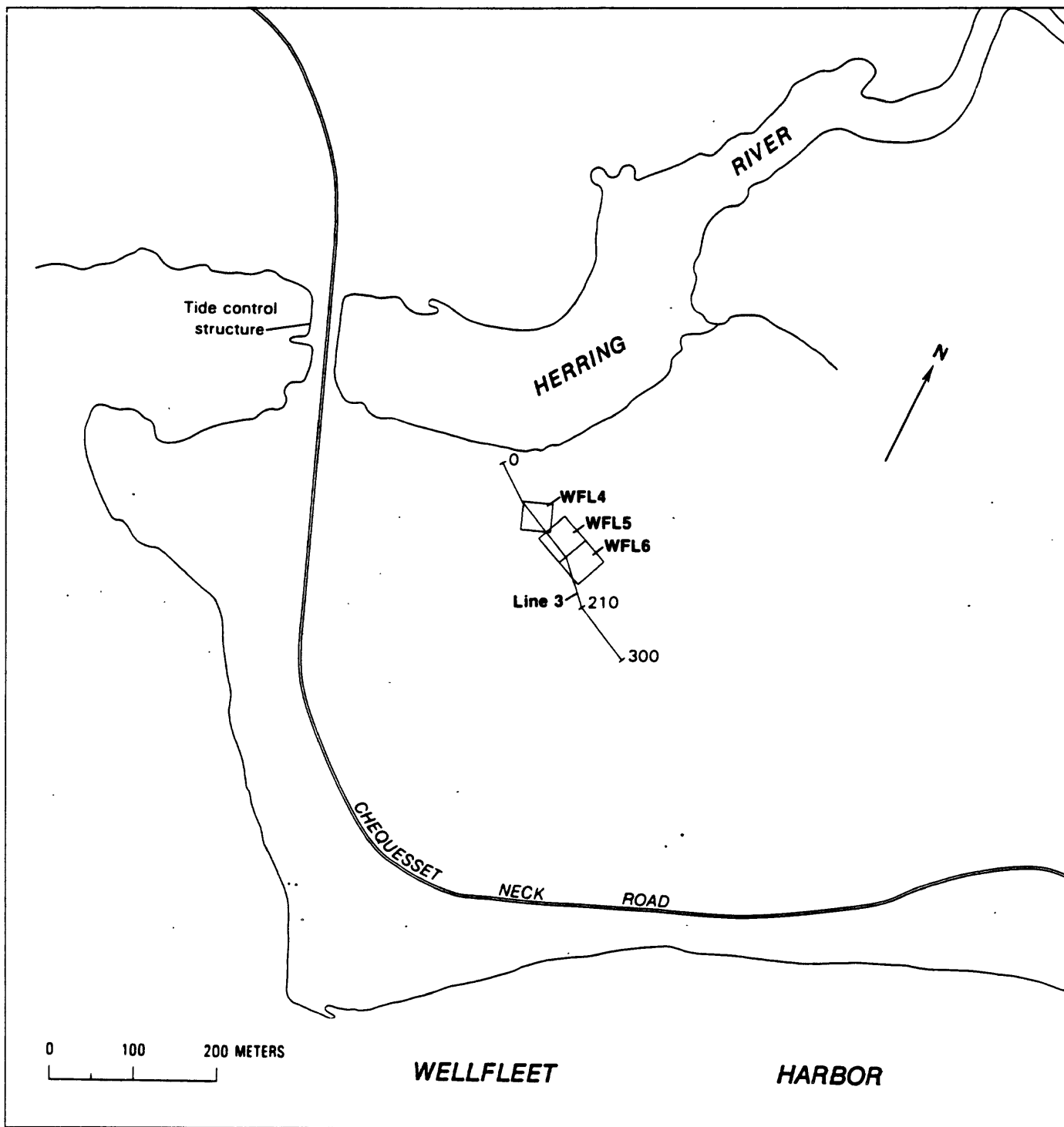
Figure 9 Chequeset Neck traverse location map showing survey line and TEM sounding loops. The numbers along the geophysical line are station numbers in meters.
