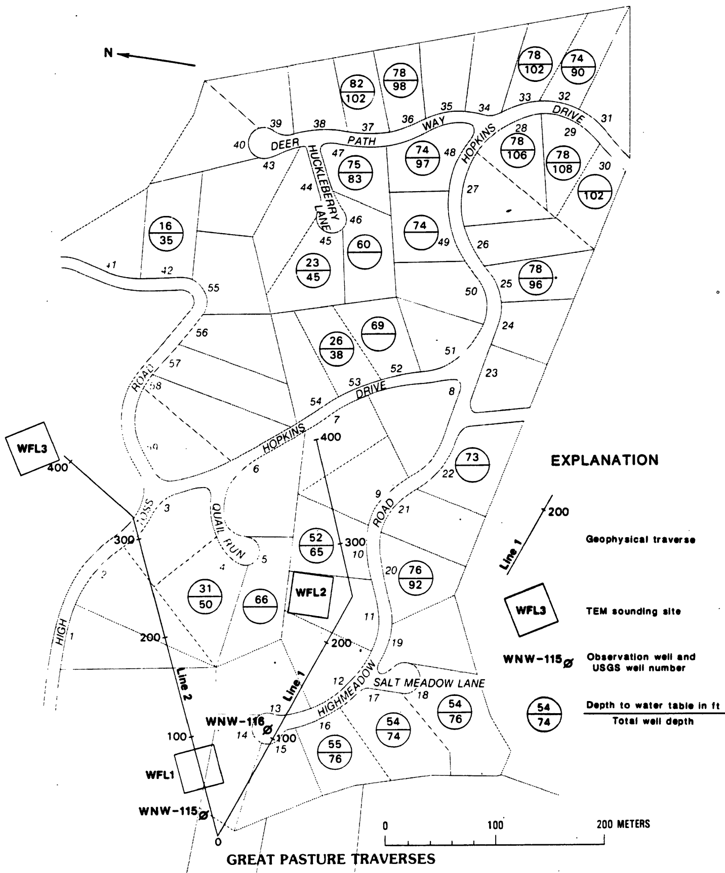
Figure 2 Great Pasture traverse location map showing survey lines, TEM sounding loops (large squares), and observation wells. The circled numbers are the depths to the water table (upper number) and total well depth (lower number) in ft in domestic water wells. The gray numbers and lines are lot numbers and property boundaries respectively. Exact location of the domestic well inside the property boundary is not known. The numbers along the geophysical lines are station numbers in meters.
