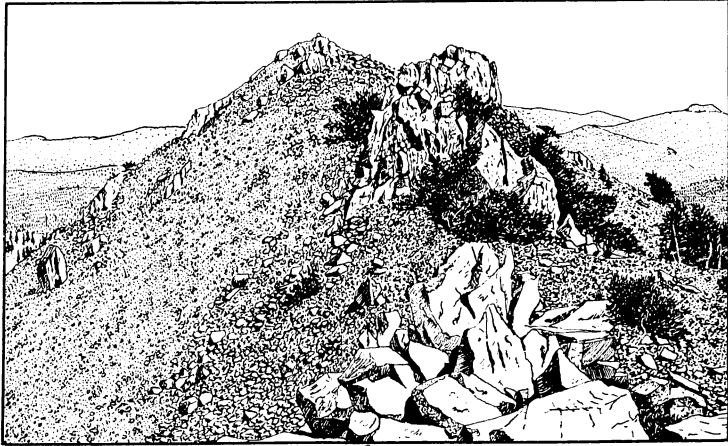
Fig. 3. The White Mountain Dome. a: looking east from the slopes of Lassen Peak, showing the great talus banks. b: east end of the ridge. The Central Plateau of augite andesite and Hat Mountain cone in the middle distance. In the background, from left to right, the dome and cone of Prospect Peak, the quartz basalt Cinder Cone and Fairfield Cone. c: part of the summit ridge, showing vertically jointed rock pinnacles protruding through coarse, angular talus blocks.
