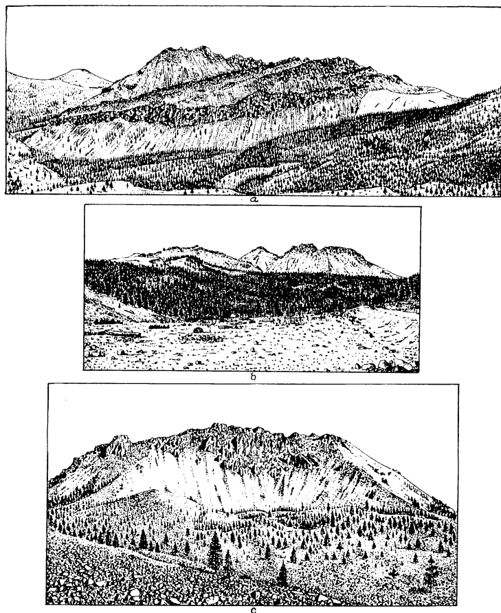
Fig. 2. The Chaos Crags. a: looking east. Shows ruined lapilli-cone and tuff-mantled hills in the foreground; also, the two dacite domes, the earlier well-banded and the later structureless. b: looking west. Shows the moat between the domes and the long talus banks. In the foreground is part of the 1915 mud-flow from Lassen Peak. c: looking south. Shows the craters at the northern base of the later dome and part of the avalanche-deposit, the Chaos Jumbles.
