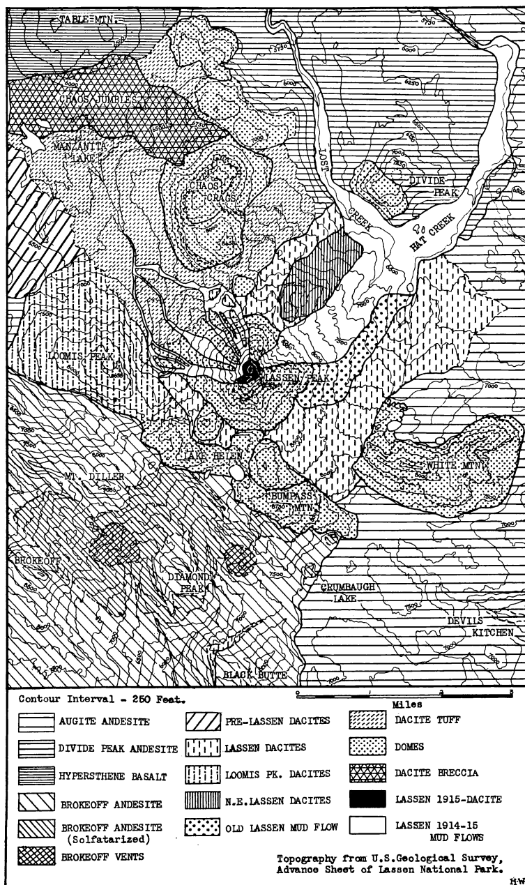
Fig. 1. Geologic sketch-map of Lassen Peak and vicinity.
