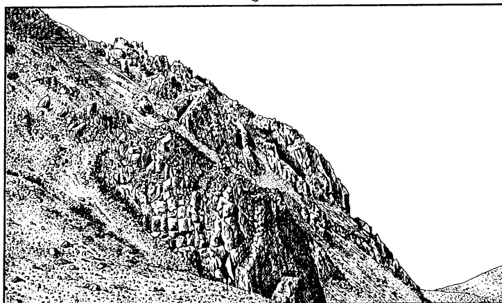
Fig. 4. The Dome of Lassen Peak. a: south slope from above Lake Helen, showing smooth sides of the plug-dome and concentric banks of talus. b: nearer view of the smooth face of the dome, showing the rounded form and fine vertical striation; height of cliff, about 500 feet. c: crags near the summit, southeast side, showing vertical joints and long talus slides.
