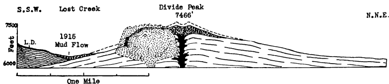
Fig. 5. Section through Divide Peak andesite cone and dacite dome. The summit of the former consists chiefly of bedded pyroclastic rocks. Flows of glassy dacite from the crater on the N. E. flank of Lassen Peak (L. D.) overlie the andesites on the south.
