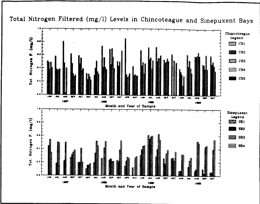
Figure 49. Seasonal Total Nitrogen Filtered Distribution in the Chincoteague-Sinepuxent Bay Complex.
