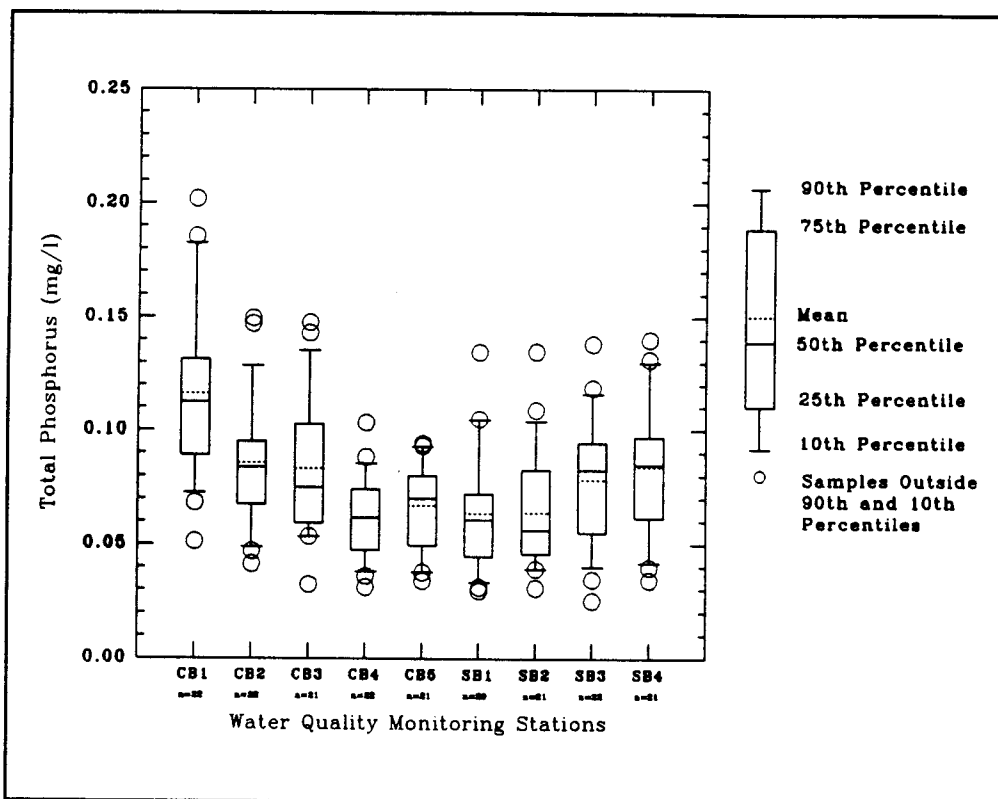
Figure 56. Total Phosphorus Distributions in the Chincoteague-Sinepuxent Bay Complex.
