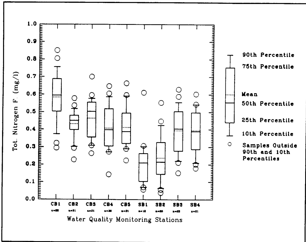
Figure 50. Total Nitrogen Filtered Distributions in the Chincoteague-Sinepuxent Bay Complex.
