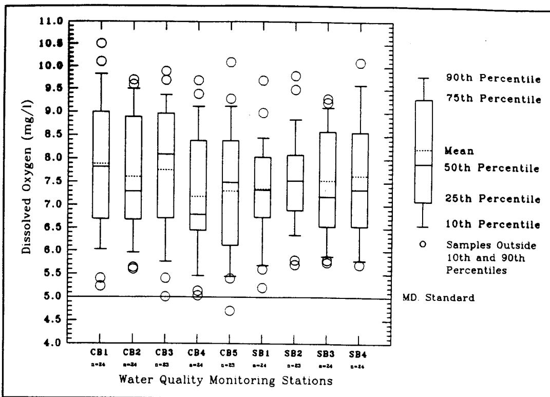
Figure 8. Dissolved Oxygen Distributions in Chincoteague-Sinepuxent Bay Complex.
