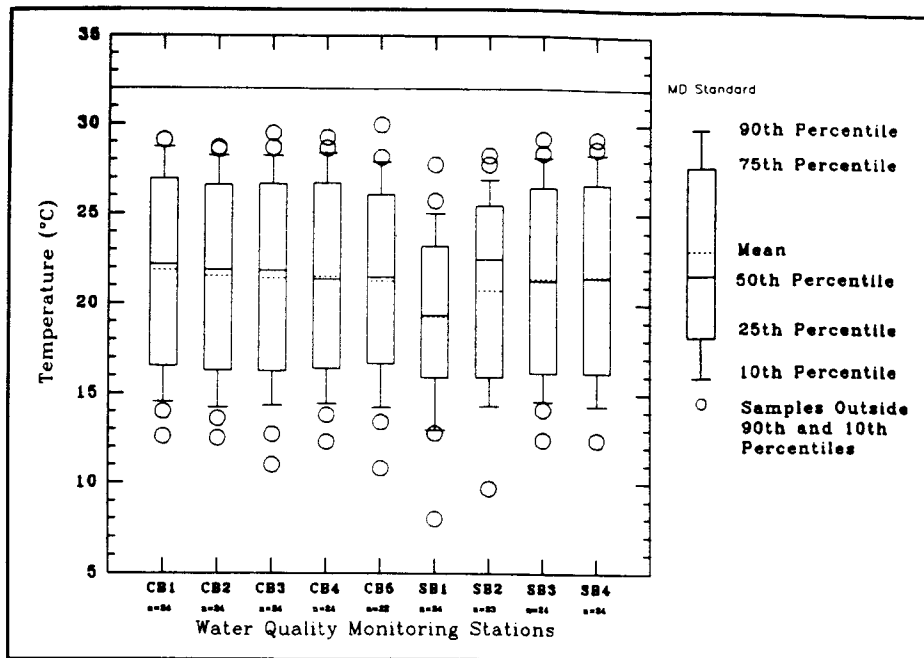
Figure 5. Water Temperature Distributions in Chincoteague-Sinepuxent Bay Complex.
