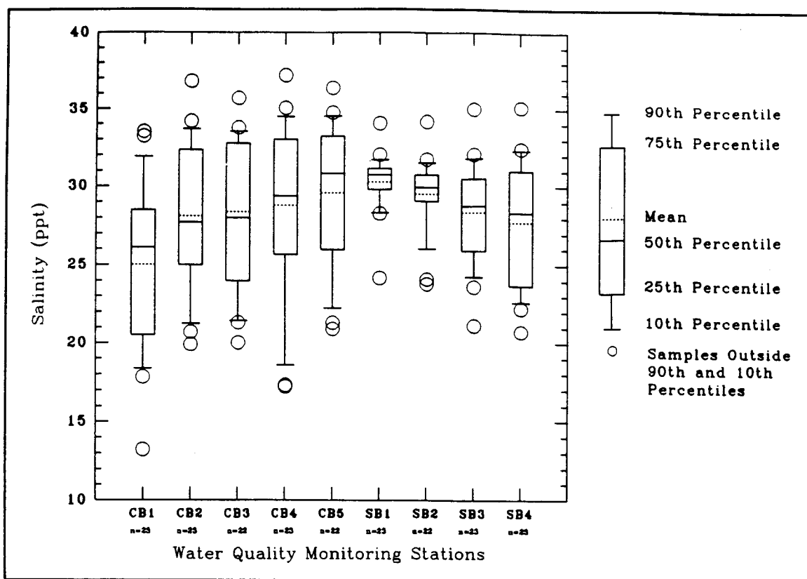
Figure 11. Salinity Distributions in the Chincoteague-Sinepuxent Bay Complex.
