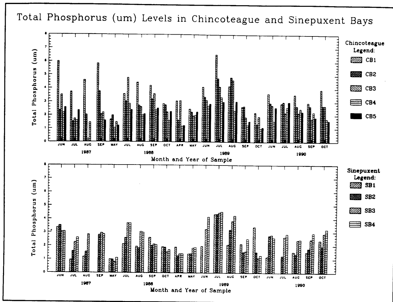
Figure 36. Seasonal Total Phosphorus Distribution in the Chincoteague-Sinepuxent Bay Complex.
