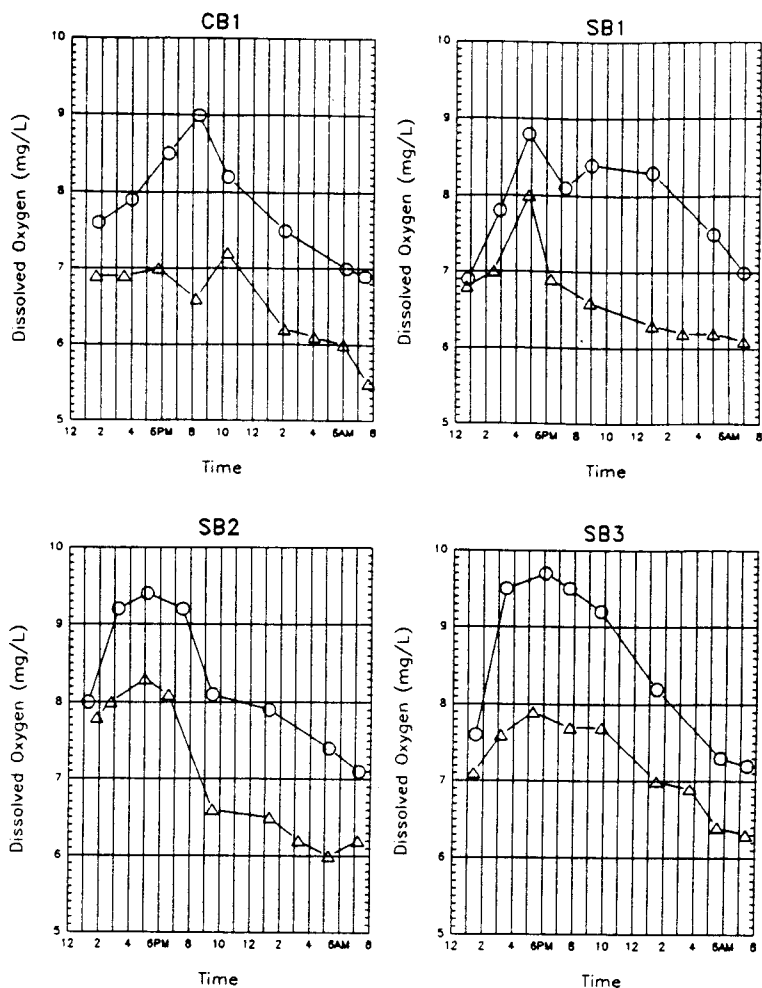
Figure 9. Diel Dissolved Oxygen During 6/19/89 – 6/20/89 and 8/01/89 – 8/02/89 in the Chincoteague-Sinepuxent Bay Complex
