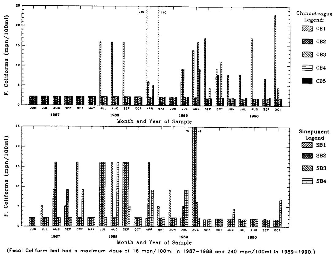
Figure 45. Seasonal Fecal Coliform Distribution in the Chincoteague-Sinepuxent Bay Complex.
