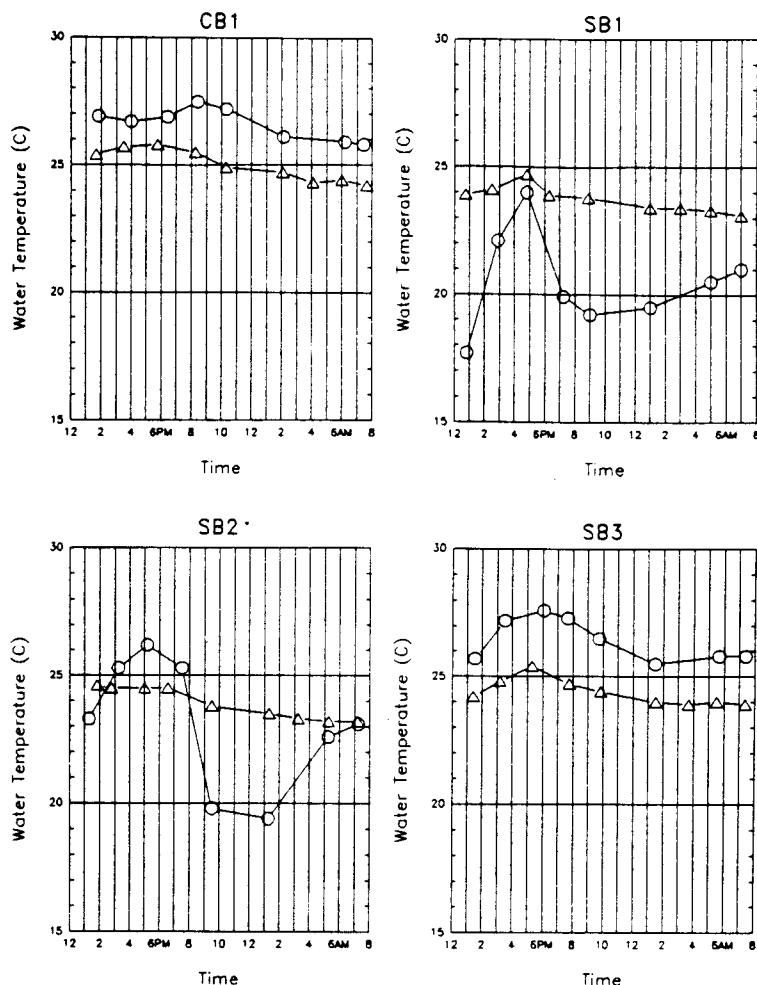
Figure 6. Diel Water Temperatures During 6/19/89 - 6/20/89 and 8/01/89 - 8/02/89 in the Chincoteague-Sinepuxent Bay Complex.
