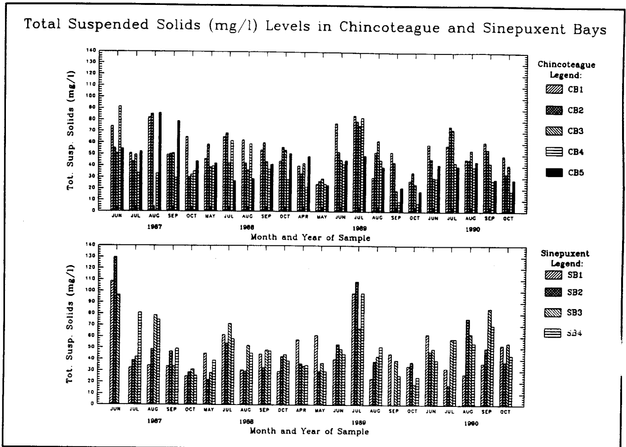
Figure 17. Seasonal TSS Distribution in the Chincoteague-Sinepuxent Bay Complex.
