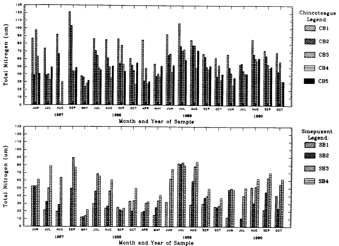
Figure 27. Seasonal Total Nitrogen Distribution in the Chincoteague-Sinepuxent Bay Complex.
