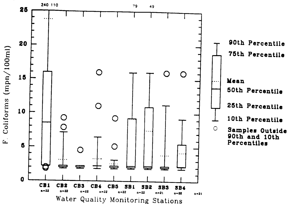
Figure 46. Fecal Coliform Distributions in the Chincoteague-Sinepuxent Bay Complex.
