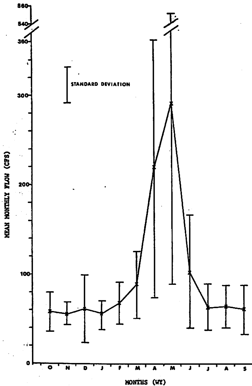
Figure 3 Mean monthly stream flow with standard deviations.
