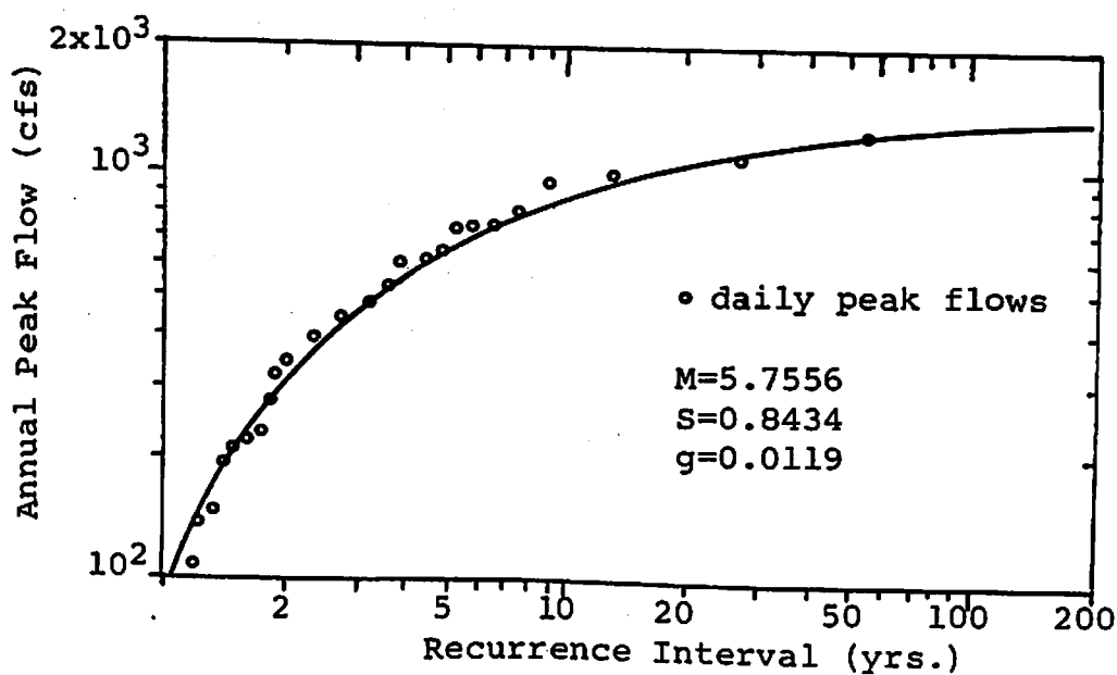
Figure 8. Flood Frequency, June 15 to September 30, for the North Fork of the Virgin River, near Springdale, Utah (USGS, 1923-1974). Log-Pearson Type III Distribution.
