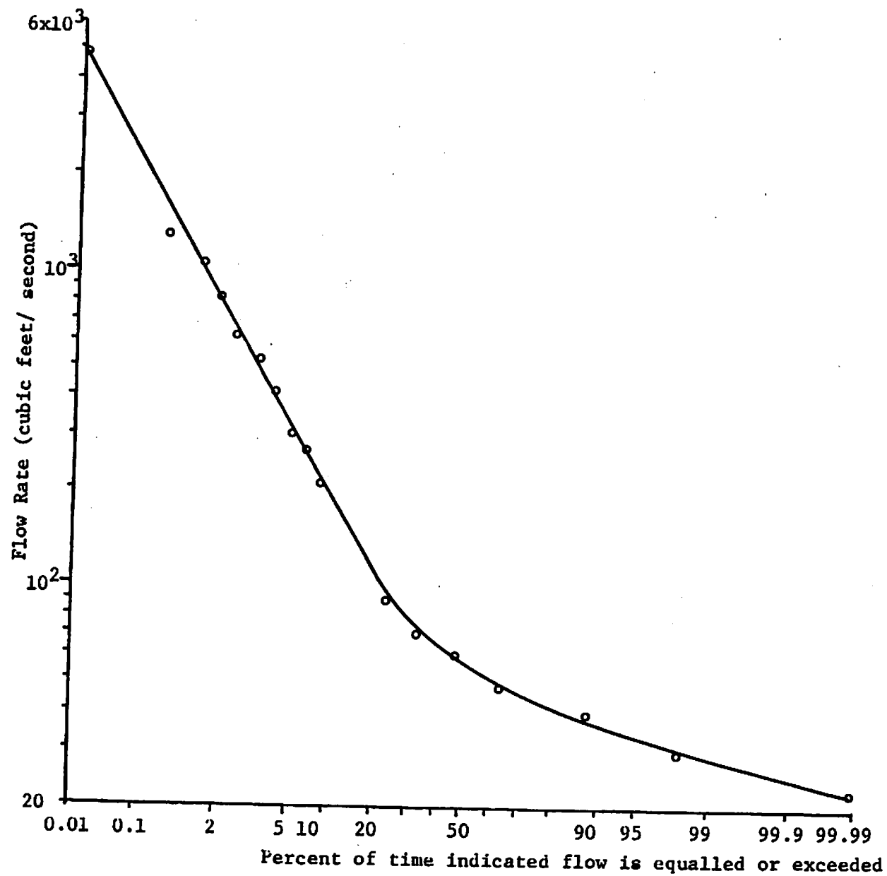
Figure 4. Flow duration curve for the North Fork of the Virgin River, near Springdale, Utah (USGS, 1923 to 1974).
