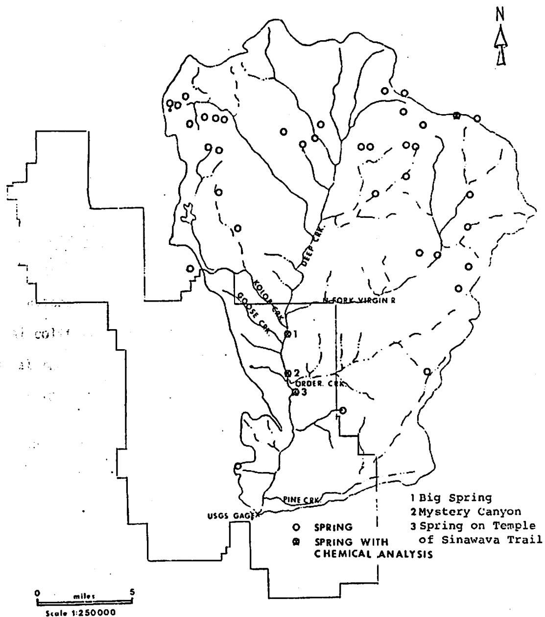
Figure 10. Nonthermal springs within the NFVR watershed as listed by the Utah Geological and Mineralogical Survey (WRB 16, 1971).
