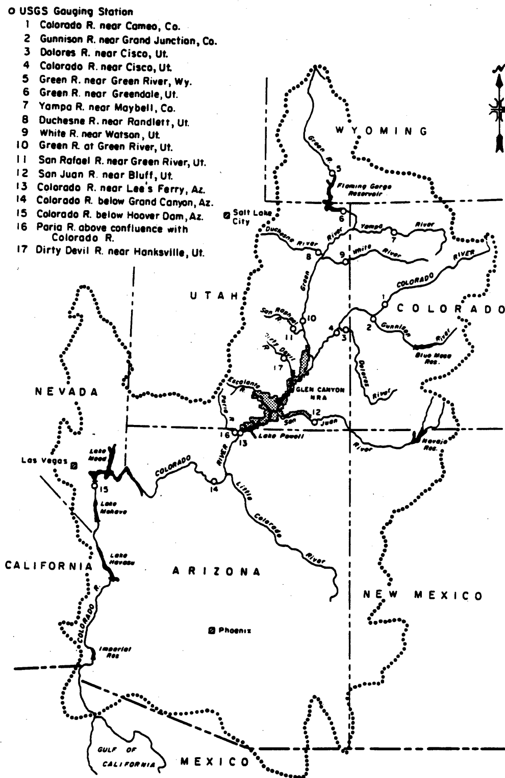
Fig. 2. Colorado River Basin, showing major tributaries, reservoirs, USGS gauging stations, and relative location of Glen Canyon National Recreation Area. (Adapted from Moody and Mueller, 1984.)
