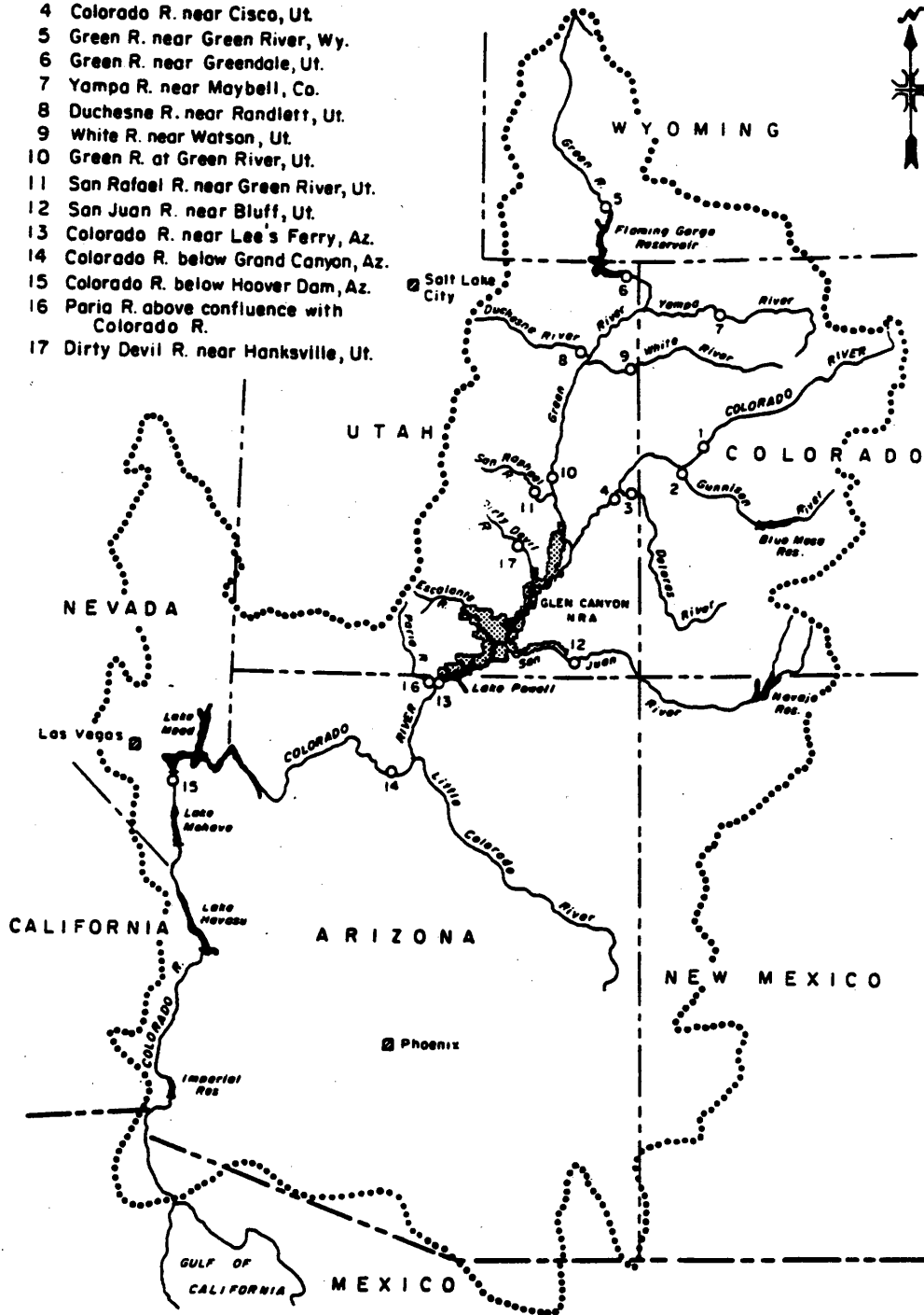
Fig. 2. Colorado River Basin, showing major tributaries, reservoirs, USGS gauging stations, and relative location of Glen Canyon National Recreation Area. (Adapted from Moody and Mueller, 1984.)
