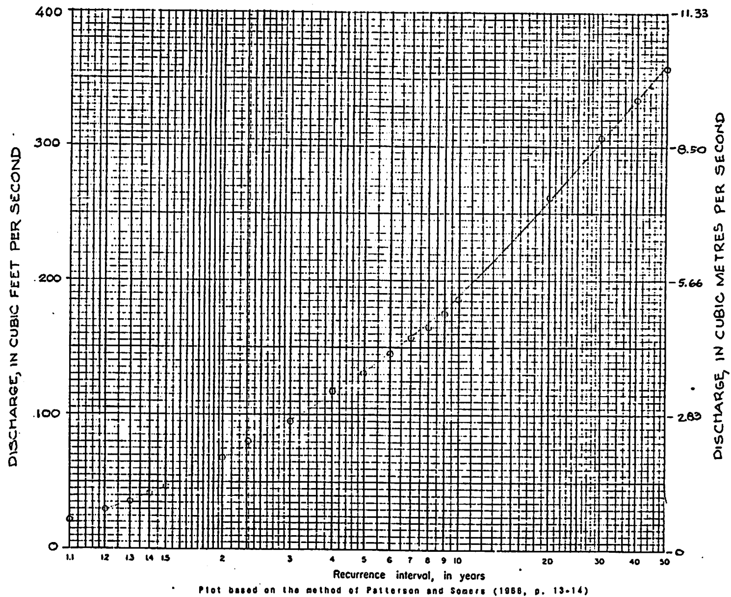
Figure 7.--Flood-frequency curve, Cub Creek near Jensen, Utah.
