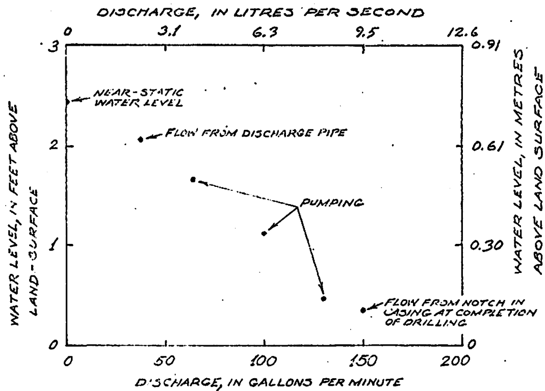
Figure 11.--Relationship of discharge to water level in Echo Park well 3.
