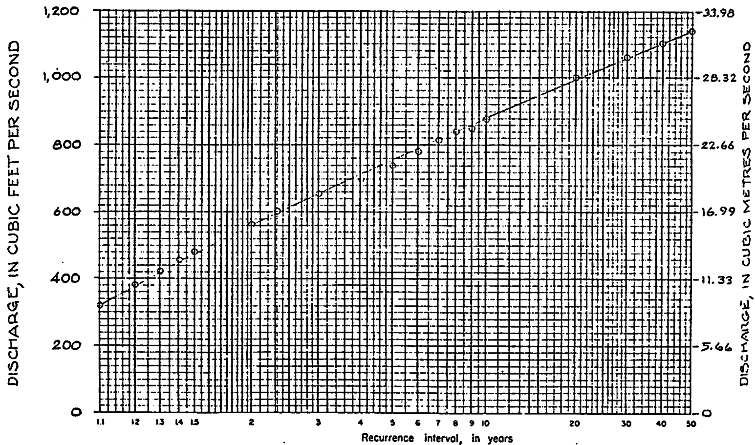
Figure 6.--Flood-frequency curve, Jones Hole Creek near Jensen, Utah.
