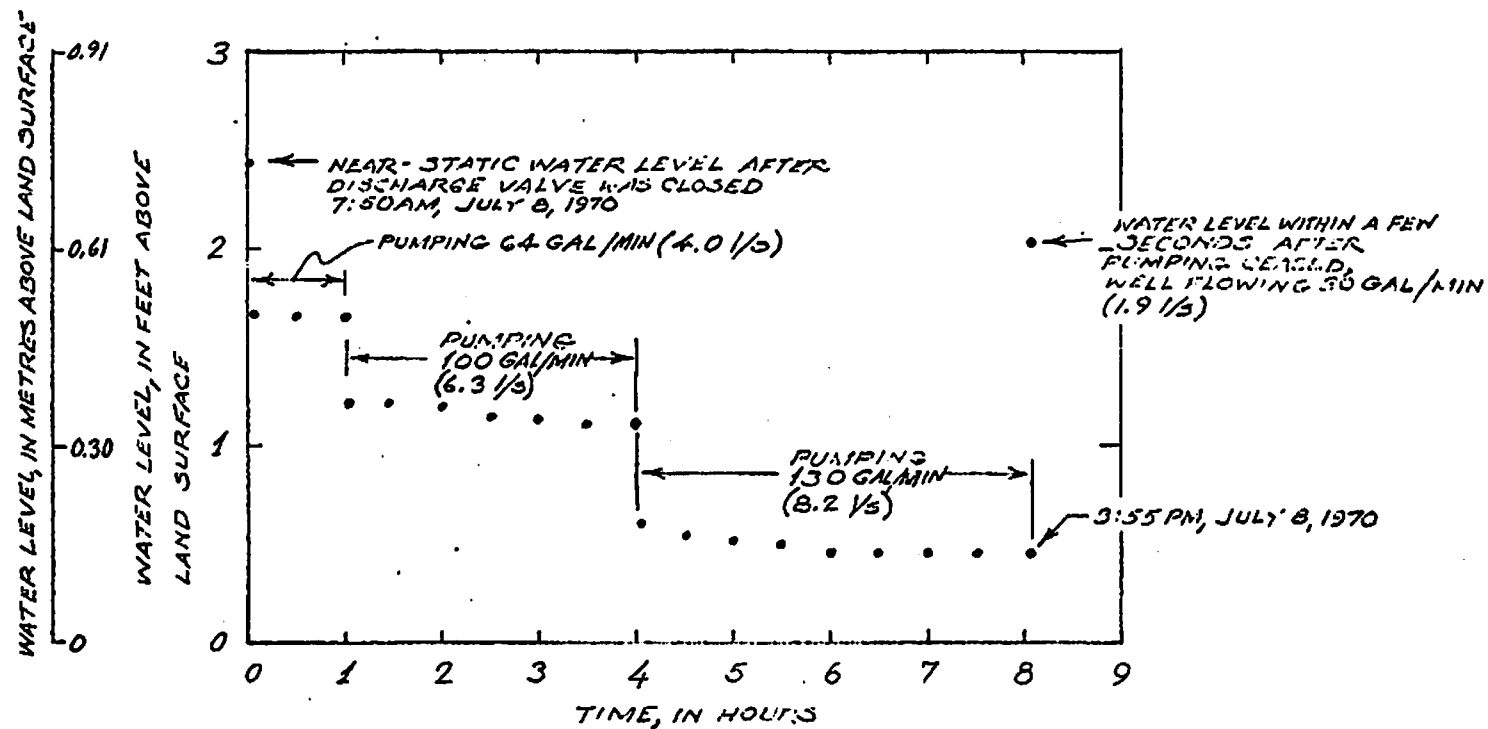
Figure 10.--Drawdown while pumping and recovery of the water level after Pumping ceased at Echo Park well 3.
