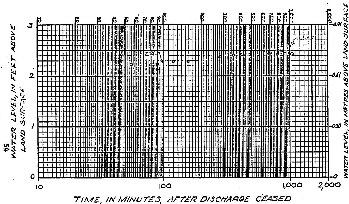
Figure 9.--Recovery curve at Echo Park well 3 showing calculation of transmissivity.
