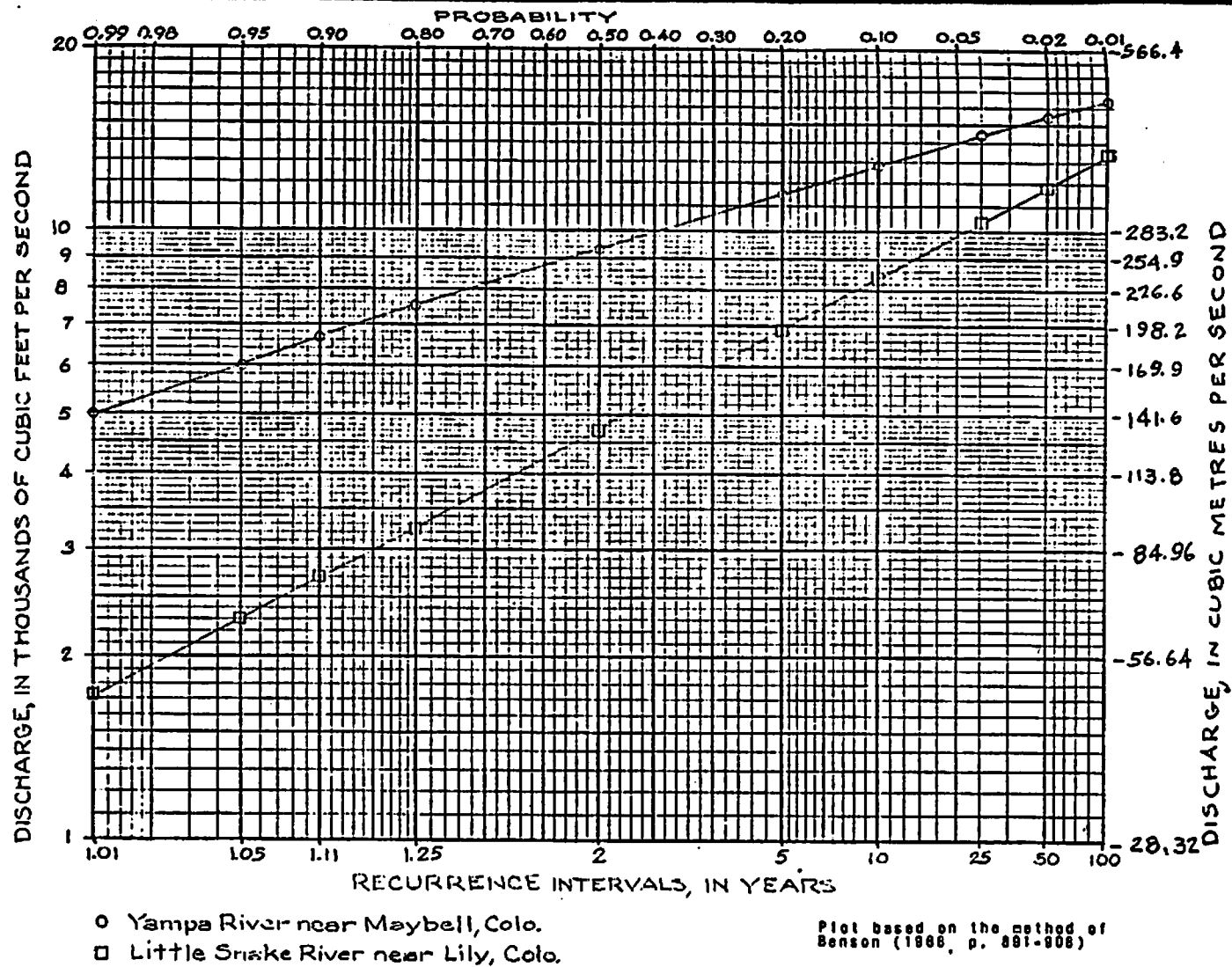
Figure 4.--Flood-frequency curves, Yampa River near Maybell and Little Snake River near Lily, Colo.
