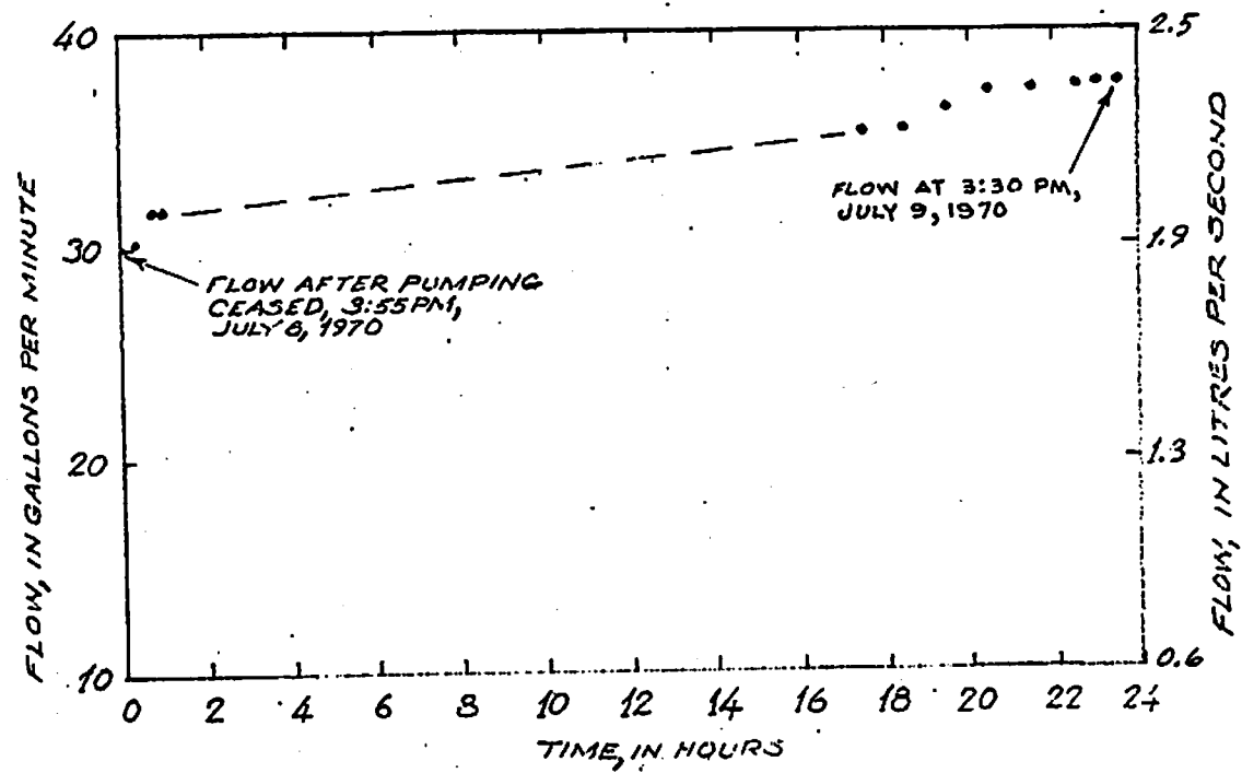
Figure 12.--Increase in artesian flow after pumping ceased at Echo Park well 3.
