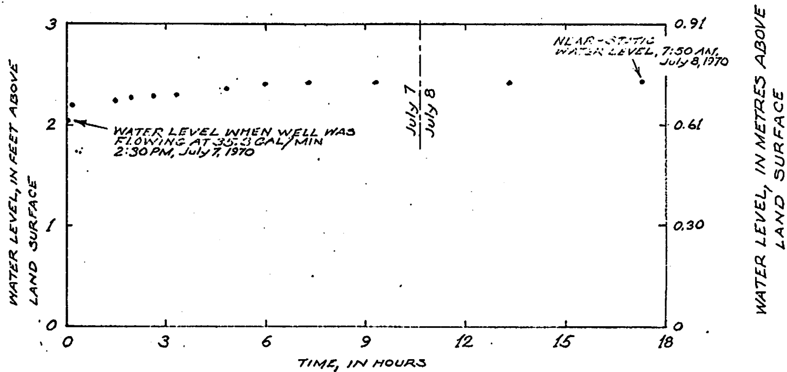
Figure 8.--Recovery of artesian pressure at Echo Park well 3, July 7-8, 1970.
