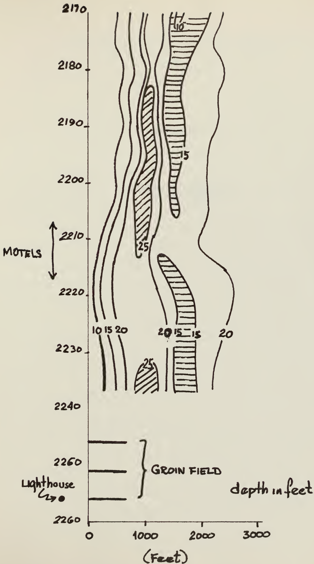
Fig. 12. Nearshore bathymetry in the nourishment area.
