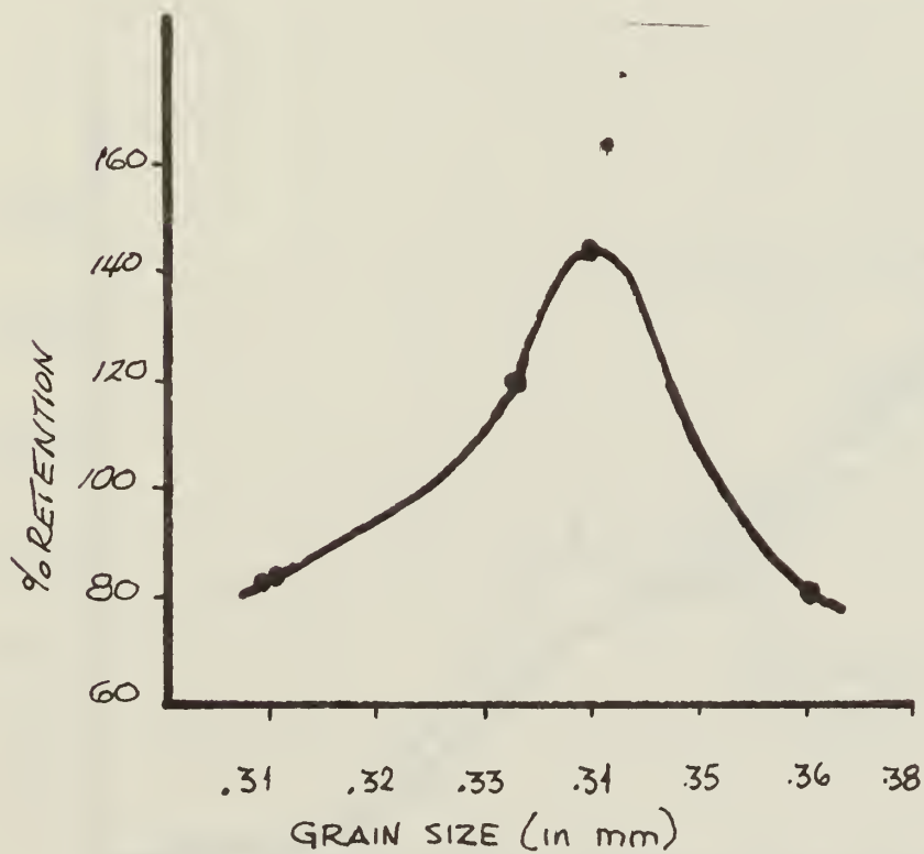
Fig. 6. Percentage retention of fill by grain size of discharge material.
