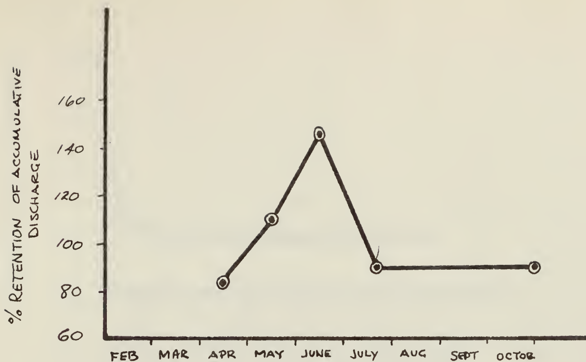
Fig. 7. Accumulative percentage retention of the fill for five intervals during the pumping period.
