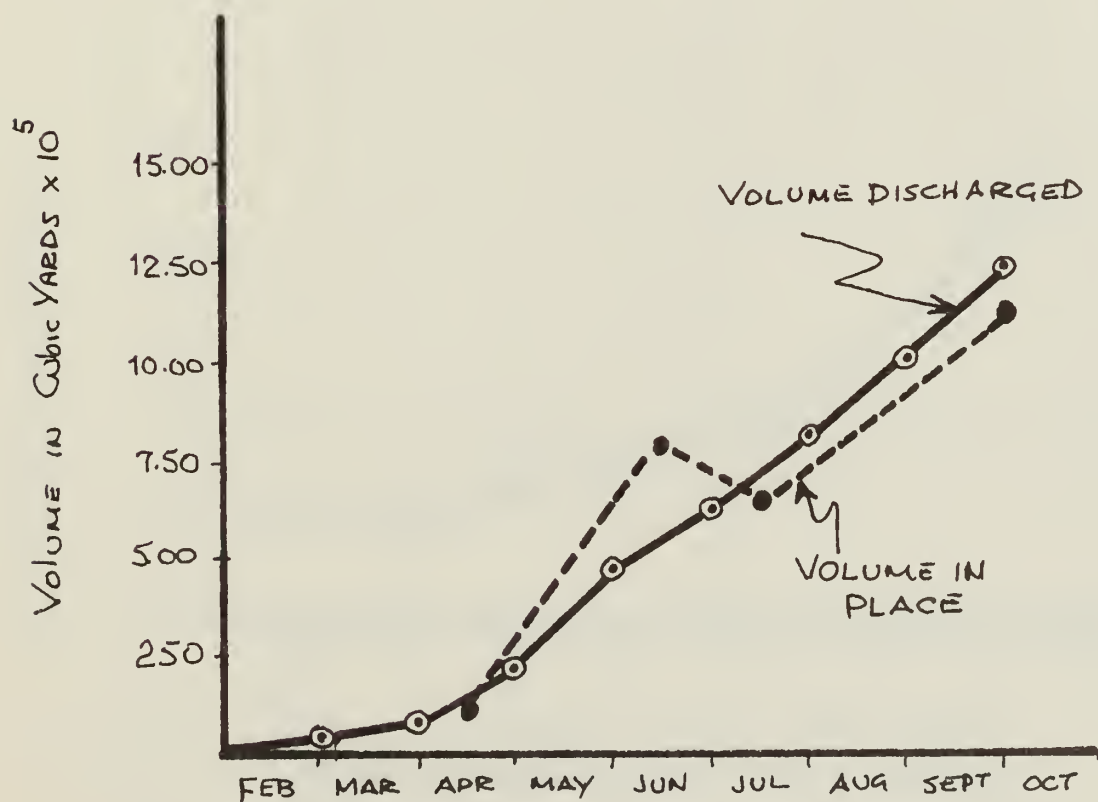
Fig. 8. Discharge volume corrected for percentage retention of the fill.
