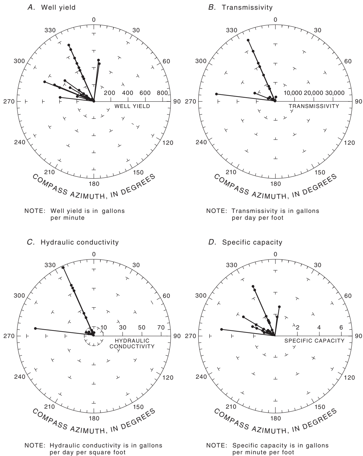
Figure 54. Relation of data from well and aquifer tests to structural orientation of surface geology, Flagstaff, Arizona. A , Well yield. B , Transmissivity. C , Hydraulic conductivity. D , Specific capacity.
