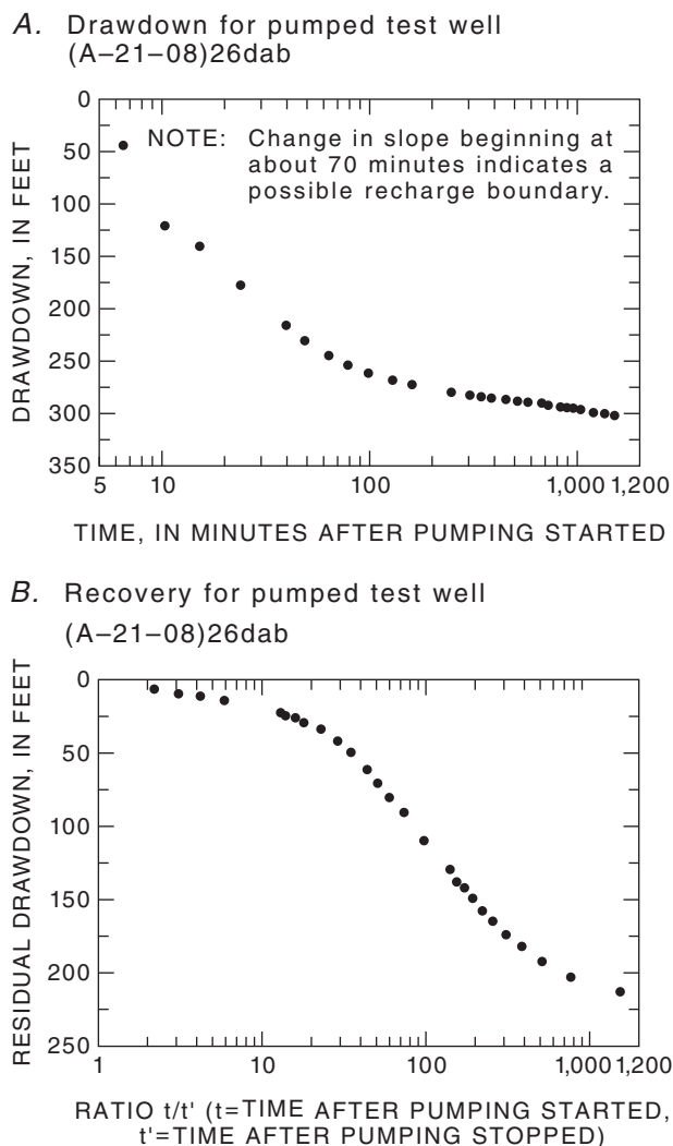
Figure 43. Drawdown and recovery data for a typical well test in the Flagstaff area. A, Walnut Canyon well. B, Recovery, Wlanut Canyon well.
