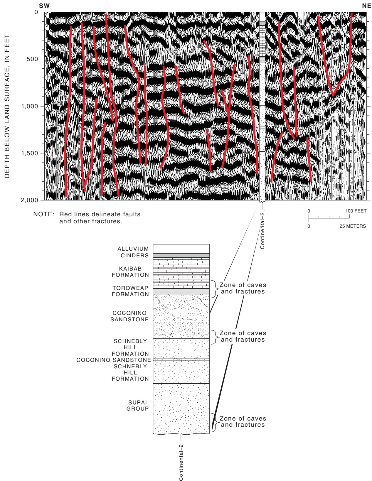
Figure 34. Stacked seismic image along Continental line 2.
