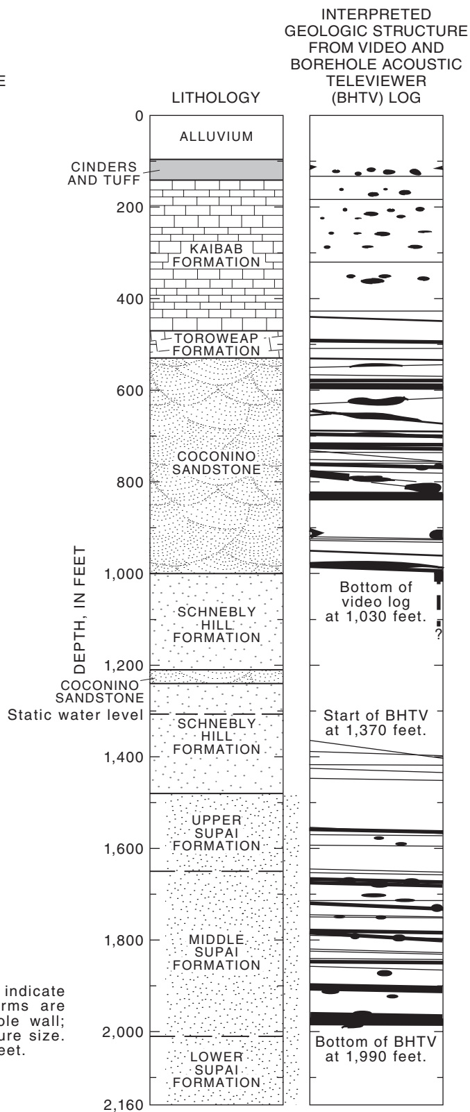
Figure 38. Lithologic and borehole-geophysical logs, Continental site. A, Well 1. B, Well 2.
