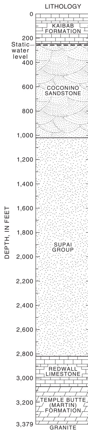
Figure 18. Lithologic and borehole-geophysical logs, Lake Mary sites. A, Well LM-6. B, Well LM-7. C, Well LM-8. D, Well LM-9.
