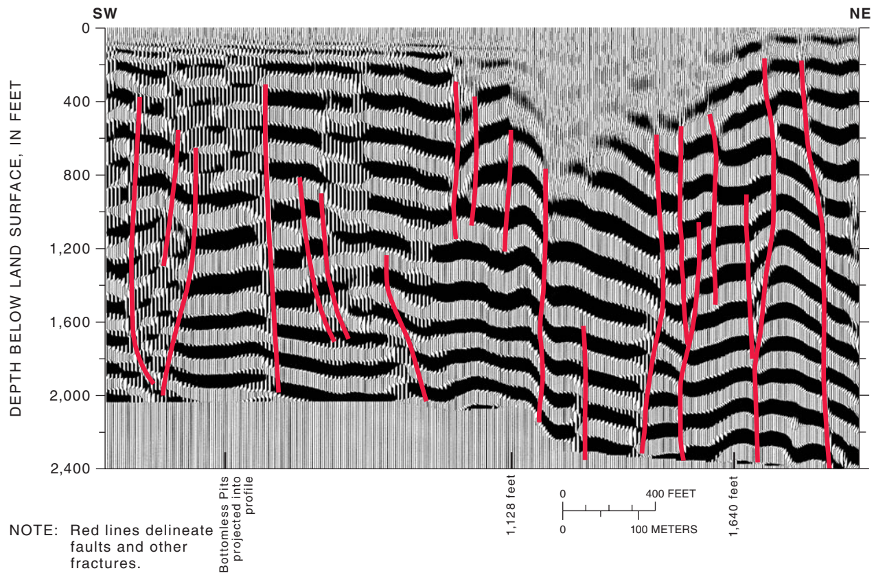
Figure 33. Stacked seismic image along Continental line 1. Low-frequency reflectors continuous over distances of several tens of feet are presumed to correspond to major layers within the subsurface. Vertical offsets in the apparent layers are presumed to be faults. Areas with blurred or missing reflectors in the southwestern half of the section correlate with the location of the Bottomless Pits solution caverns. Missing reflectors in the upper 656 feet from 1,128 to 1,640 feet correspond to an area where surface-shot points were skipped because of locally steep topography.
