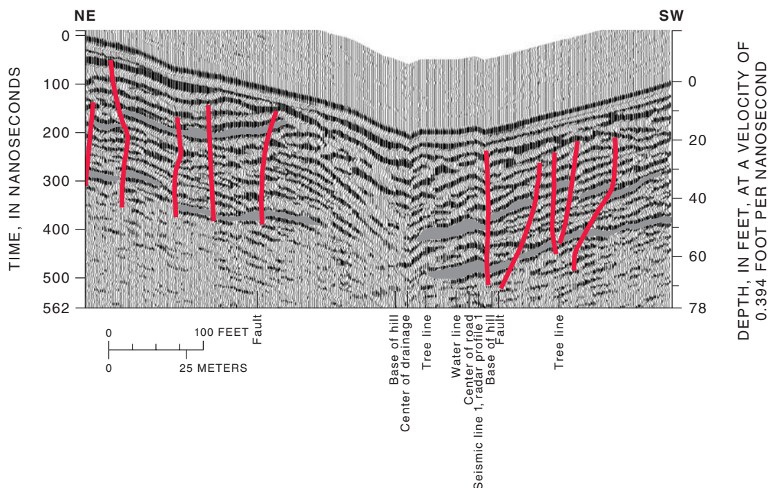
Figure 22. Selected interpreted ground-penetrating radar data for the Skunk Canyon area. A, Radar profile 1, 0–300 feet. B, Radar profile 2, 0–620 feet. C, Radar profile 3, 0–600 feet. Interpreted fractures are shown in red, and interpreted bedding planes are gray fills. Hyperbolic events are interpreted as small openings or open horizontal fractures in between bedding planes.
