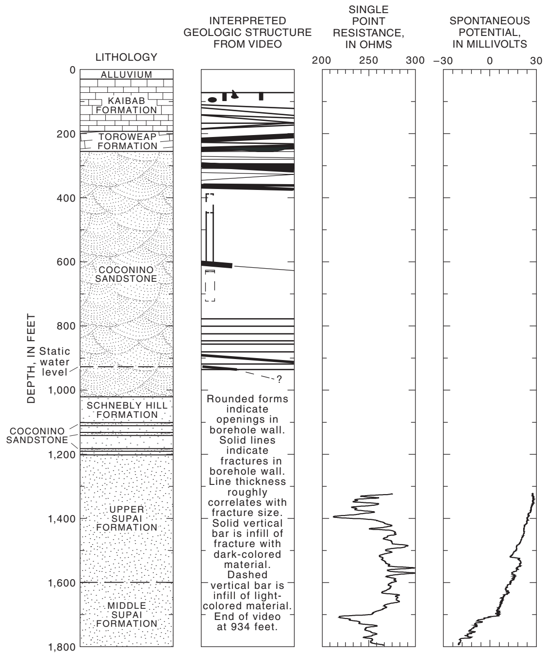
Figure 25. Lithologic and borehole-geophysical logs, Skunk Canyon well.
