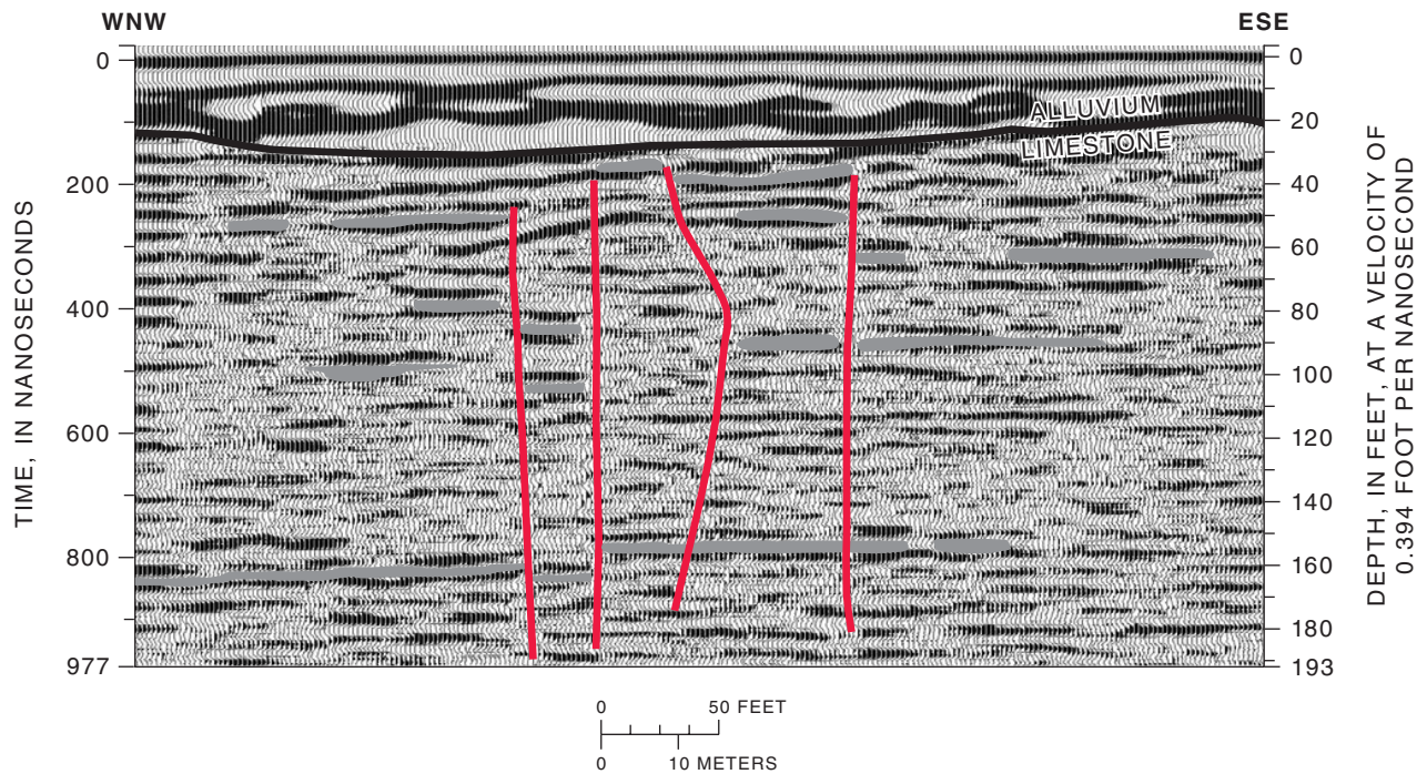
Figure 32. Selected interpreted ground-penetrating radar data for the Continental area. A , Radar profile 2, 0–450. B , Radar profile 3, 0–480 feet. C , Radar profile 9, 0–360 feet. Interpreted fractures are shown in red and interpreted bedding planes are gray fills. Hyperbolic events are interpreted as openings or open horizontal fractures.
