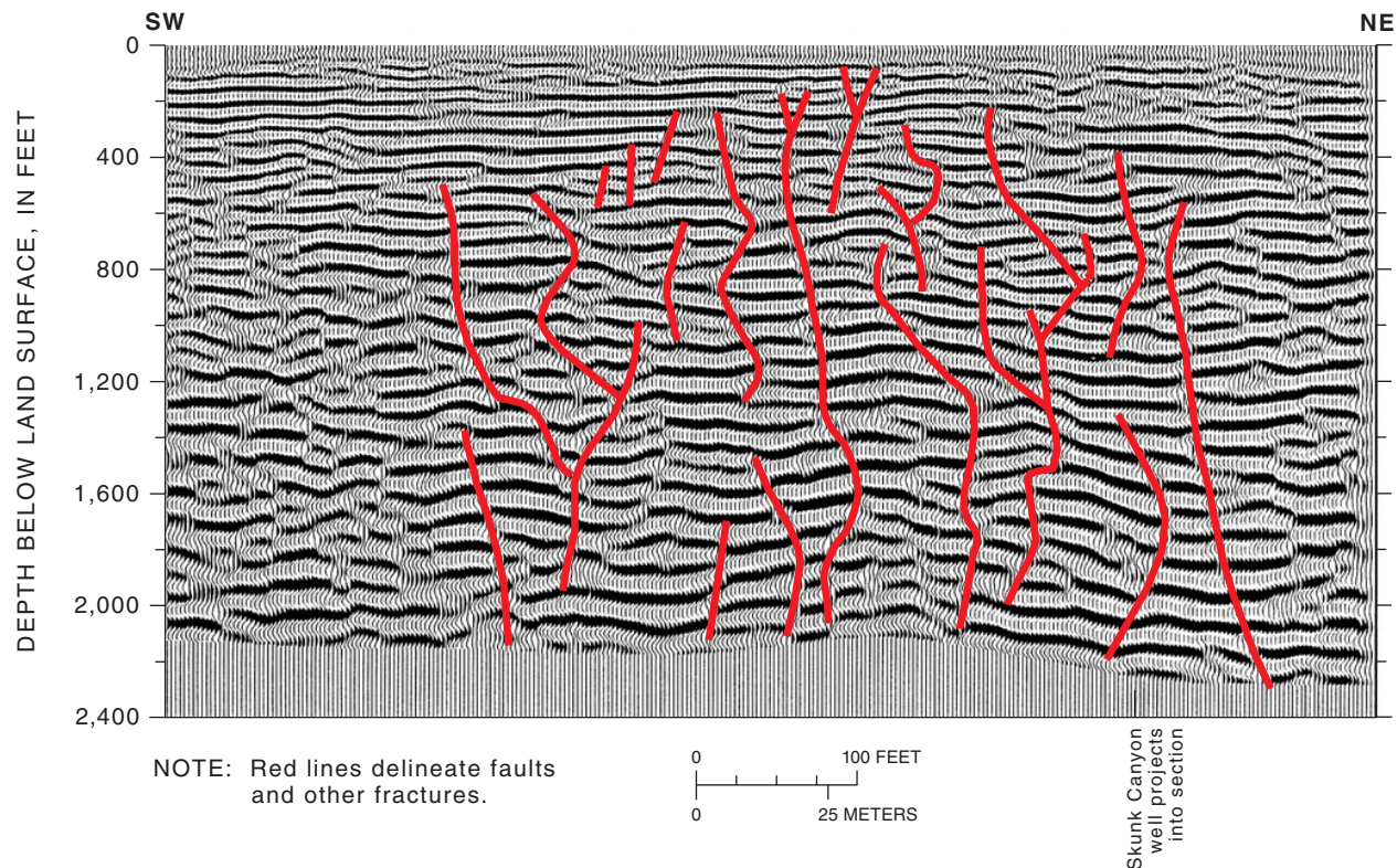
Figure 23. Stacked seismic image of the Skunk Canyon North profile No. 1. Many of the faults in the section are highlighted, but no major, through-going faults are apparent.
