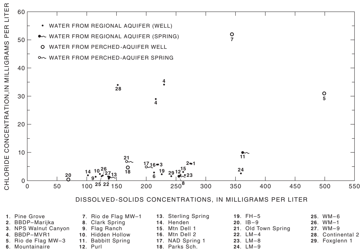
Figure 46. Concentrations of chloride as a function of concentrations of dissolved solids in water from the regional aquifer and perched water-bearing zones, Flagstaff, Arizona, 1995–97.
