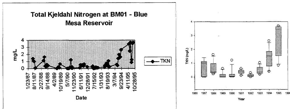
Figure 3. Examples of Graphs and Plots for Water Quality Data
