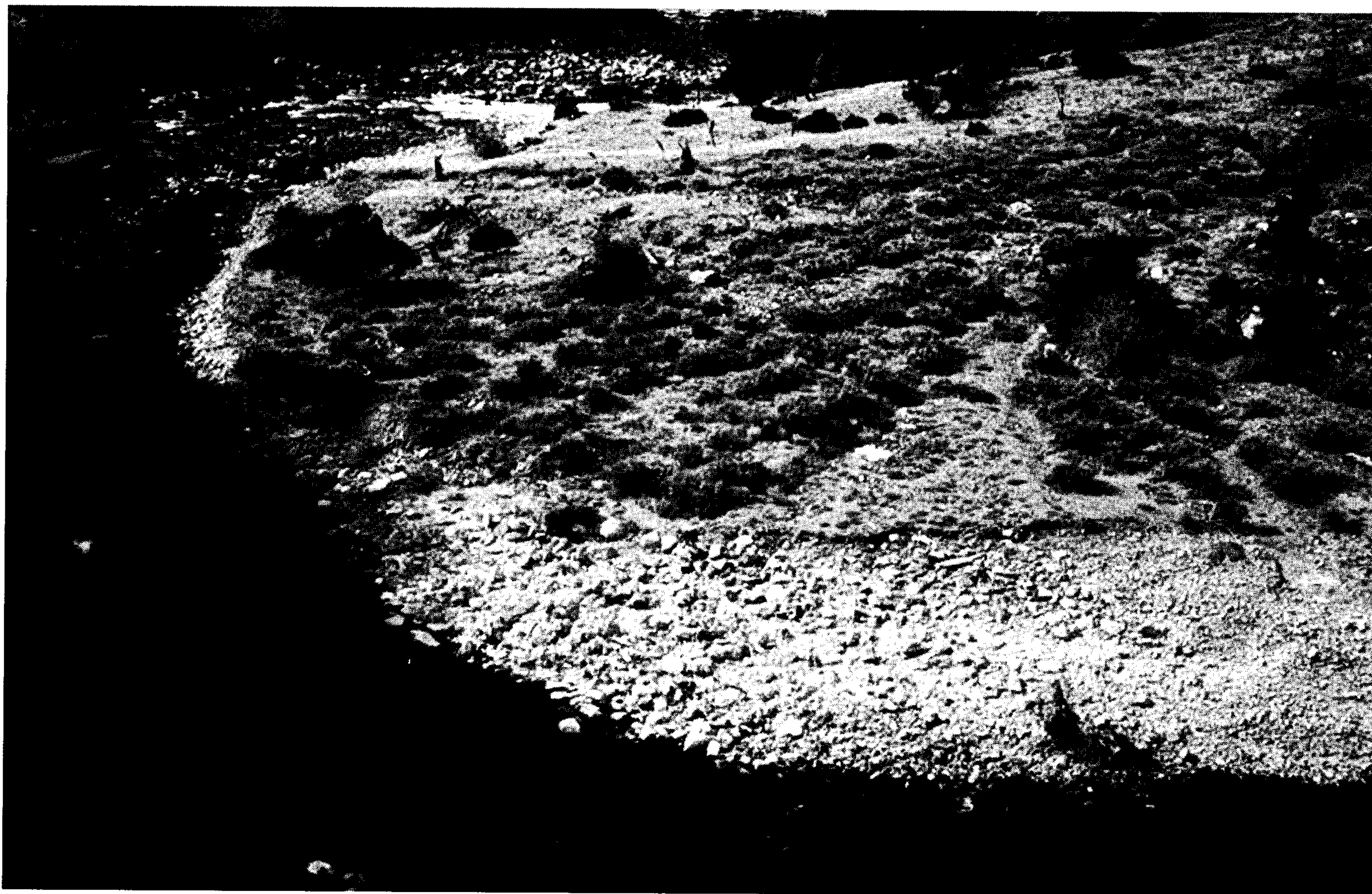
Figure 15. Replicate photographs of the Red Rock Canyon study reach from monument 0005-D, downstream view of debris fan at Tributary 11.3R: (A) August 6, 1994, 400 cubic feet per second, (B) September 26, 1995, 600 cubic feet per second—Continued.
