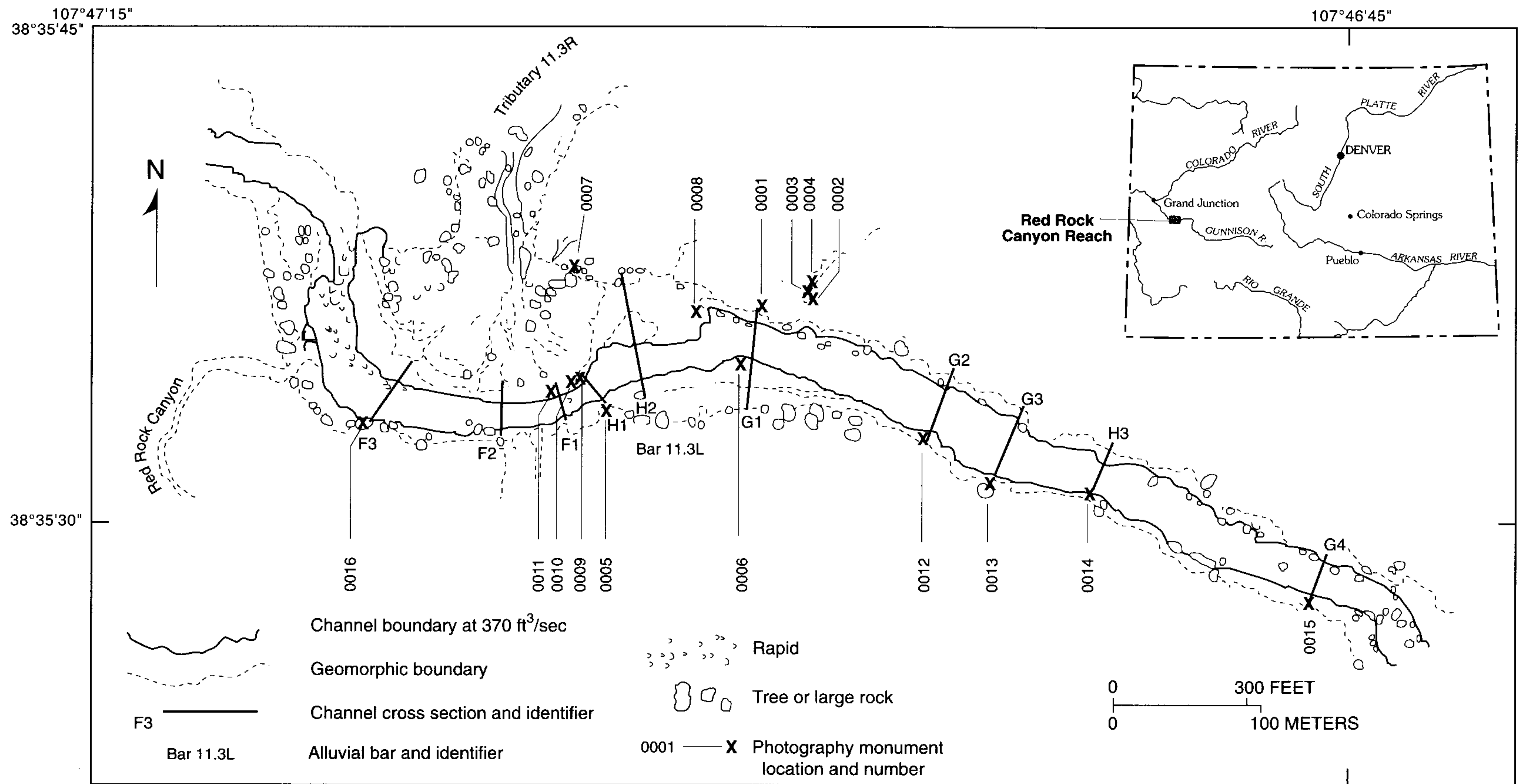
Figure 5. Map of the Red Rock Canyon study reach showing location of surveyed cross sections and oblique-photography monuments. Channel boundary at 370 cubic feet per second determined from July 3, 1989, aerial photograph.
