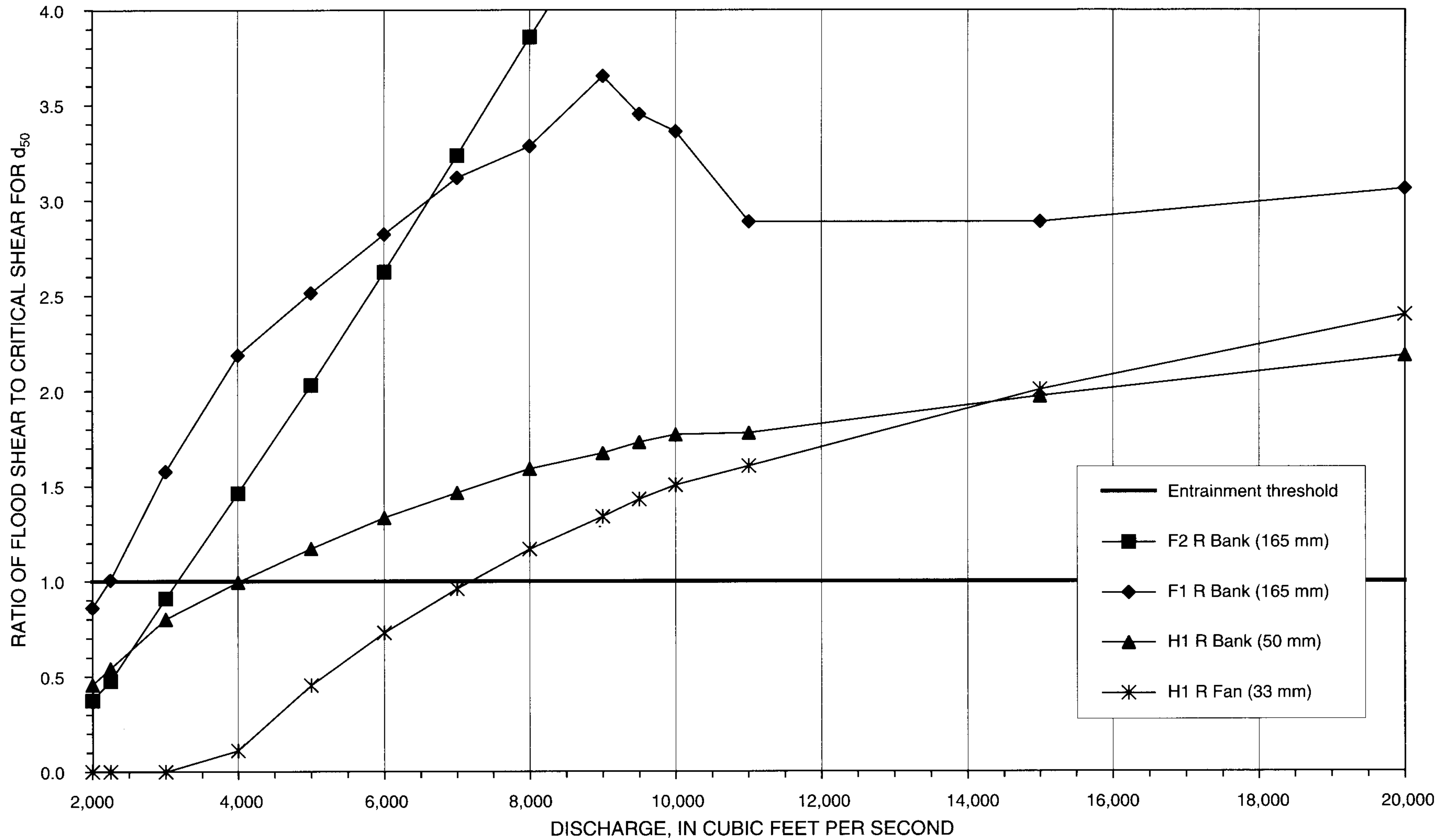
Figure 9. Plot showing sediment-entrainment potential on distal debris-fan surfaces in the Red Rock Canyon study reach. Median particle size of the surface is shown in parentheses.
