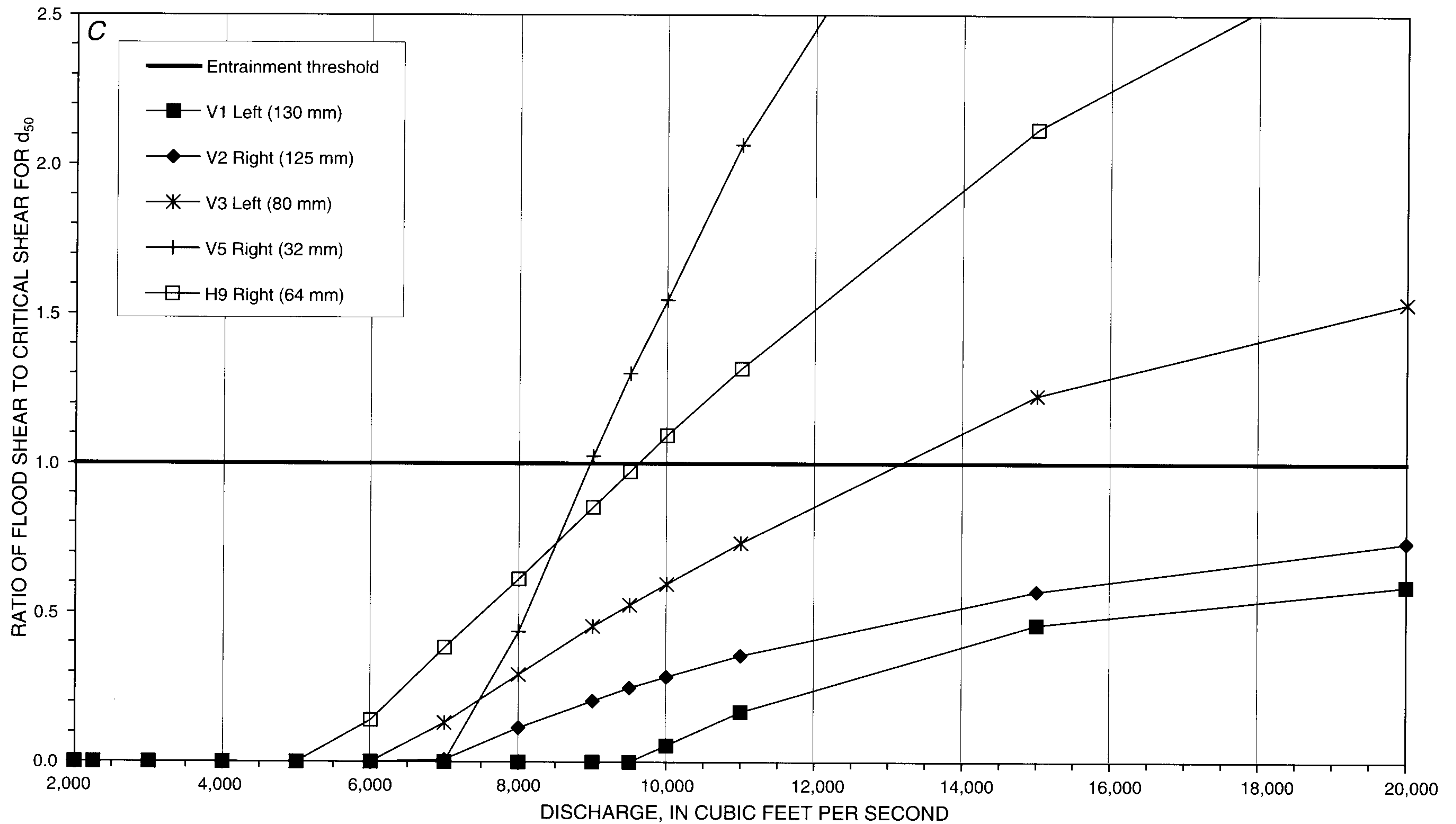
Figure 8. Plots showing sediment-entrainment potential on similar geomorphic surfaces in the Warner Point study reach: (A) low-flow banks, (B) low-bar surfaces, (C) high-bar surfaces, and (D) overflow channels. Median particle size of the surface is shown in parentheses—Continued.
