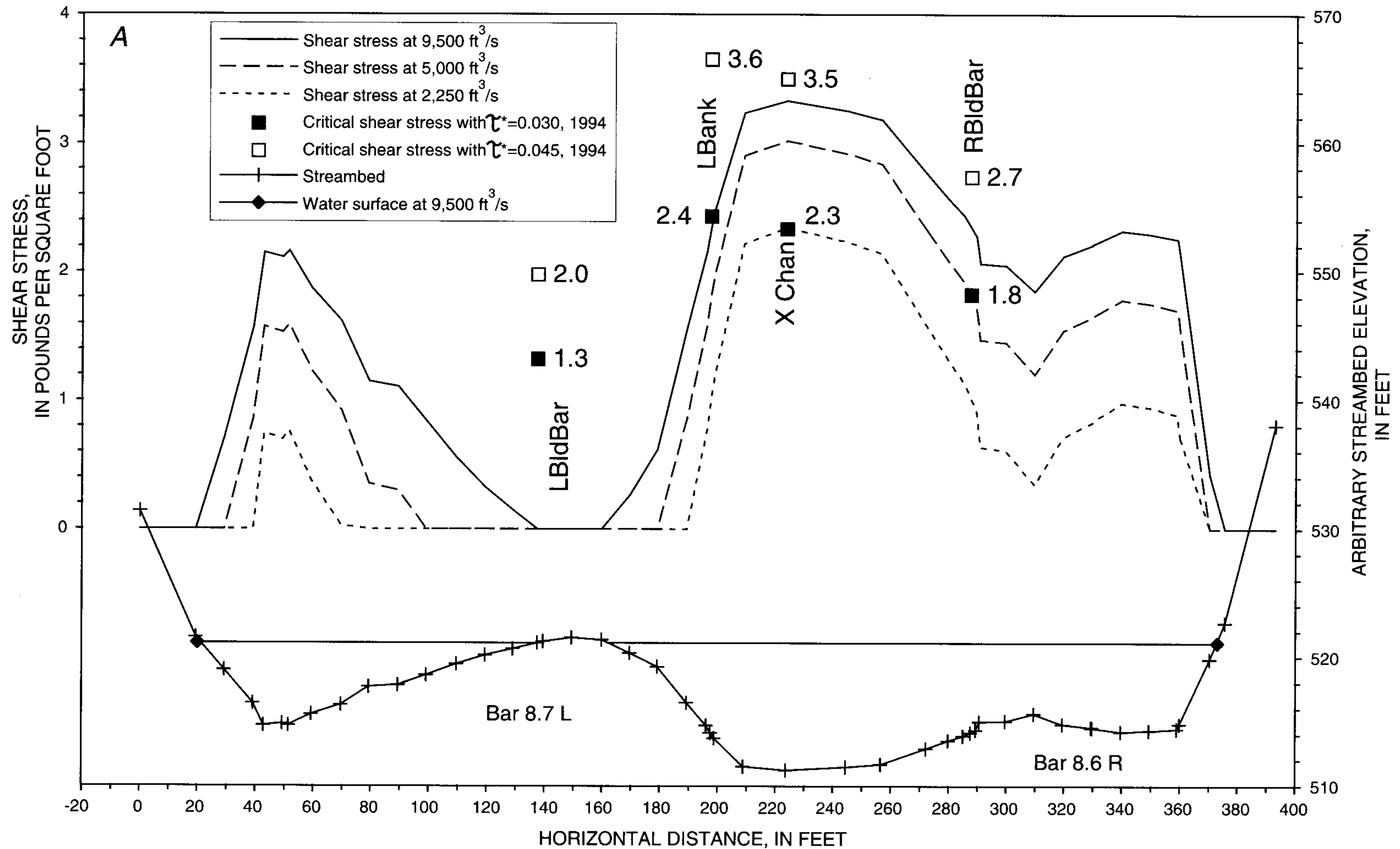
Figure 6. Plots showing channel cross section, shear-stress distribution, and critical shear stress for sediment median particle size in the Warner Point study reach: (A) cross section V1, (B) cross section V2, (C) cross section H60, (D) cross section H3, (E) cross section V3, (F) cross section V4, (G) cross section V5, and (H) cross section H9 (study reach shown in fig. 4).
