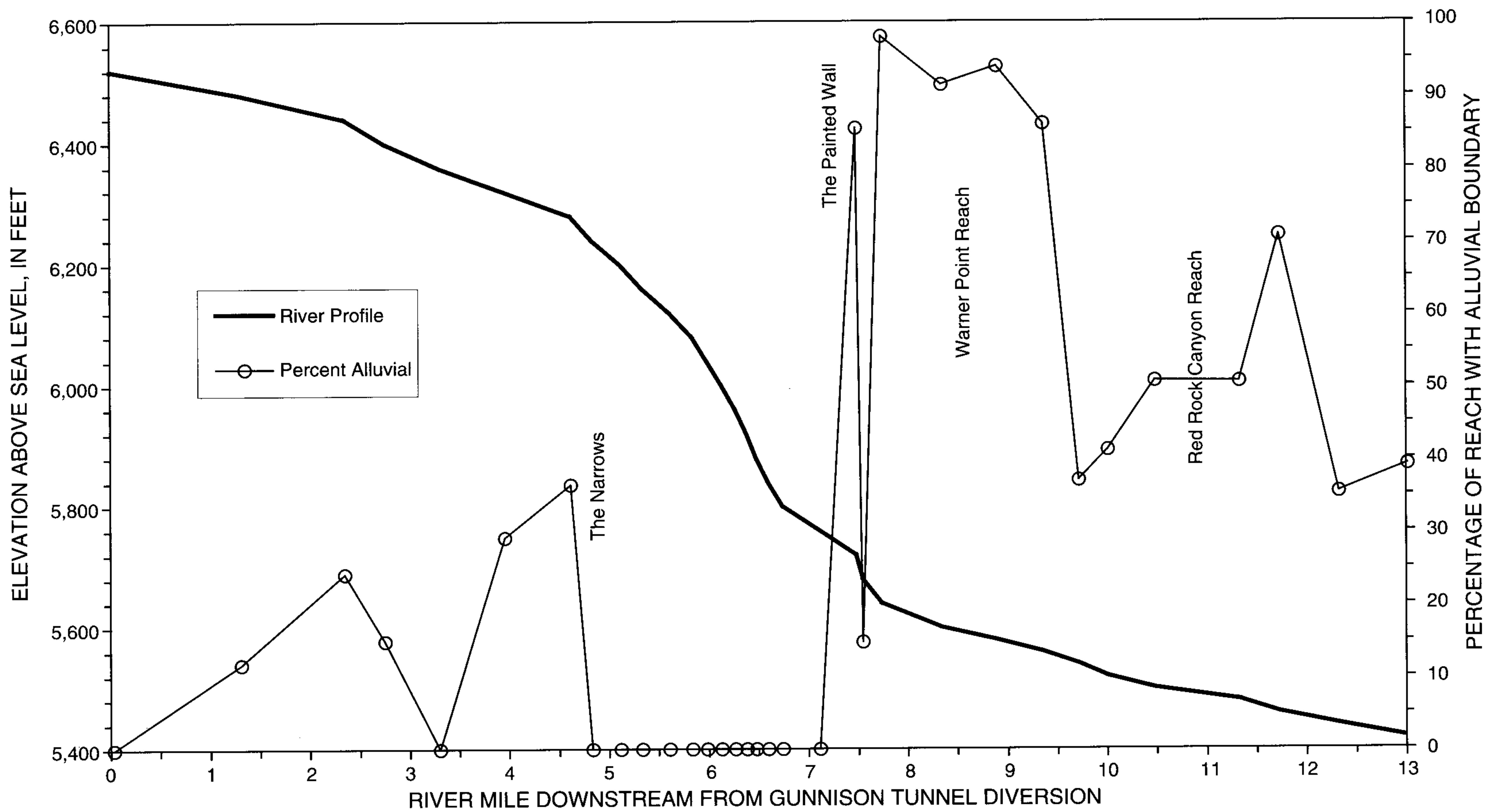
Figure 3. Gunnison River profile and the location and relative abundance of alluvial deposits in Black Canyon of the Gunnison National Monument.
