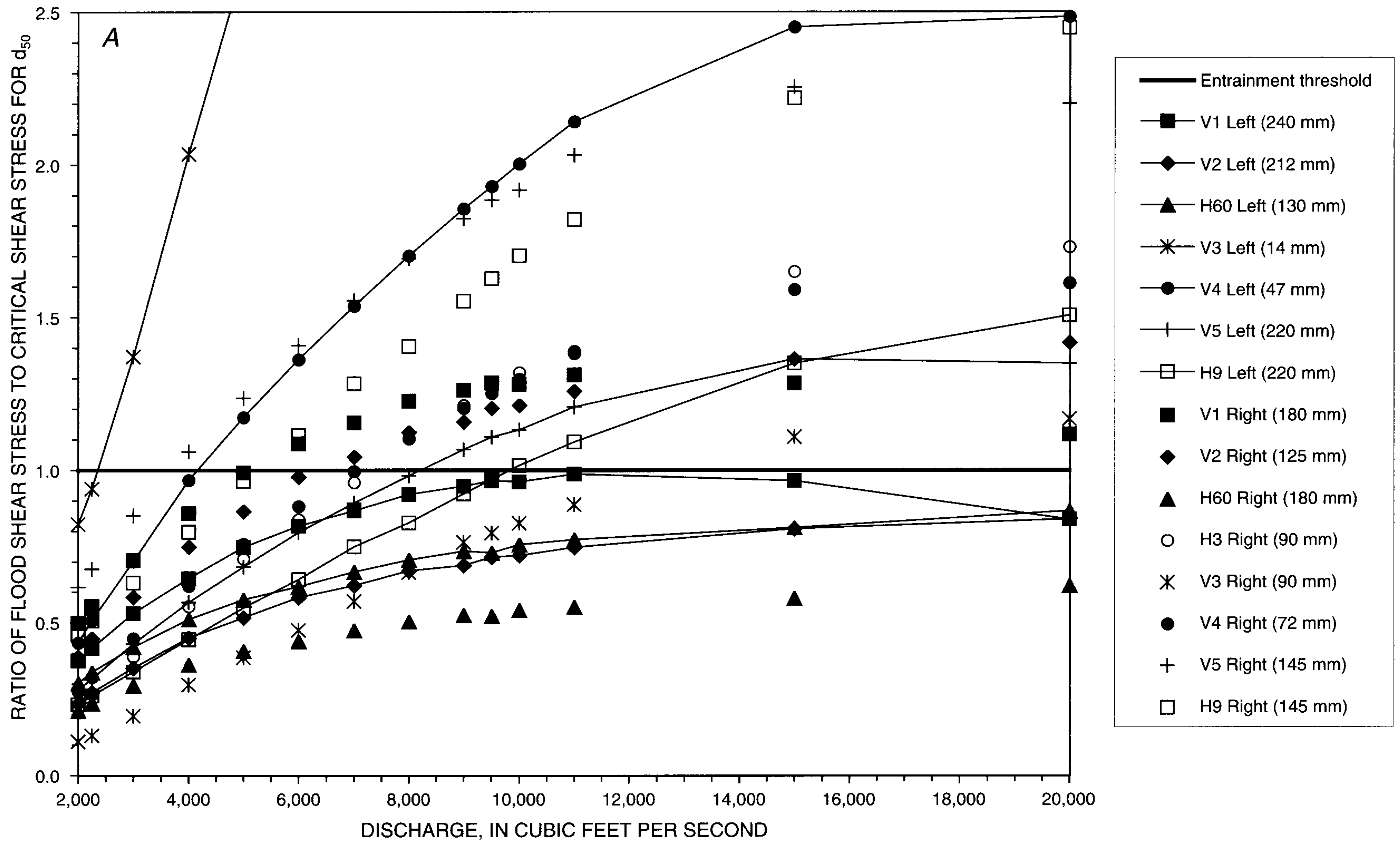
Figure 8. Plots showing sediment-entrainment potential on similar geomorphic surfaces in the Warner Point study reach: (A) low-flow banks, (B) low-bar surfaces, (C) high-bar surfaces, and (D) overflow channels. Median particle size of the surface is shown in parentheses.
