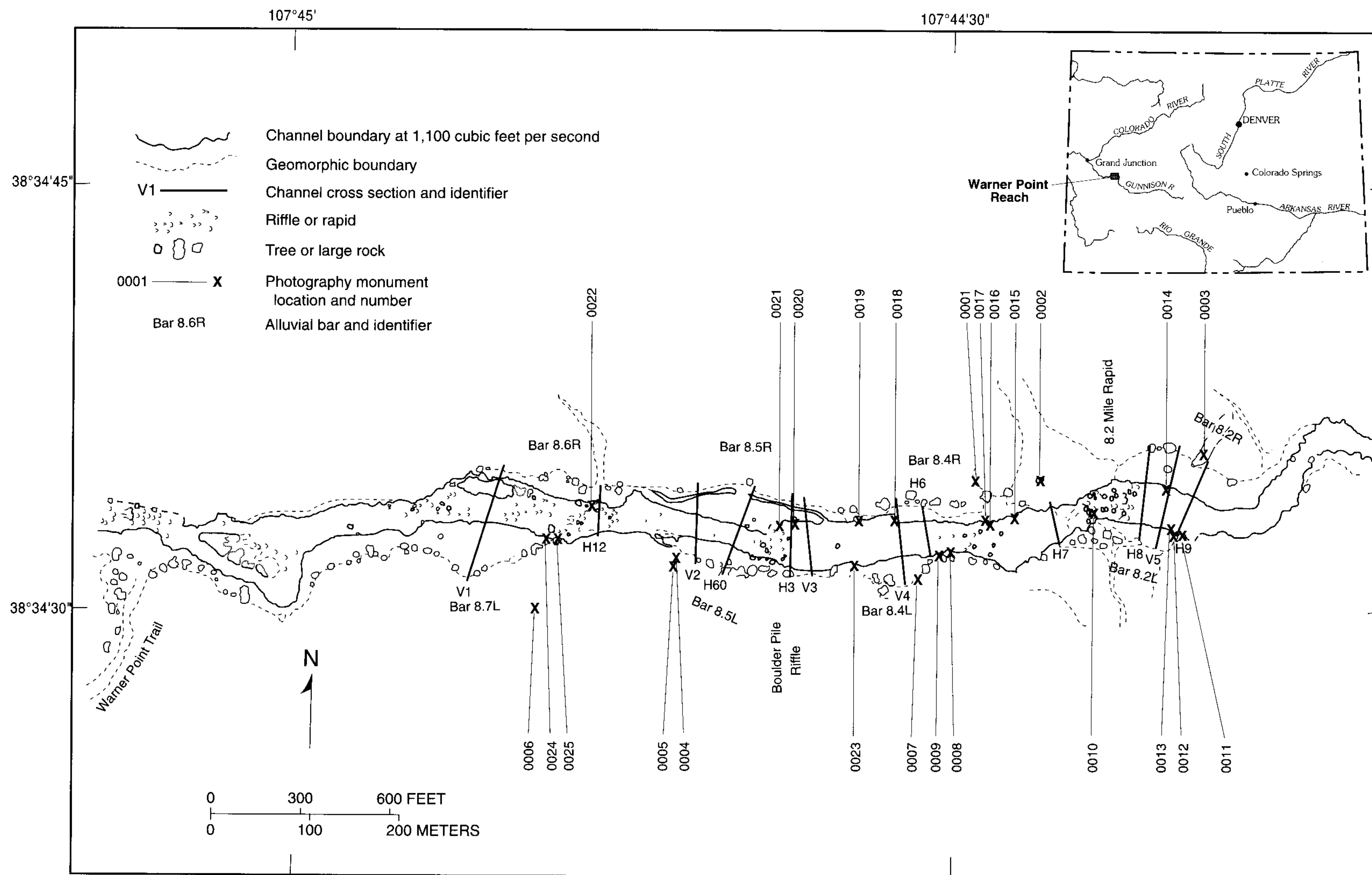
Figure 4. Map of the Warner Point study reach showing location of surveyed cross sections and oblique-photography monuments. Channel boundary at 1,100 cubic feet per second determined from June 27, 1982, aerial photograph.
