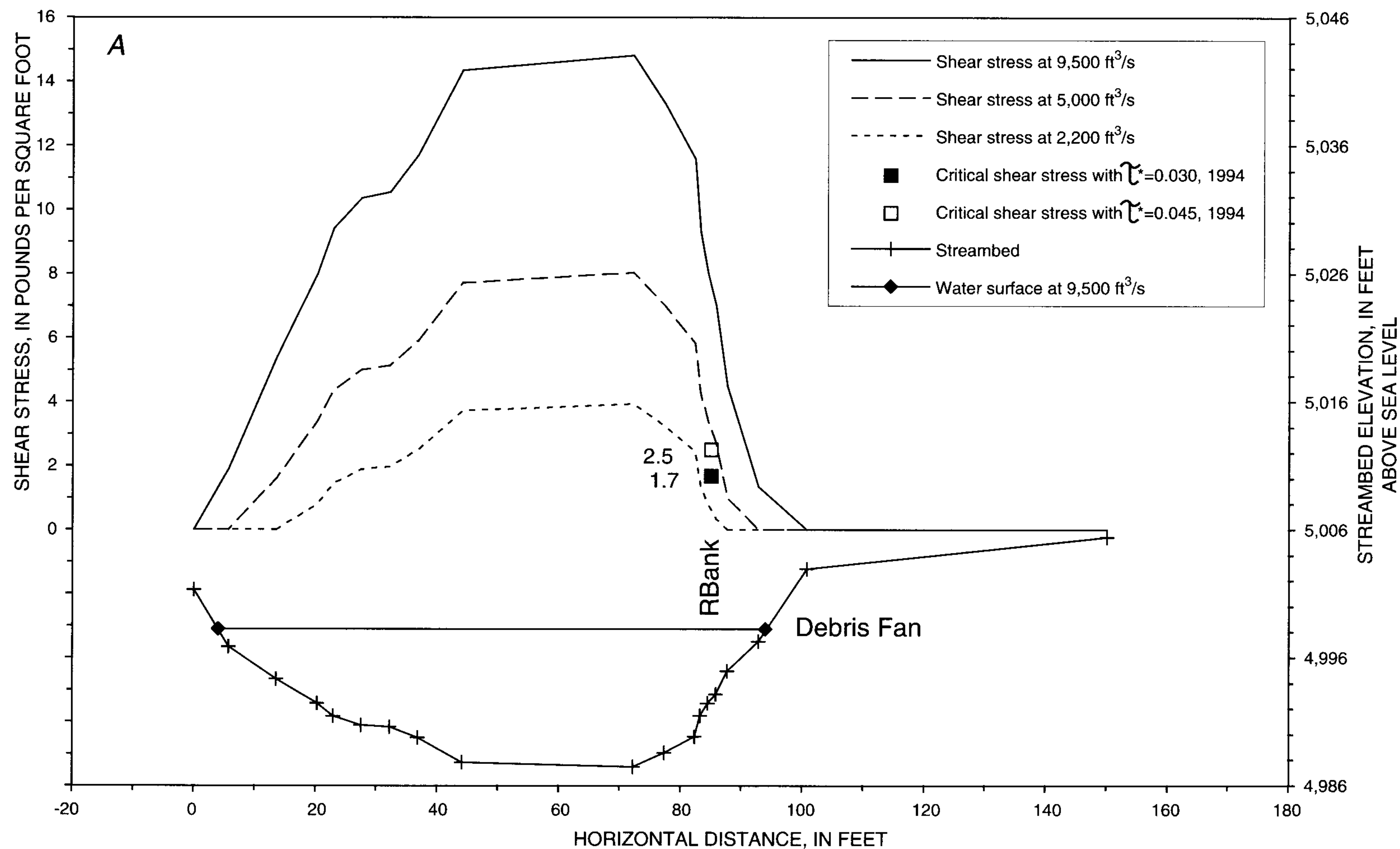
Figure 7. Plots showing channel cross section, shear-stress distribution, and critical shear stress for sediment median particle size in the Red Rock Canyon study reach, (A) cross section F2, (B) cross section F1, (C) cross section H1, (D) cross section H2, (E) cross section G1, and (F) cross section G2. (study reach shown in fig. 5).
