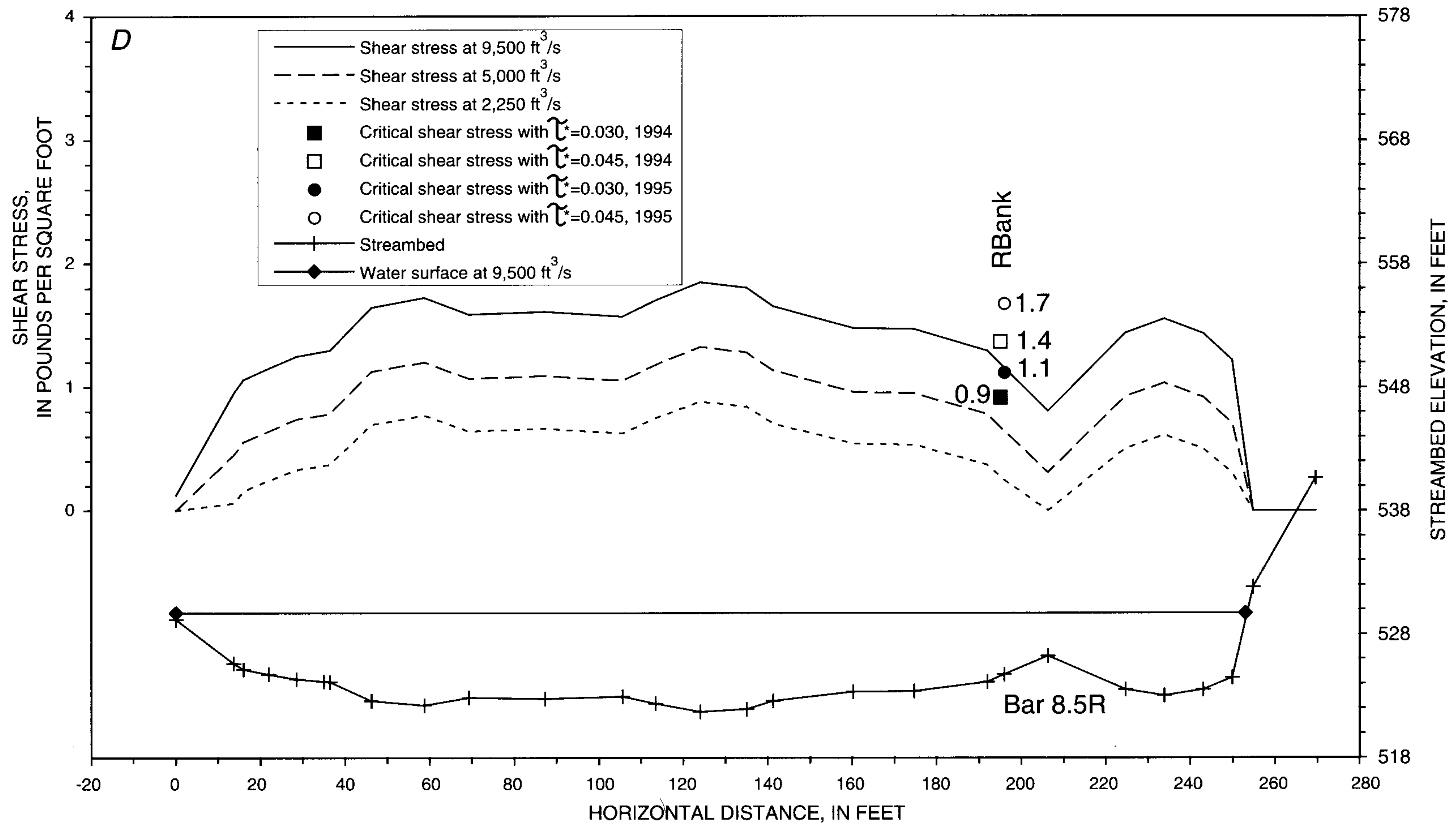
Figure 6. Plots showing channel cross section, shear-stress distribution, and critical shear stress for sediment median particle size in the Warner Point study reach: (A) cross section V1, (B) cross section V2, (C) cross section H60, (D) cross section H3, (E) cross section V3, (F) cross section V4, (G) cross section V5, and (H) cross section H9 (study reach shown in fig. 4)—Continued.
