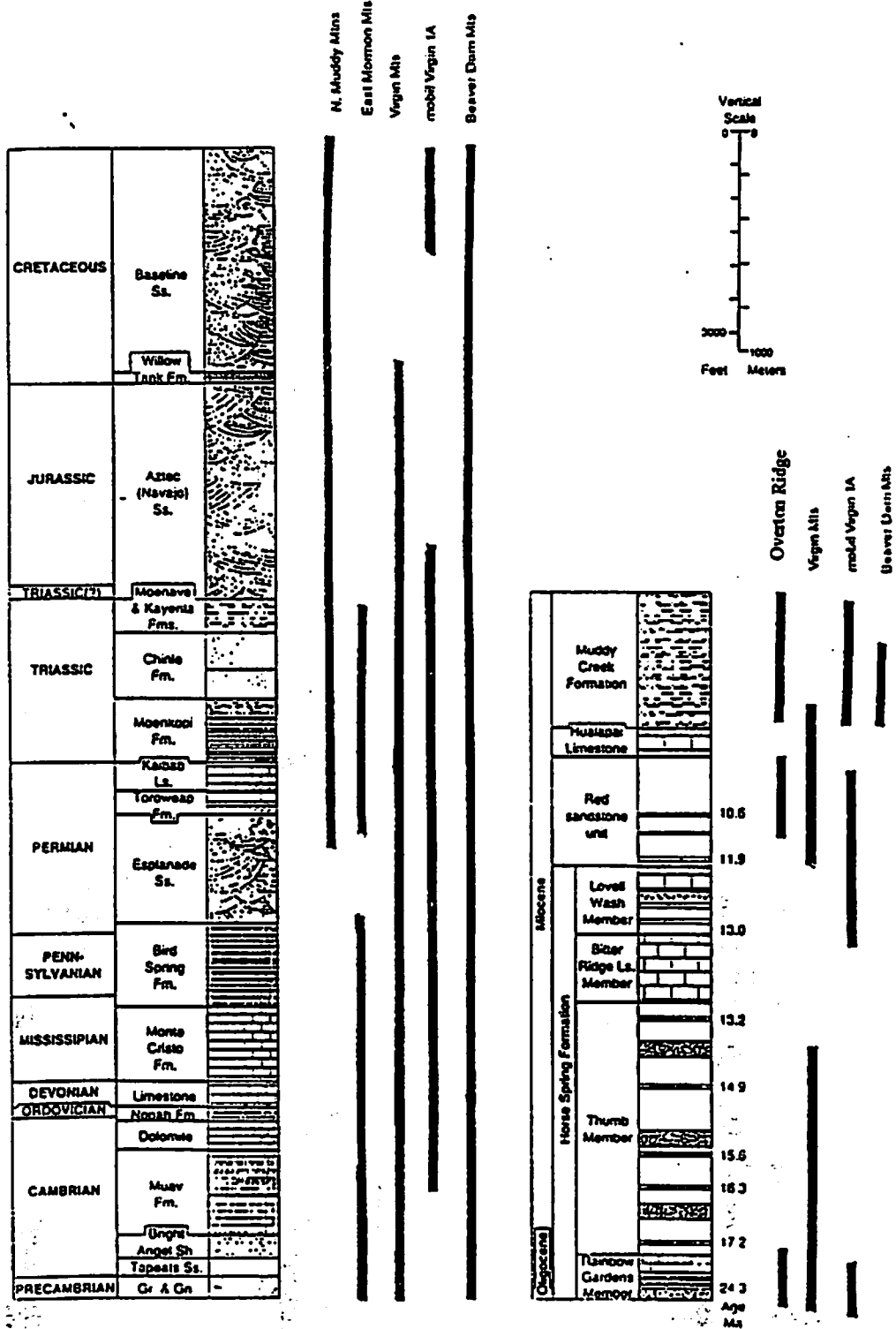
Figure 6: Generalized Stratigraphy of the Lower Virgin River Basin (from Metcalf, 1995).
