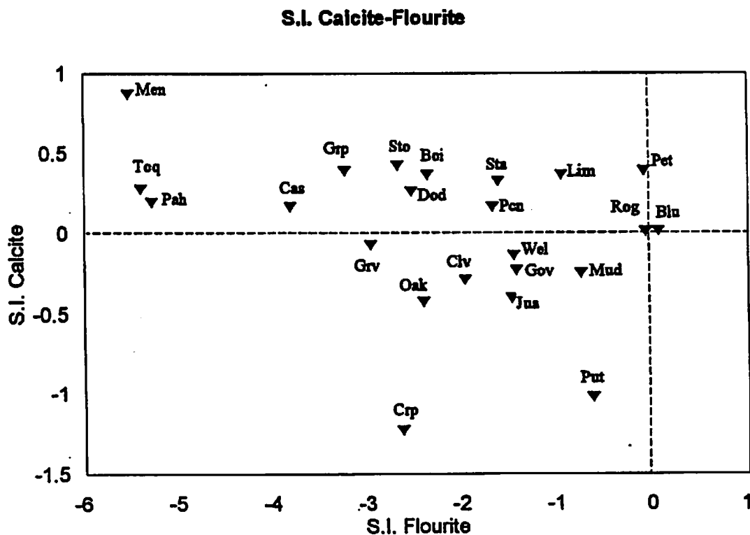
Figure 27: Virgin River Basin Spring Water Mineral Equilibrium Plot: calcite vs. fluorite
