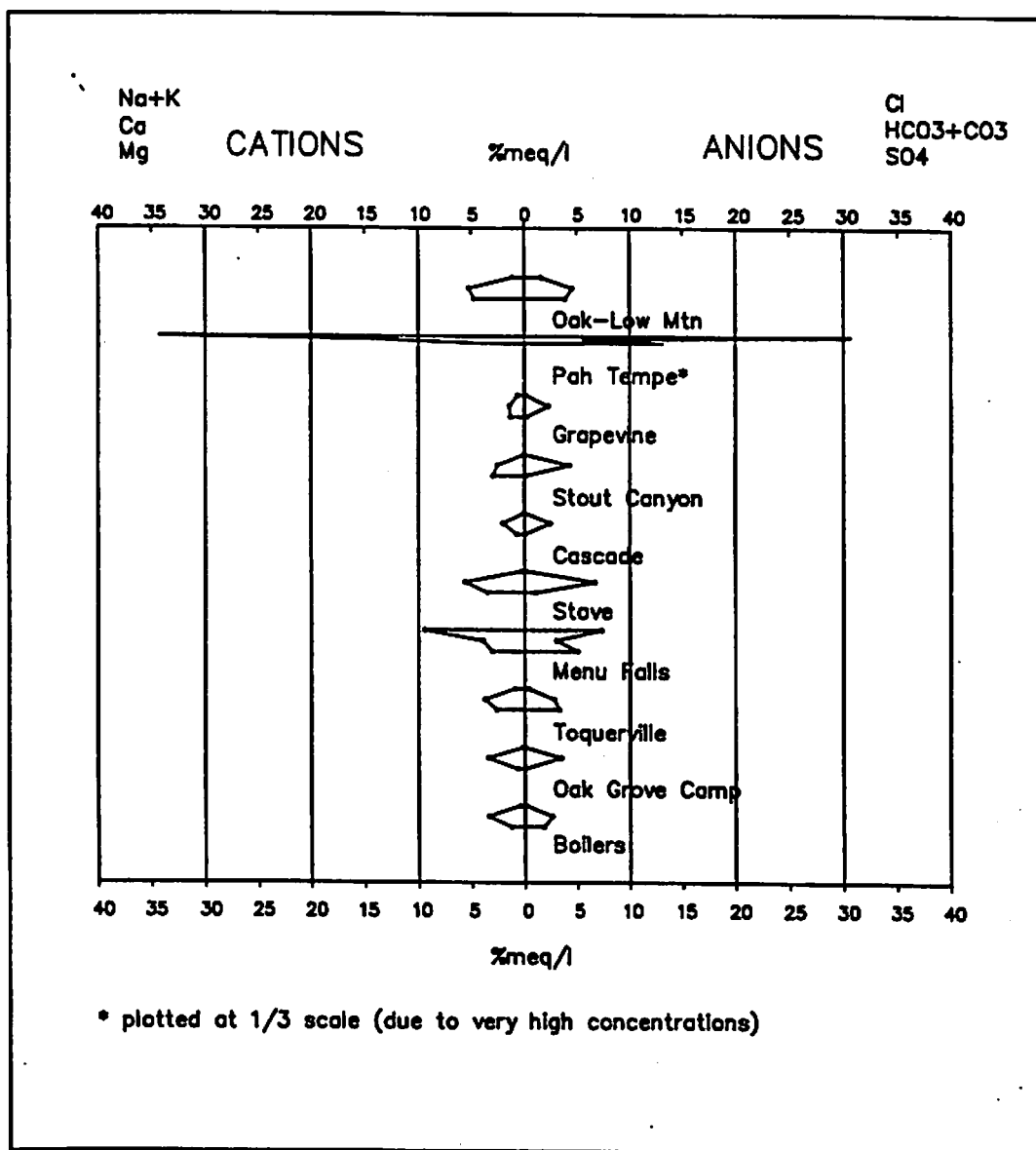
Figure 11: Stiff Diagram: Upper and Central Virgin River Basin Spring Waters
