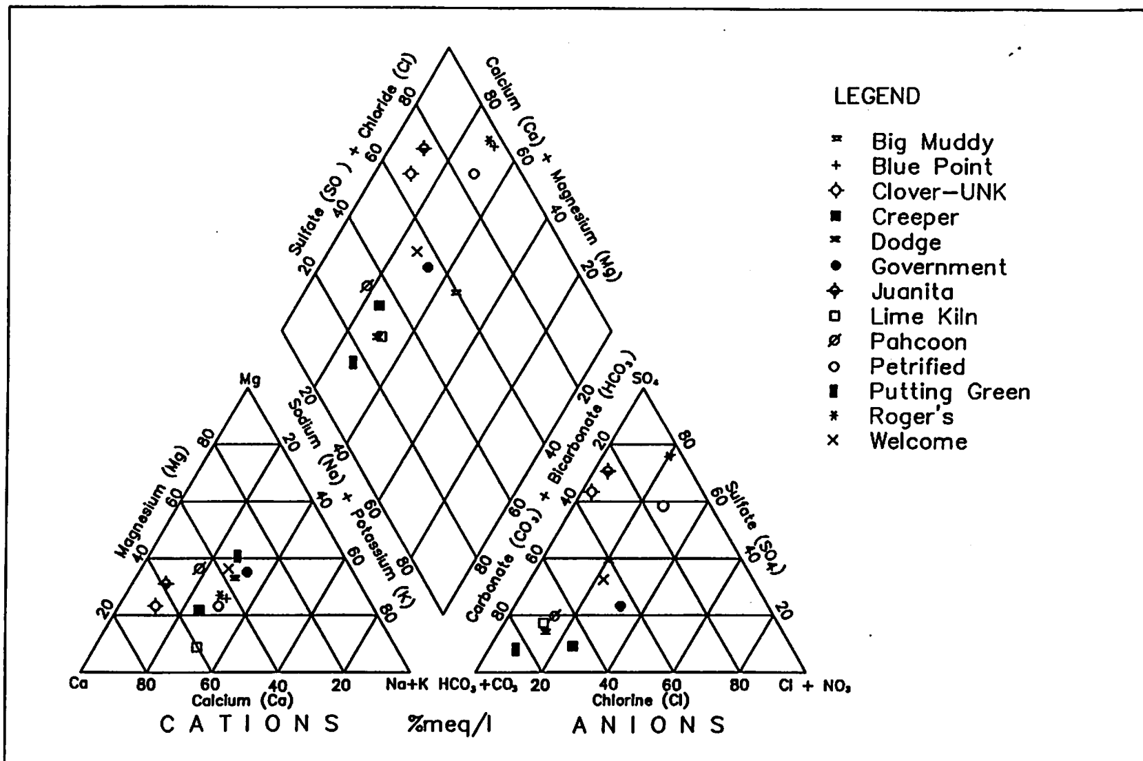
Figure 8: Piper Diagram: Lower Virgin River Basin Spring Waters
