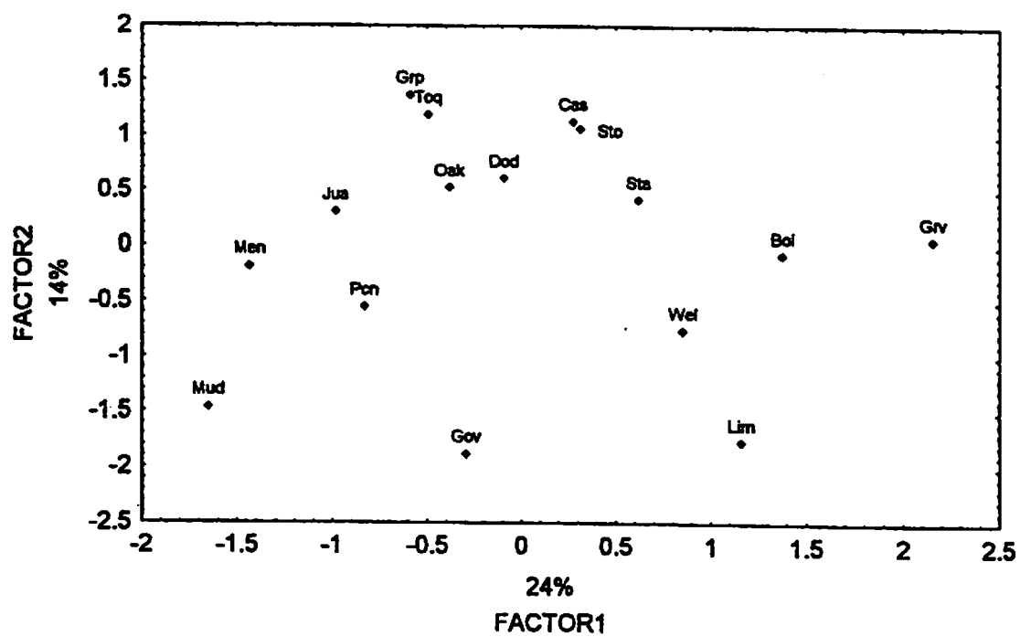
Figure 17: All Chemical Concentrations, without Previous Groupings
