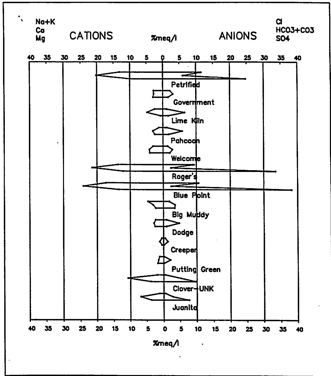
Figure 10: Stiff Diagram: Lower Virgin River Basin Spring Waters
