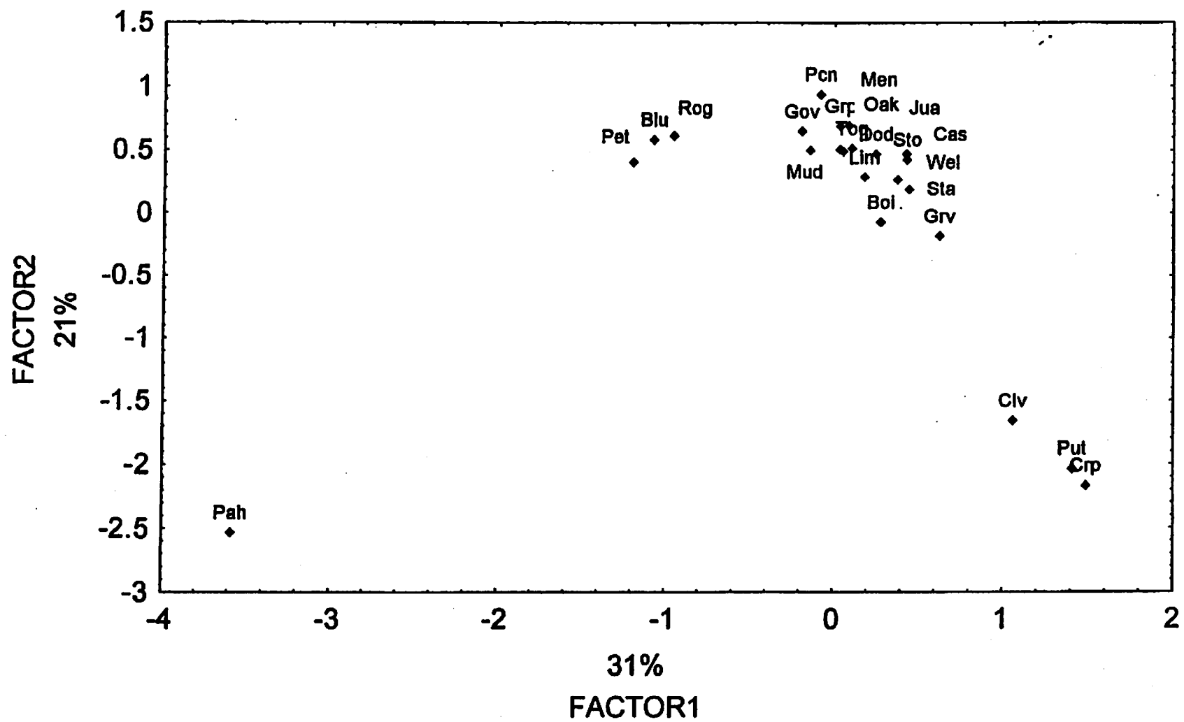
Figure 15: All Trace Elements, All Springs
