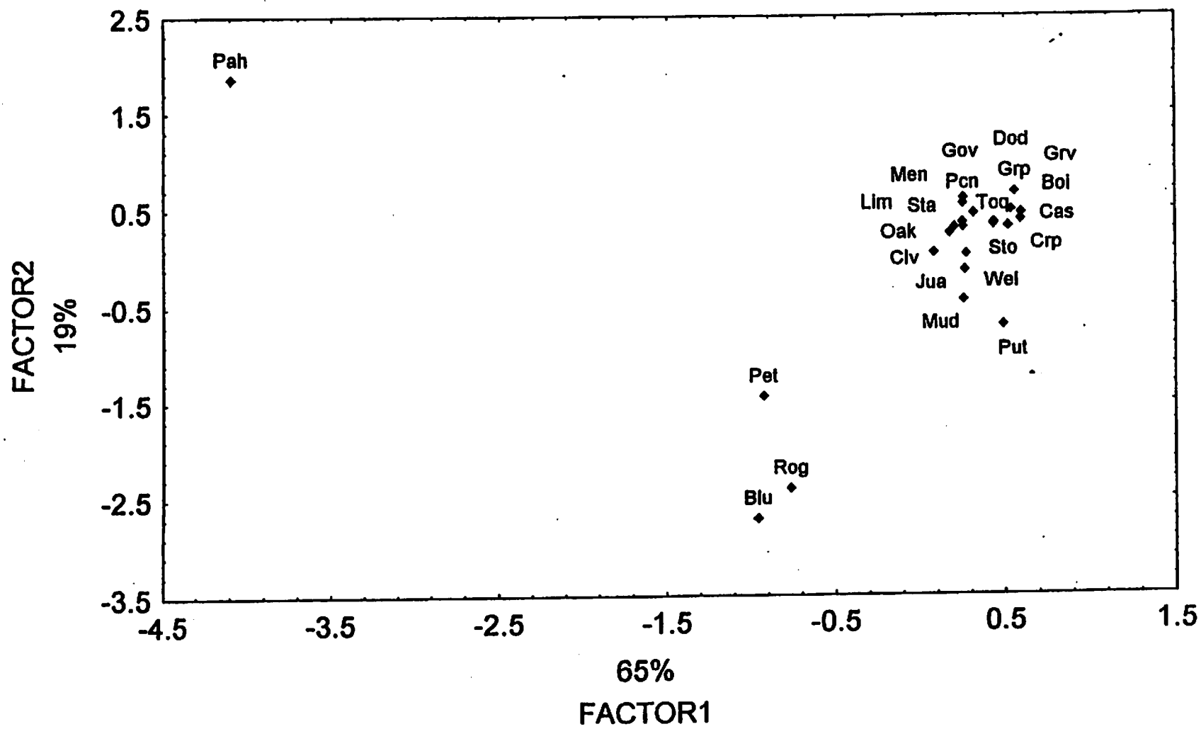
Figure 20: Major Ions, All Springs
