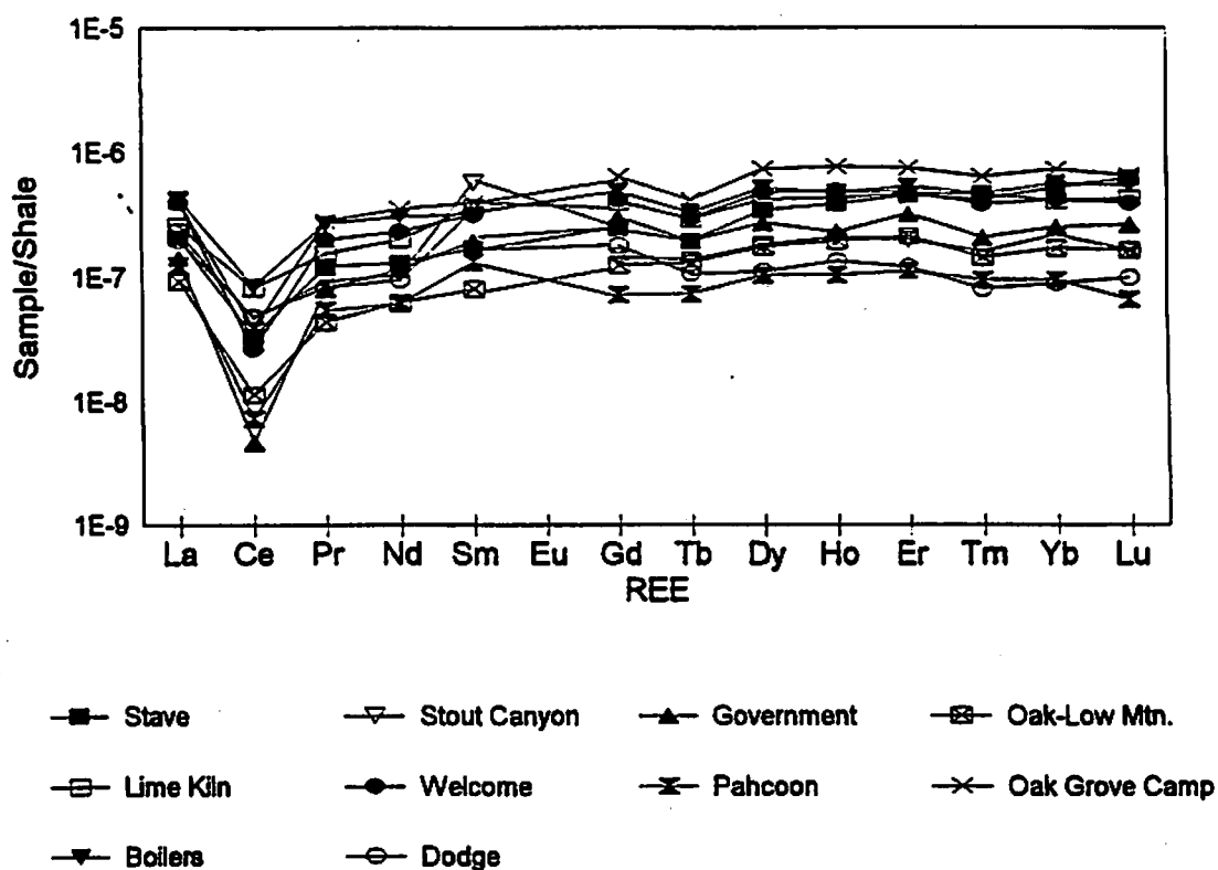
Figure 22: REE Normalization Plot Typical of Spring in the Virgin River Basin
