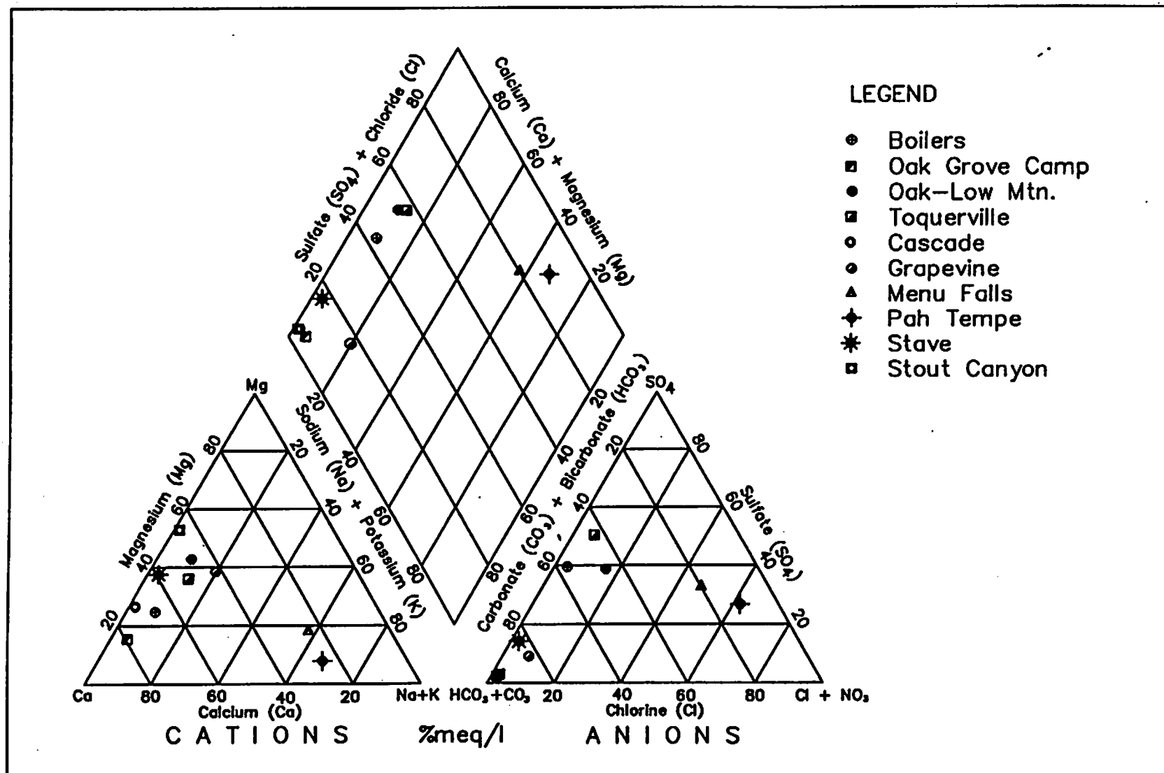
Figure 9: Piper Diagram: Upper and Central Virgin River Basin Spring Waters
