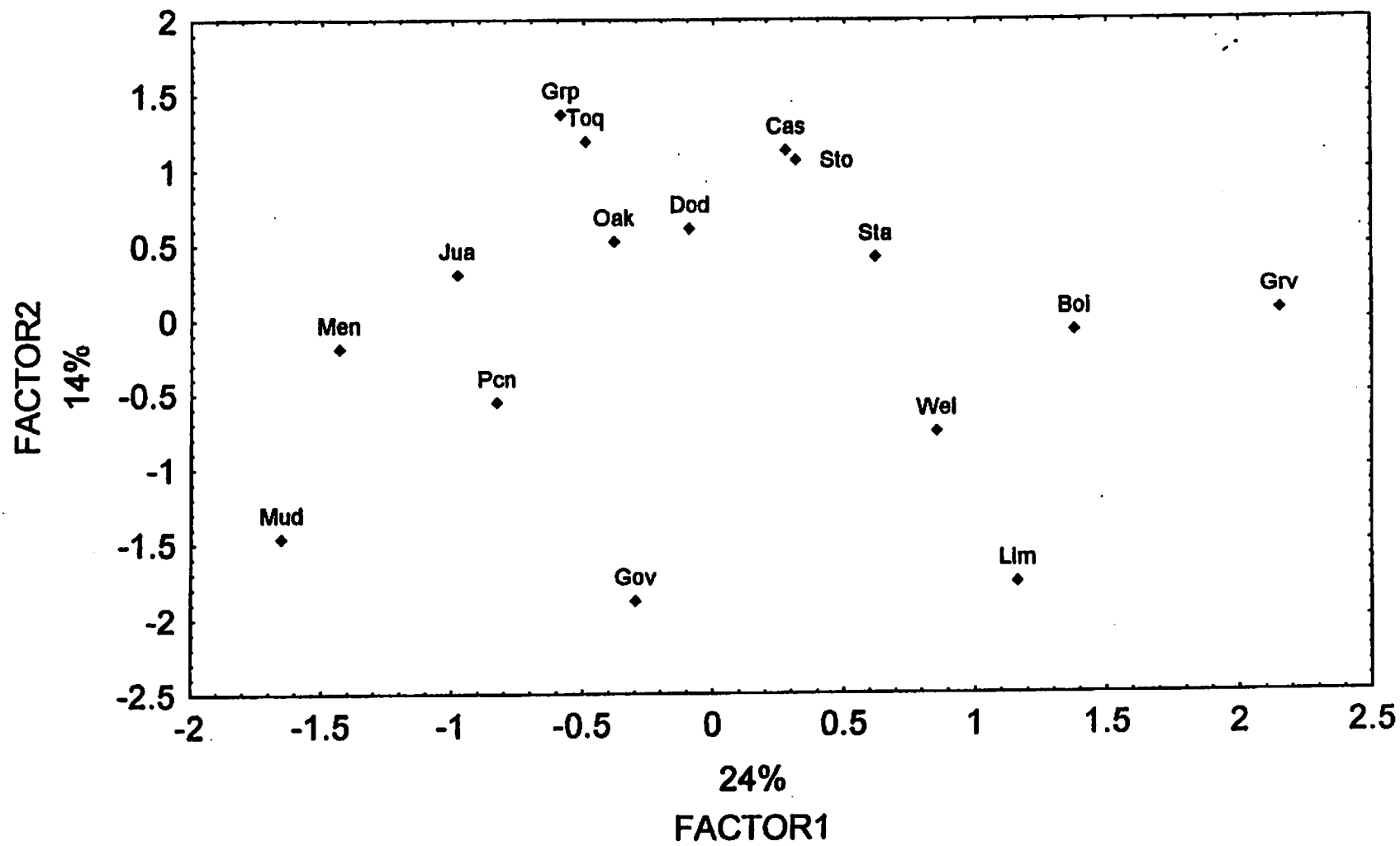
Figure 17: All Chemical Concentrations, without Previous Groupings
