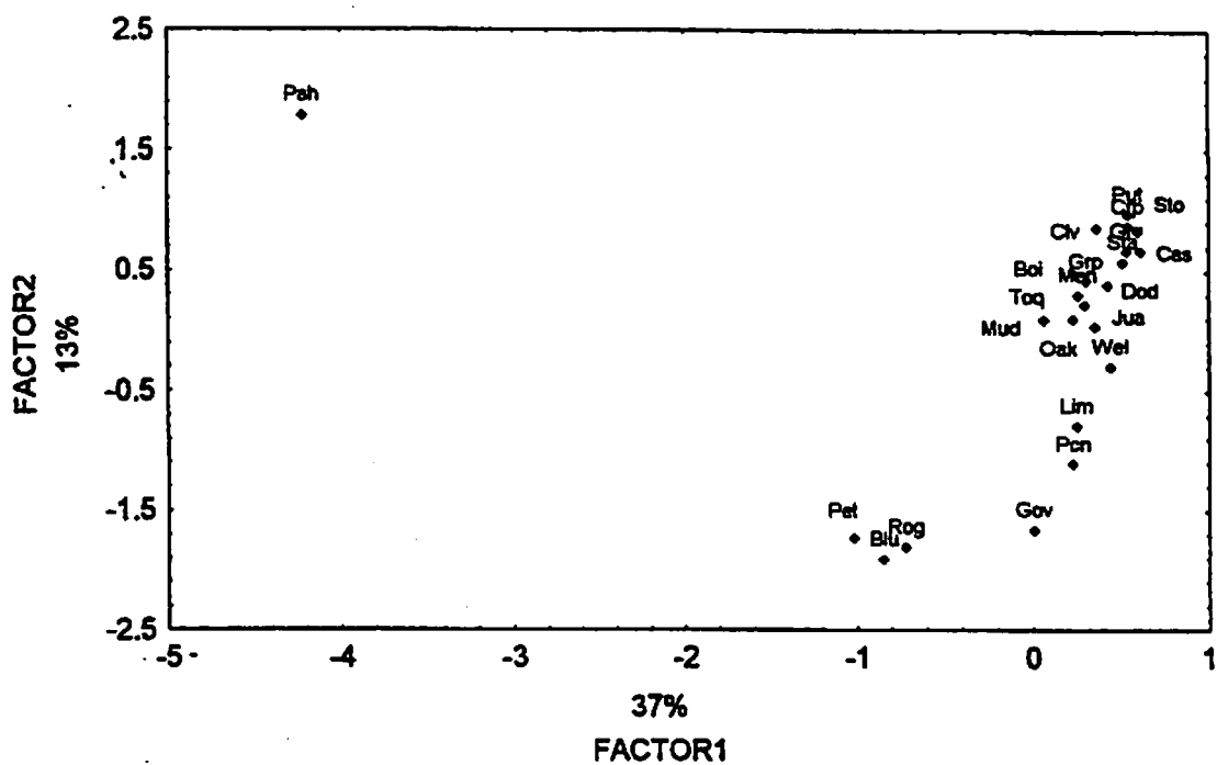
Figure 16: Trace Elements without REE Concentrations
