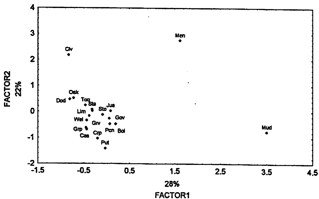
Figure 21: Selected Trace Elements without Pah Tempe, Petrified, Roger's, and Blue Point Springs
