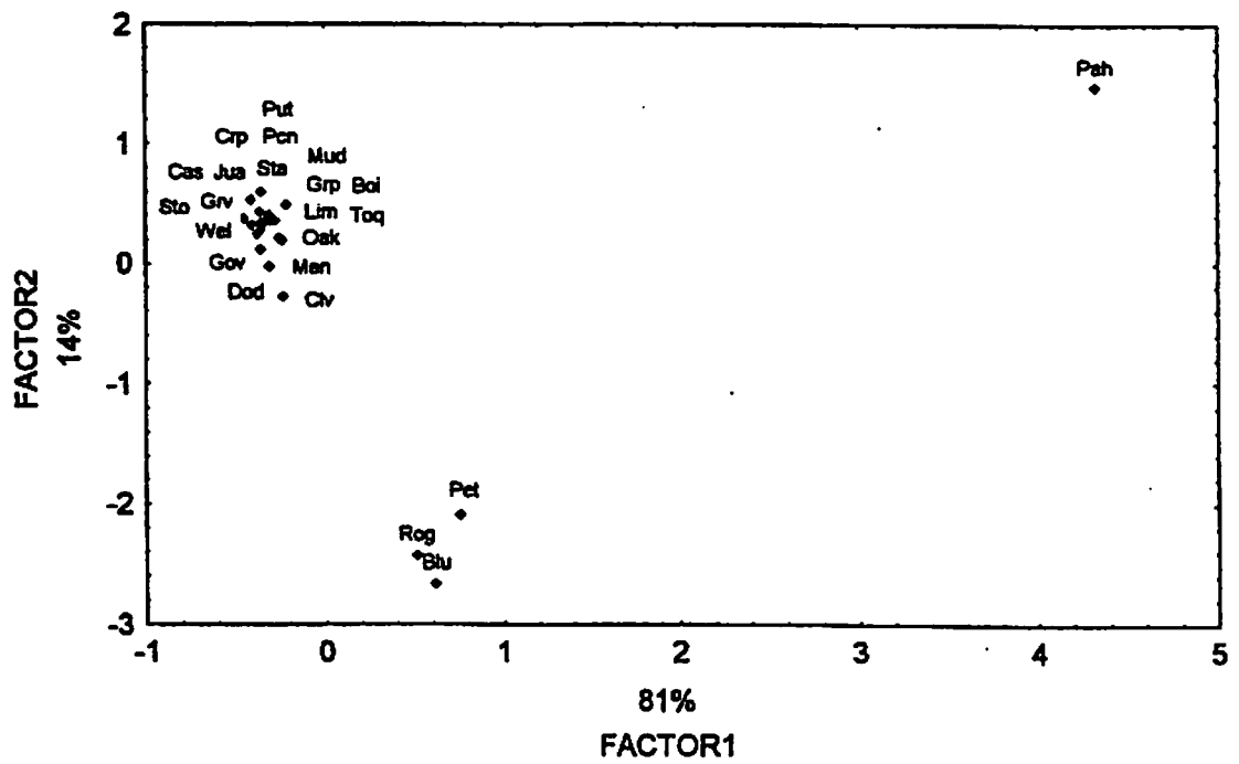
Figure 19: Selected Trace Elements, All Springs
