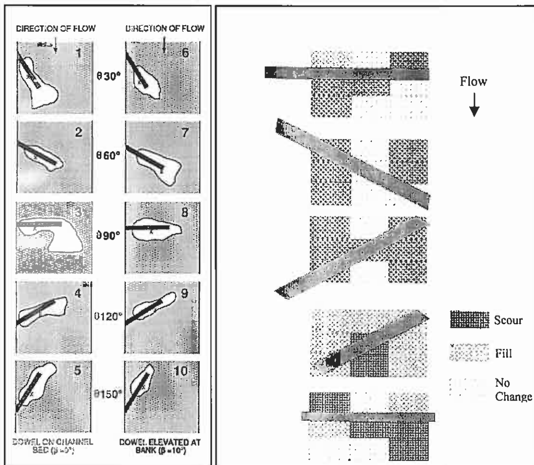
Figure 24. Diagrams showing possible orientations of LWD with associated scour patterns (from Hildebrand et al., 1997; Cherry and Beschta, 1989, and Hildebrand et al., 1998 respectively).
