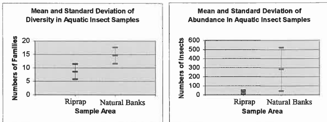
Figure 23. Plots of means and standard deviations for aquatic insect diversity and abundance in samples from riprap and natural bank areas. Note that means of non-riprap samples are higher than riprap samples, however there is some overlap with the standard deviations.
