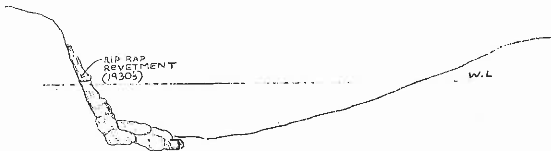
Figure 13. Cross section diagram of CCC rock revetment construction showing the bank protected along the toe and into the channel bed (From Howell and Milestone, 1981).
