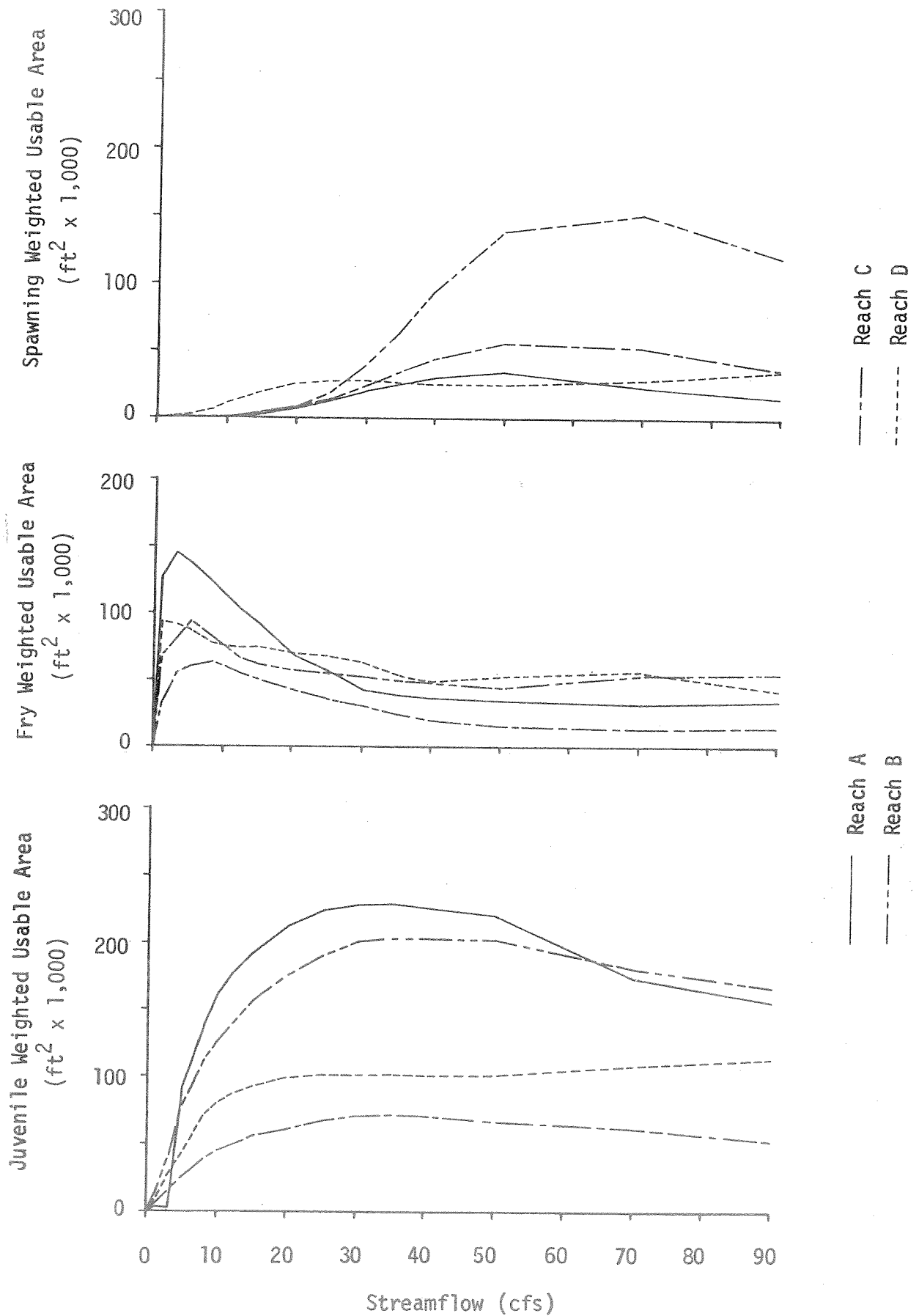
FIGURE 7. Steelhead trout habitat/streamflow relationship, Lagunitas Creek.
