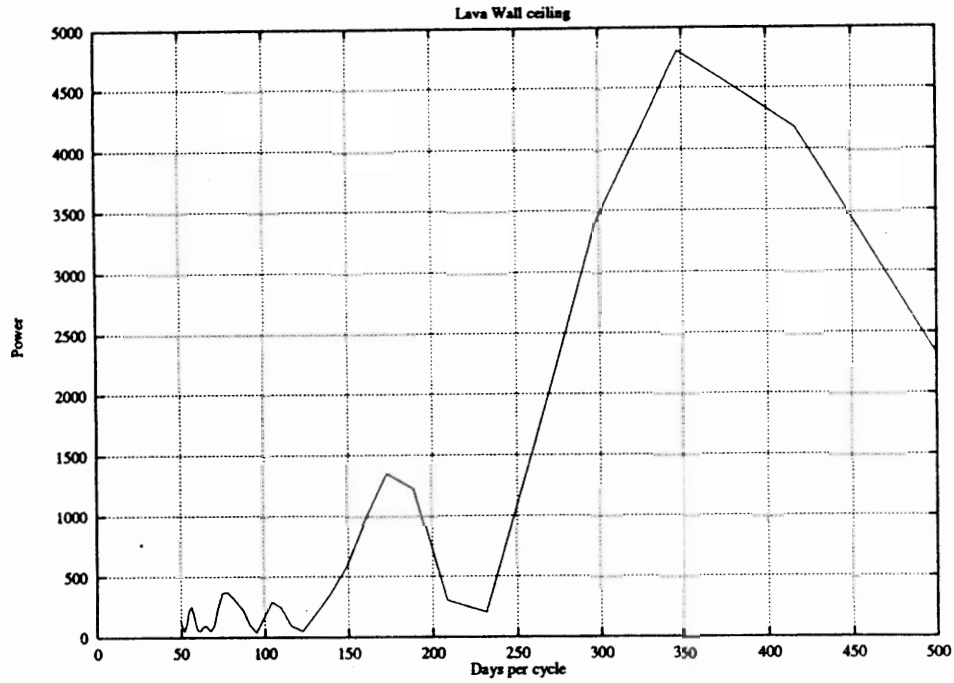
Figure 4.39: Power spectrum for cycles longer than one day for the Lava Wall ceiling temperature.
