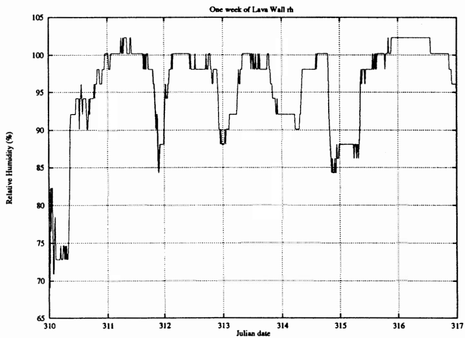
Figure 4.24: One week of relative humidity in Lava Wall.
