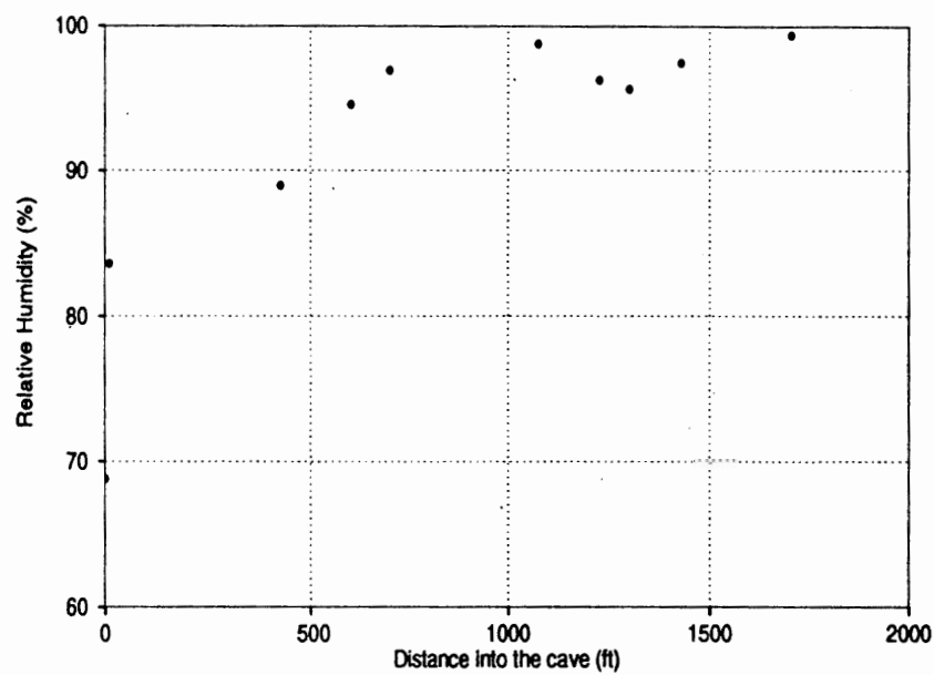
Figure 4.45: Distance vs Humidity in Braided Cave, El Malpais National Monument on August 16, 1995.
