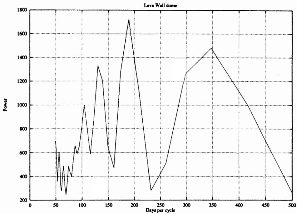
Figure 4.41: Power spectrum for cycles longer than one day for the Lava Wall dome temperature.
