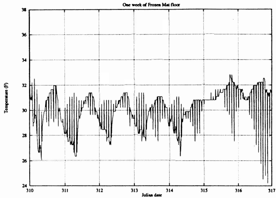
Figure 4.16: One week of temperatures for the floor in Frozen Mat.
