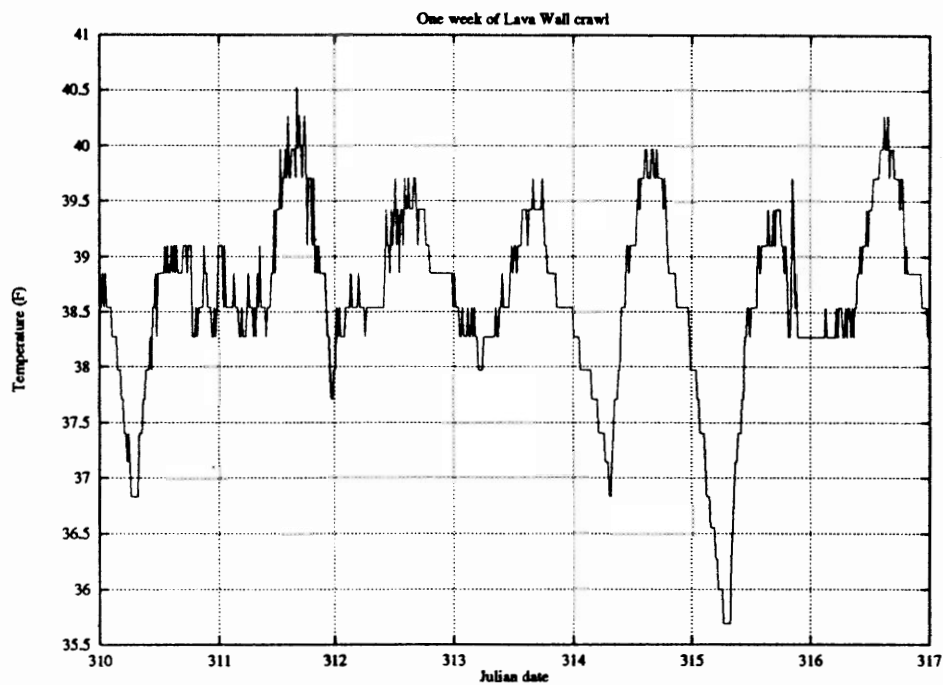
Figure 4.23: One week of temperatures for the crawl in Lava Wall.
