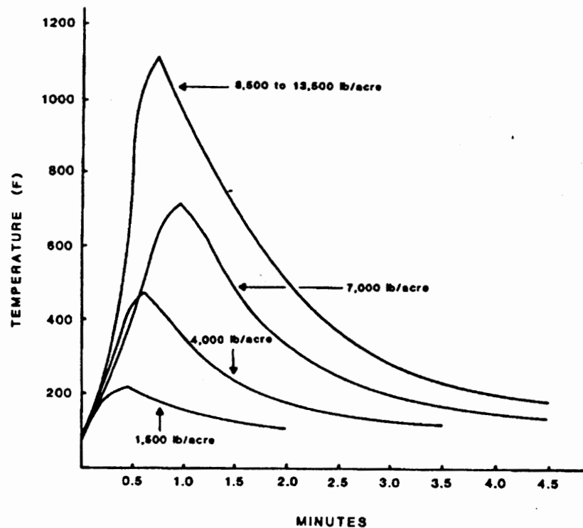
Figure 2.1: Time-temperature curves at the soil surface during prescribed grass fires for four amounts of fine fuel. At the time of burning, air temperature, relative humidity, and wind were 21°C to 27°C, 20 to 40 percent, and 13-24 km/h. (reproduced without permission from [42])
