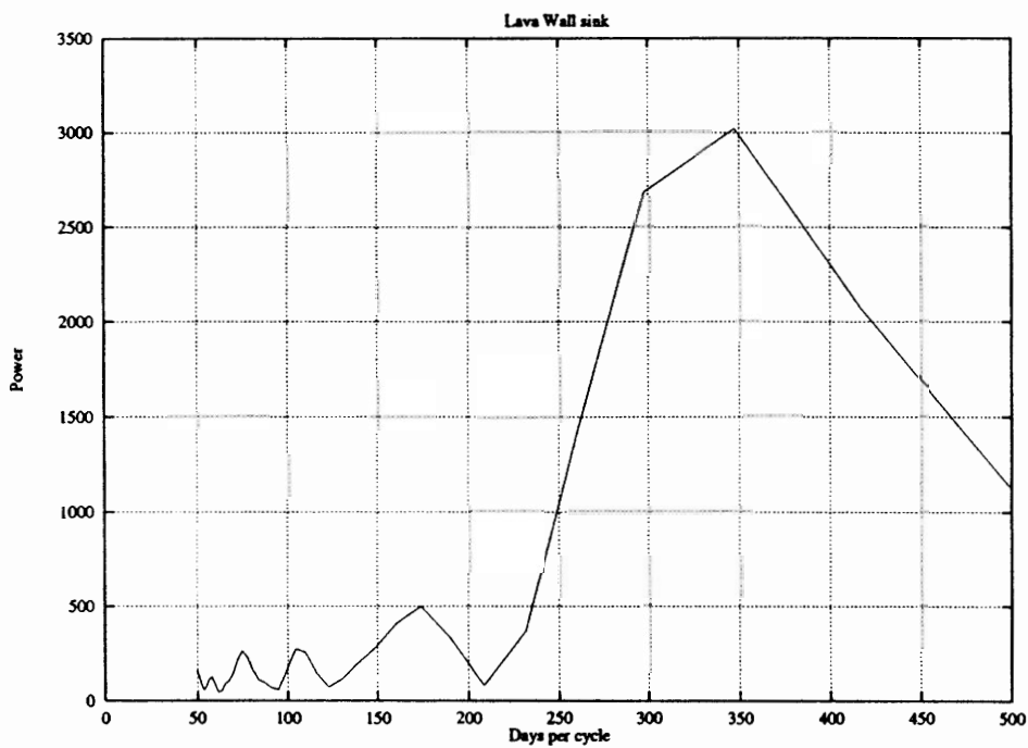
Figure 4.44: Power spectrum for cycles longer than one day for the Lava Wall sink temperature.
