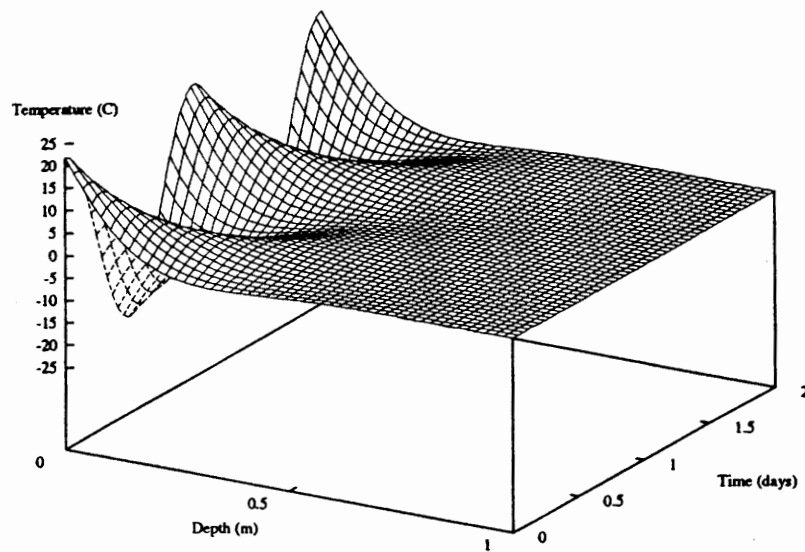
Figure 4.4: Plot showing temperature versus time and distance which illustrates the conduction of heat into the lava. This plot shows two days of solar heating. Distance is in meters, temperature is in C.
