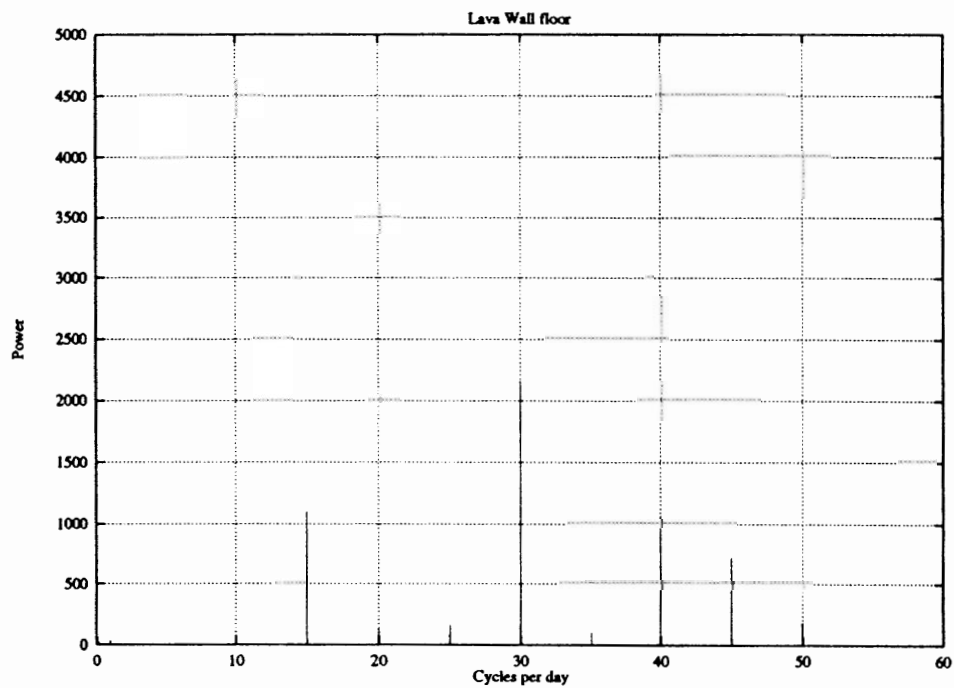
Figure 4.32: Power spectrum for the Lava Wall floor temperature.
