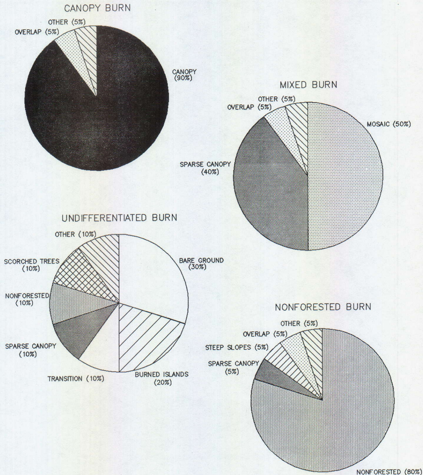
Figure 3. Composition of each map unit as estimated from aerial photographic data from 10 test areas (295,420 acres). See text for description.
