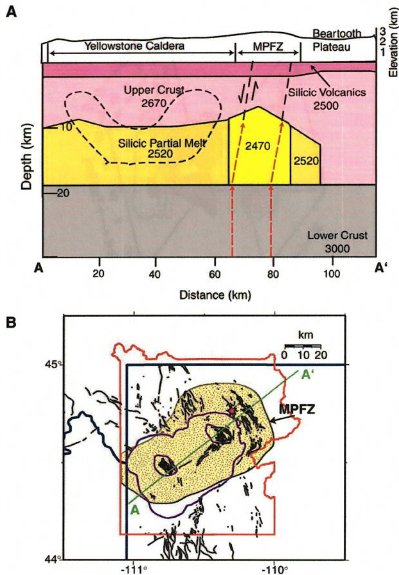
Fig. 8. (A) Cartoon illustrating possible magma movement northeast of the Yellowstone caldera. Southwest dipping extensional faults of the Mirror Plateau Fault Zone (MPFZ) facilitate magma movement. Densities in \text{kg/m}^3 . Red arrows indicate magma movement. (B) Map of the Yellowstone area. Purple outlines the 0.6 Ma caldera. Pink star is the location of Hot Springs Basin Group hydrothermal system. Yellow stipple pattern shows the lateral extent of partial melt derived from our density model.
