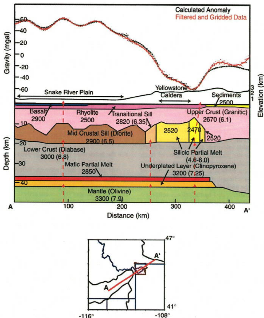
Fig. 12. Cross section of the YSRP density model reflecting the results of previous studies and the velocity–density composition analysis of this study. Numbers in parentheses represent P wave velocities (km/s). Line above cross section represents the generalized topography (km above sea level).
