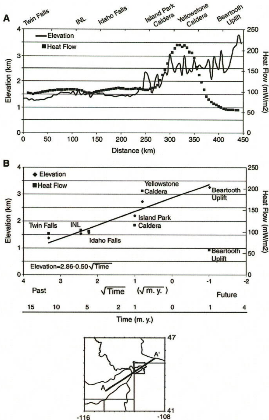
Fig. 13. Generalized relationships between elevation (km), heat flow (mW/m 2 ), and volcanic age along the track of the Yellowstone hotspot. A. Plots of elevation (km) and surface heat flow from Blackwell and Richards (2004). Heat flow and elevation increase with increasing distance along the hotspot track. B. A plot of elevation and heat flow vs. the square root of time (where time is the age of silic volcanic rocks in millions of years from Armstrong et al. (1975)) shows an approximately linear decay of elevation with the square root of time comparable to the lithospheric cooling described by Smith and Braille (1993).
