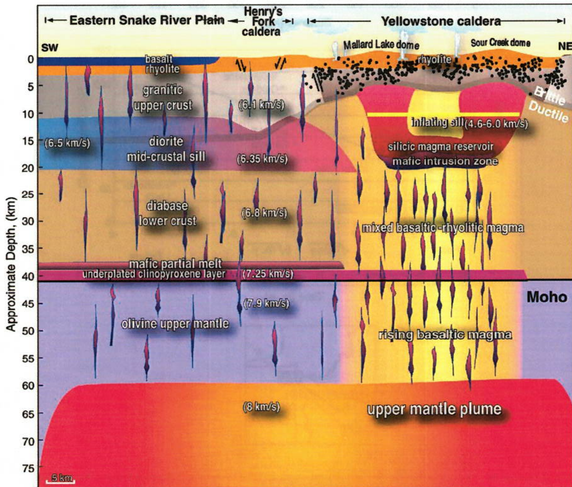
Fig. 14. Cross section of the YSRP summarizing the model of crustal structure, composition and magmatic processes interpreted from this and other studies.
