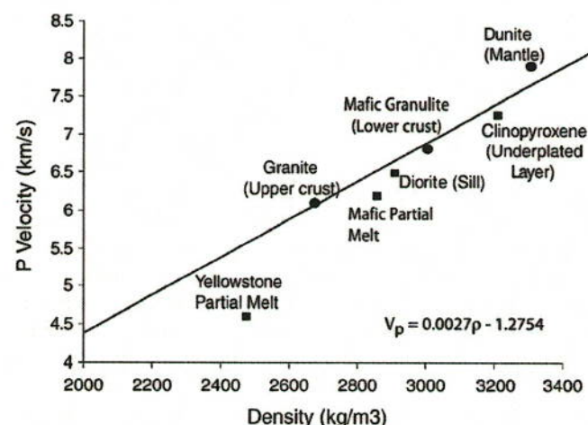
Fig. 9. Velocity–density plot for rocks in the YSRP volcanic field. Circles are rocks with densities inferred from other studies and squares are densities of rocks evaluated in this study. The Yellowstone upper crustal partial melt and mafic melt were not included in the calculation of the linear equation.
