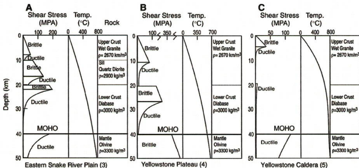
Fig. 11. Strength models of the eastern SRP, Yellowstone Plateau, and Yellowstone caldera. Profile locations and respective strain rates are shown in Fig. 10.
