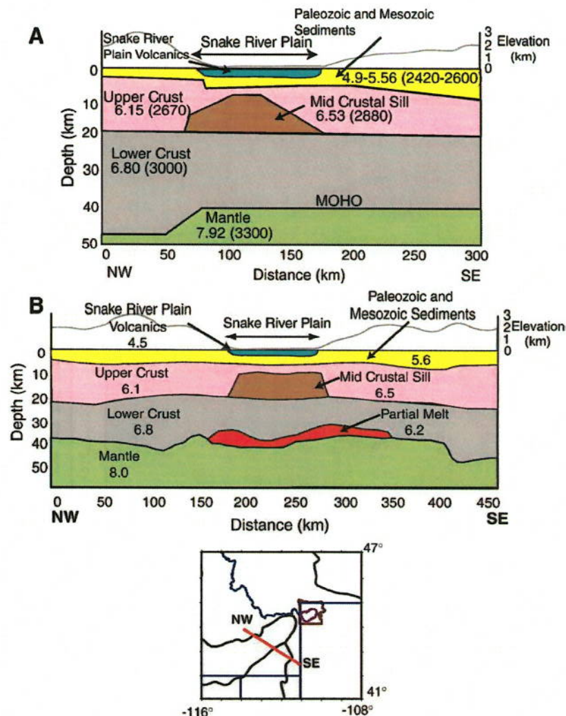
Fig. 4. (A) Crustal structure of the SRP determined from the seismic refraction study of Sparlin et al. (1982). (B) Crustal structure of the SRP determined from the seismic receiver function analysis of Peng and Humphreys (1998). Red line on the map represents the approximate location of both profiles. Velocities in km/s. Numbers in parentheses are densities in kg/m 3 . Lines above the models represent generalized topography (km above sea level).
