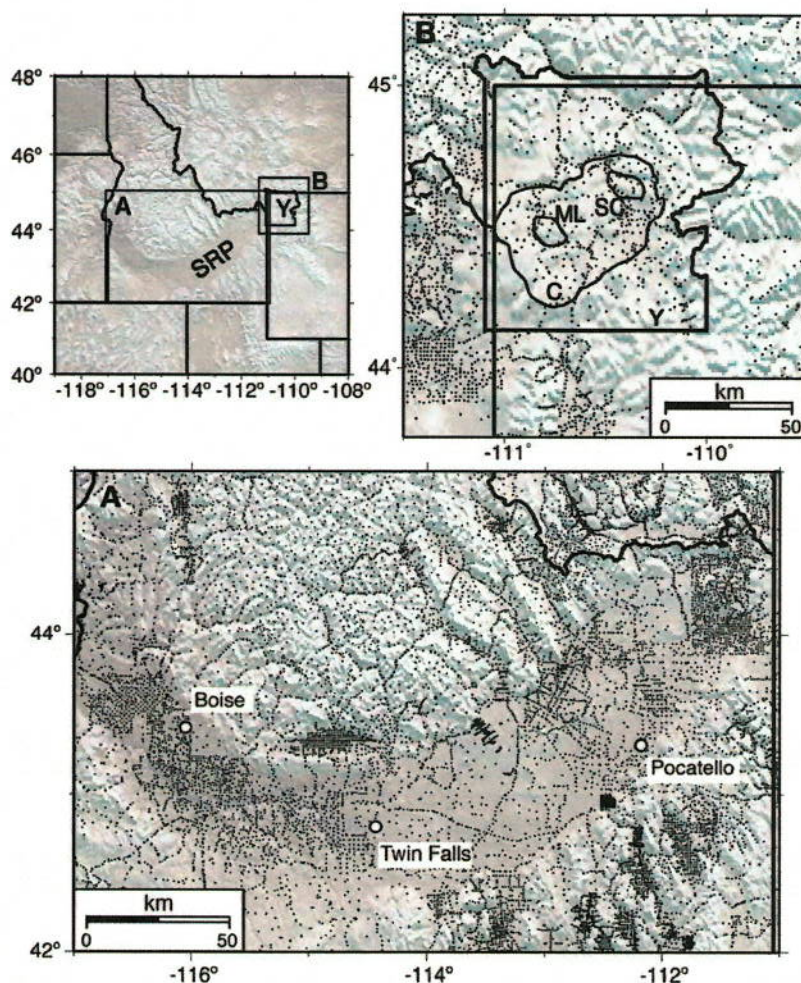
Fig. 2. Map showing the distribution of gravity stations in the SRP (A) and Yellowstone (B). Black dots are gravity stations. Yellowstone National Park (Y), the Snake River Plain (SRP), the 0.6 Ma Yellowstone caldera (C), Mallard Lake resurgent dome (ML), and Sour Creek resurgent dome (SC) are marked.
