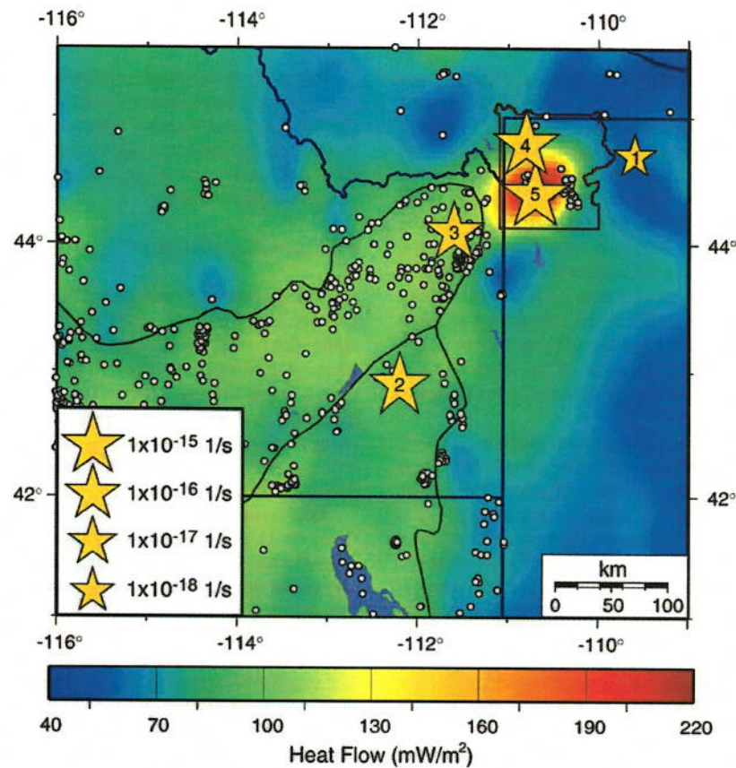
Fig. 10. Map showing heat flow from Blackwell et al. (2007) and the locations of the calculated strength profiles from rheologic modeling. Strain rates at each location from Puskas et al. (2007). Circles represent the location of boreholes used to determine heat flow values.
