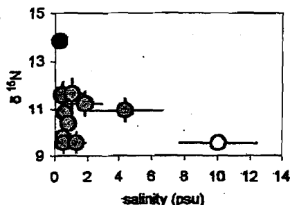
Figure 6. Average \delta^{15}\text{N} (‰) values of grass shrimp muscle tissue vs. average salinity for the 12 sampling stations. Samples were collected 11 times between Dec. 2000 and July 2002. Error bars represent 95% confidence levels. The black and white symbols stand for the stations closest to the diversion and marine station, respectively.
