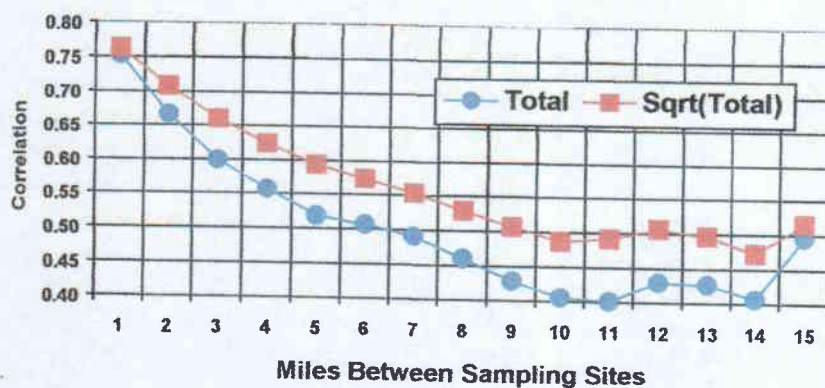
Figure 16. Spatial correlations between sampling locations
