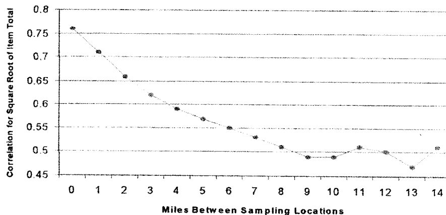
Figure 17. Average correlation vs. sampling distance (miles)
