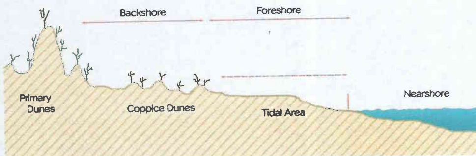
Figure 3. Shoreline zones
