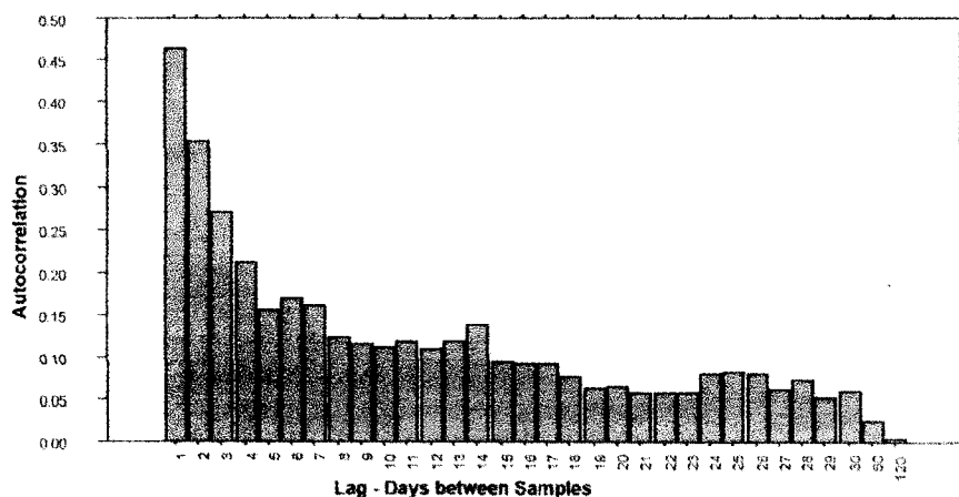
Figure 18. Autocorrelation vs. days between sampling
