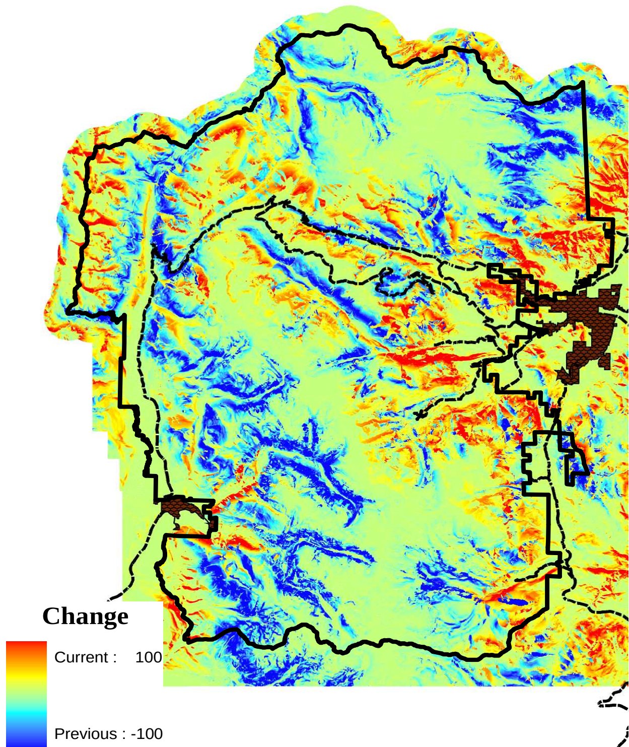
Figure 5. Map illustrating shift in predicted suitable black bear den locations from 1984–2006 in Rocky Mountain National Park, Colorado. Cooler colors represent sites historically suitable for denning but currently less utilized, while warmer colors illustrate areas currently selected for den sites but were previously less suitable. Roads are depicted by dashed lines, while brown cross-hatched areas represent urban sites.
