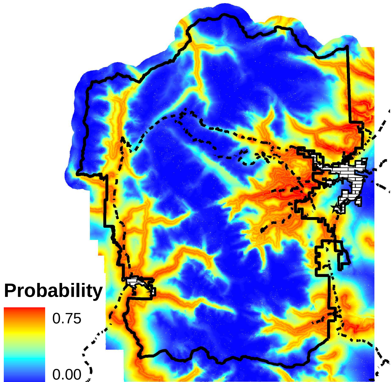
Figure 2. Map depicting probability of use by black bears in Rocky Mountain National Park (RMNP), Colorado from 2003–2006. Variables nested within the model include distance to trails and slope. The RMNP boundary is demarcated by a solid black line, roads are depicted by dashed lines, while white-bricked areas represent urban sites.
