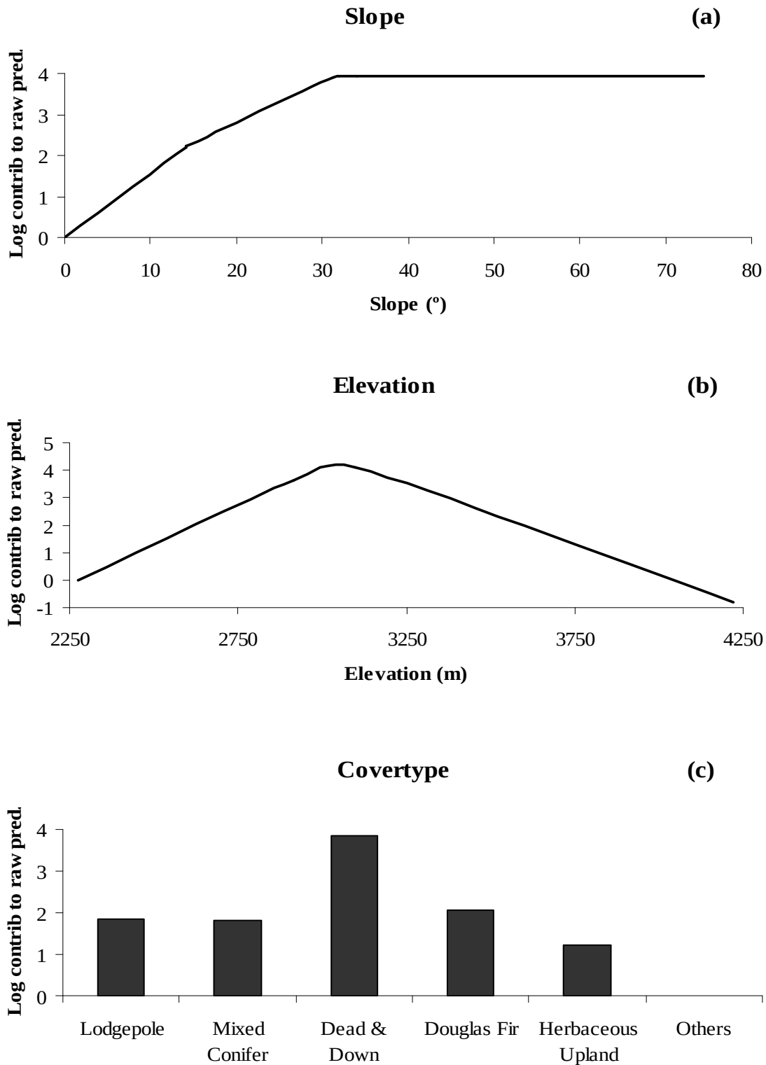
Figure 2. Relationships between the exponential contribution of slope (a), elevation (b), and covertype (c) to the raw prediction score and the observed value for 35 black bear den sites observed from 1984–1991 in Rocky Mountain National Park, Colorado.
