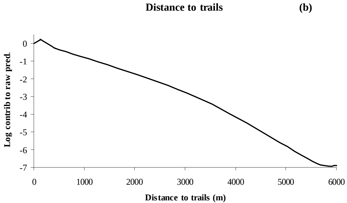
Figure 1. Relationships between the exponential contribution of elevation (a) and distance to trails (b) to the raw prediction score and the observed value for 9 bears from 2003–2006 in Rocky Mountain National Park, Colorado.
