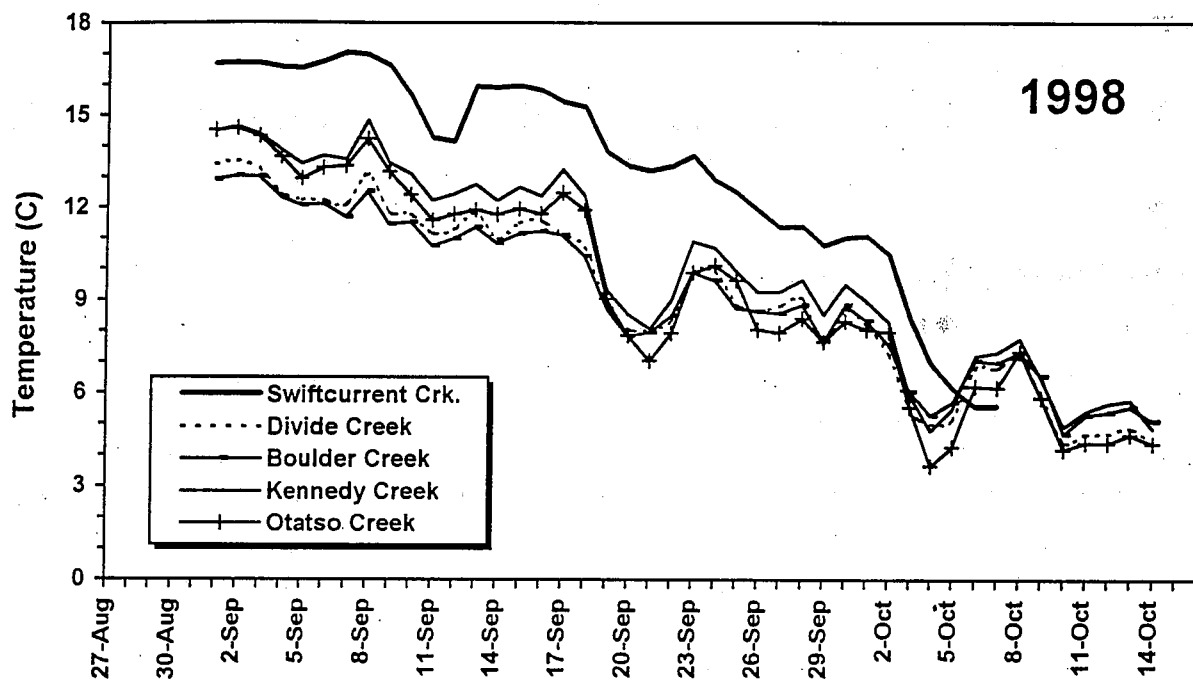
Figure 2. Mean daily stream temperatures (°C) in Swiftcurrent, Divide, Boulder, Kennedy and Otatso creeks, Saint Mary River drainage, Montana, Aug.-Oct., 1997-98.
