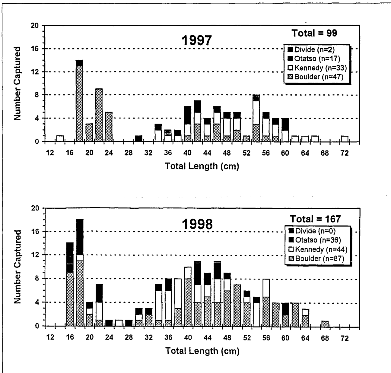
Figure 8. Length-frequency distribution for all bull trout captured in fish traps in the Saint Mary River Drainage, Montana, 1997-98.
