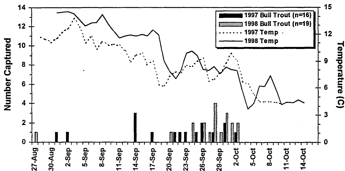
Figure 6. Chronology of captures of downstream-migrating adult bull trout and corresponding mean daily temperatures ( ^{\circ}\text{C} ) in Otatso Creek, Saint Mary River drainage, Montana, August-October, 1997-98.
