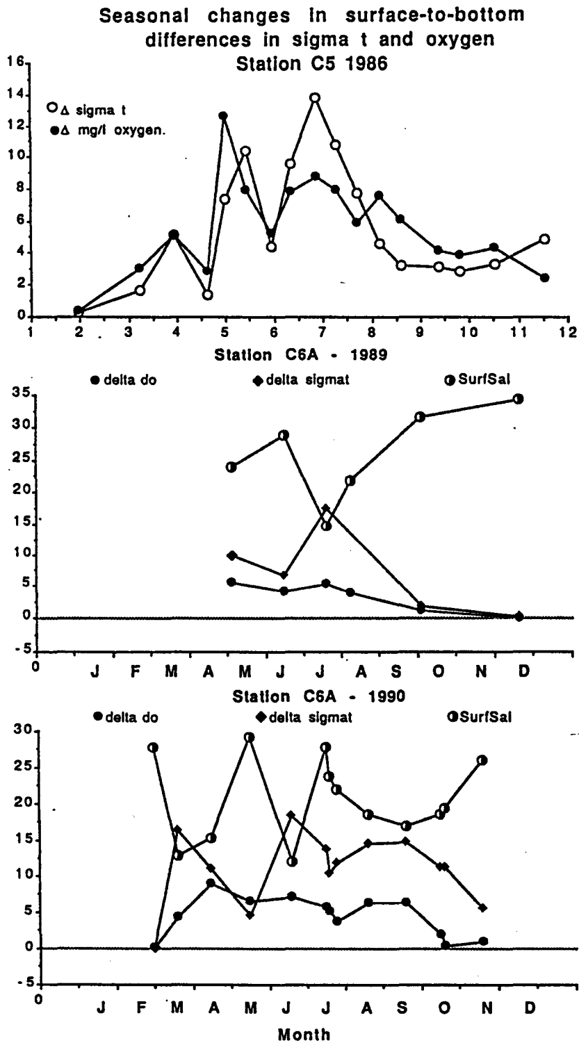
Figure 2. Changes in intensity of stratification and surface-to-bottom oxygen differences in three years (modified from Rabalais et al. 1991b).
