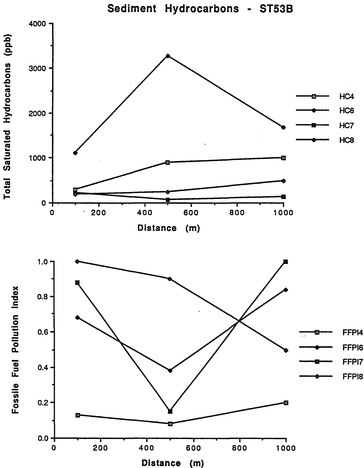
Figure 20. Distribution of total saturated hydrocarbons (top) and FFPI (bottom) for Unocal ST53B for months April (4), June (6), July (7) and August (8).
