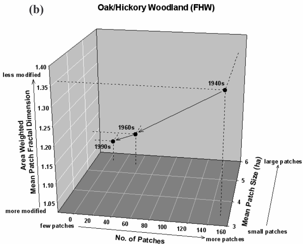
Figure 4-34: 3D landscape metrics space for (a) upland scrub, and (b) oak/hickory woodland at WICR showing the magnitude and direction of change
