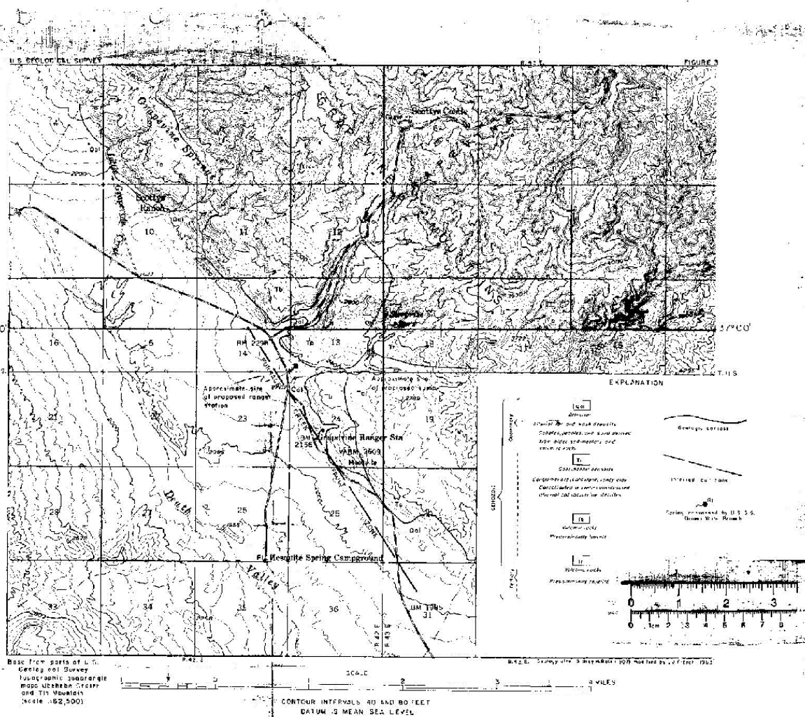
FIGURE 3-RECONNAISSANCE GEOLOGIC MAP OF GRAPEVINE RANGER STATION AREA, DEATH VALLEY NATIONAL MONUMENT CALIFORNIA
