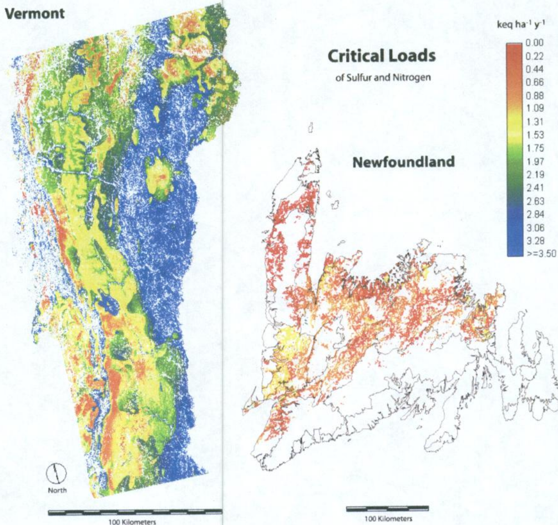
Figure 1. Critical load of sulfur + nitrogen deposition to upland forested areas of (a) Vermont and (b) Newfoundland. Sulfur + nitrogen atmospheric deposition rates higher than the critical load result in greater exports of nutrient cations ( \text{Ca}^{2+} , \text{Mg}^{2+} , \text{K}^+ ) than inputs and eventual deterioration of soil fertility, forest health, and forest productivity. Critical loads are expressed in kilo-equivalents per hectare per year; nitrogen deposition includes both ammonium + nitrate forms.
