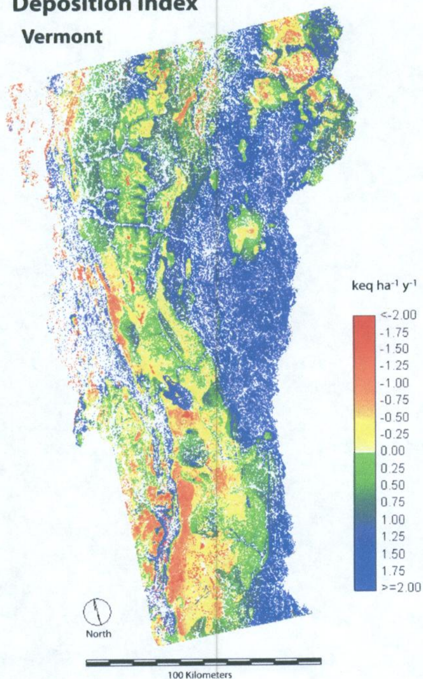
Figure 5. The deposition index for atmospheric sulfur and nitrogen deposition to Vermont (1996-1999) with respect to forest ecosystem critical loads. Positive values of the deposition index reflect the capacity of a forest ecosystem to tolerate additional acidic deposition. Negative values of the index correspond to the reduction in S and N deposition required to eliminate present or deter the development of future nutrient limitations. Red areas indicate current sulfur and nitrogen atmospheric deposition rates greater than the critical load. The deposition index is expressed in terms of the kilo-equivalents of charge per hectare per year. Nitrogen deposition includes both ammonium + nitrate forms.
