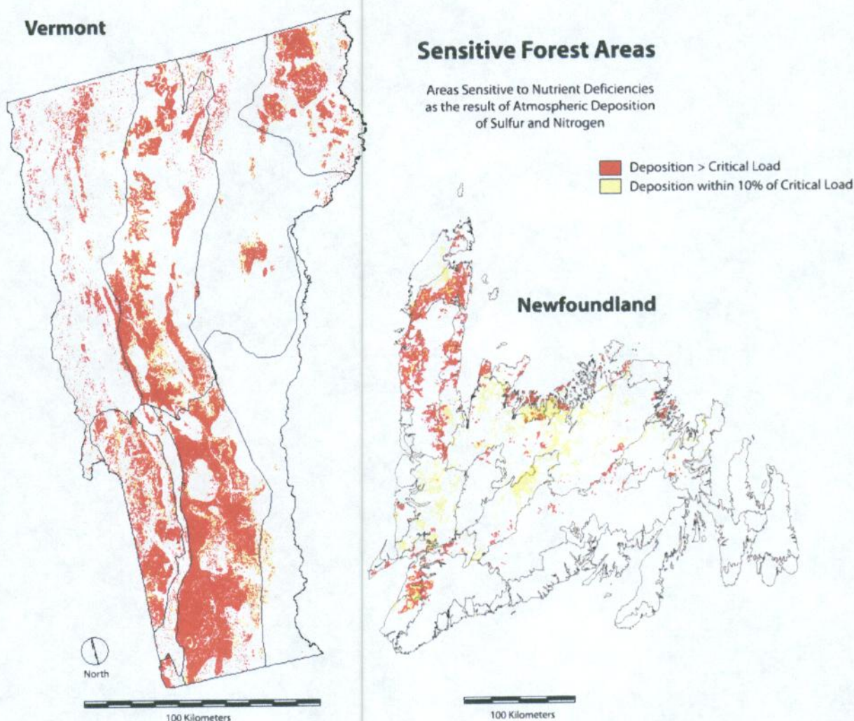
Figure 2. Forested Areas of (a) Vermont and (b) Newfoundland that are sensitive to the negative effects of combined atmospheric sulfur and nitrogen deposition. Red areas indicate current sulfur and nitrogen atmospheric deposition rates greater than the critical load. Yellow areas indicate current atmospheric deposition rates within 10% of the critical load.
