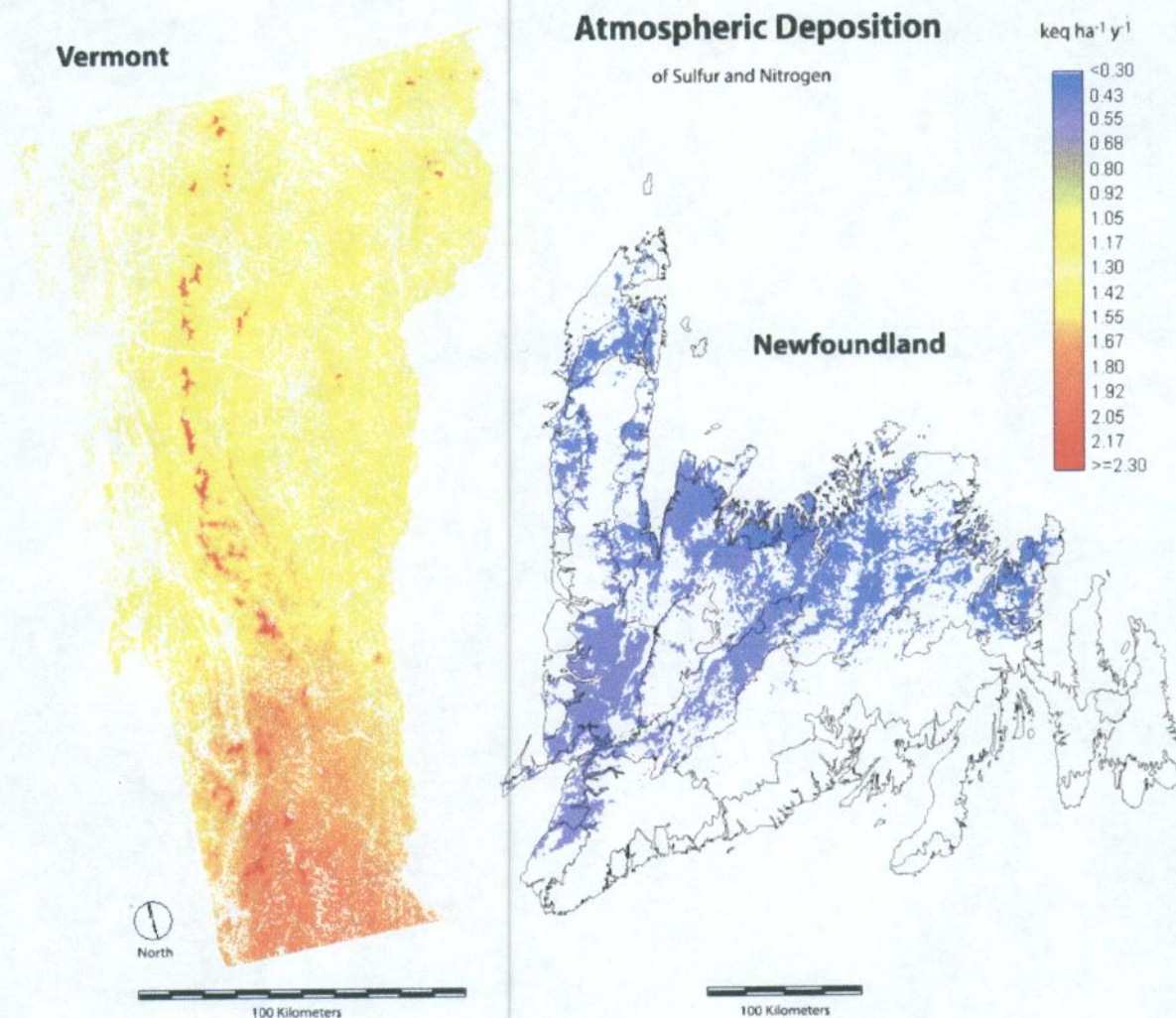
Figure 4. Average annual atmospheric deposition of sulfur and nitrogen to (a) Vermont (1996-1999) and (b) Newfoundland (1994-1997). Total deposition (particle + \text{SO}_2 + precipitation + cloud water [VT only]) expressed in terms of the kilo-equivalents of charge per hectare per year; nitrogen deposition includes both ammonium + nitrate forms. This represents the total base-neutralizing and cation-leaching power of S and N atmospheric deposition.
