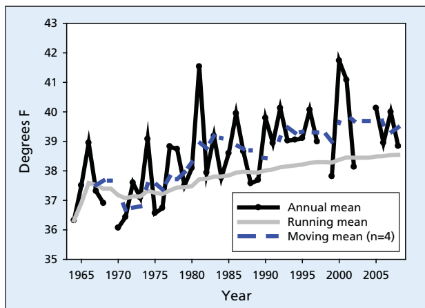
Average annual minimum temperature, Pipe Spring NM.
