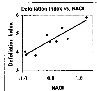
Correlation between NAO Index and defoliation due to insects.
