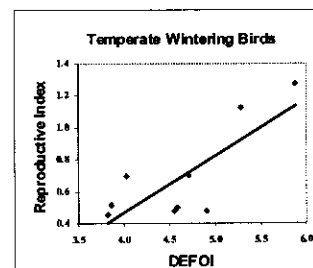
Correlation between defoliation index and reproductive index of temperate wintering birds.
