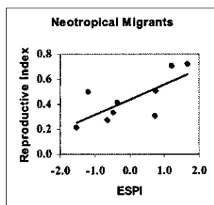
Correlation between El Niño Southern Oscillation Index (ESPI) and reproductive index of neotropical migrants.
