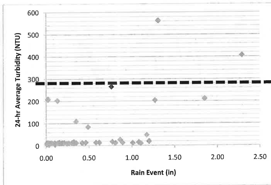
Figure 4.7: 24-hr average turbidity with 280-NTU limit for RH.
