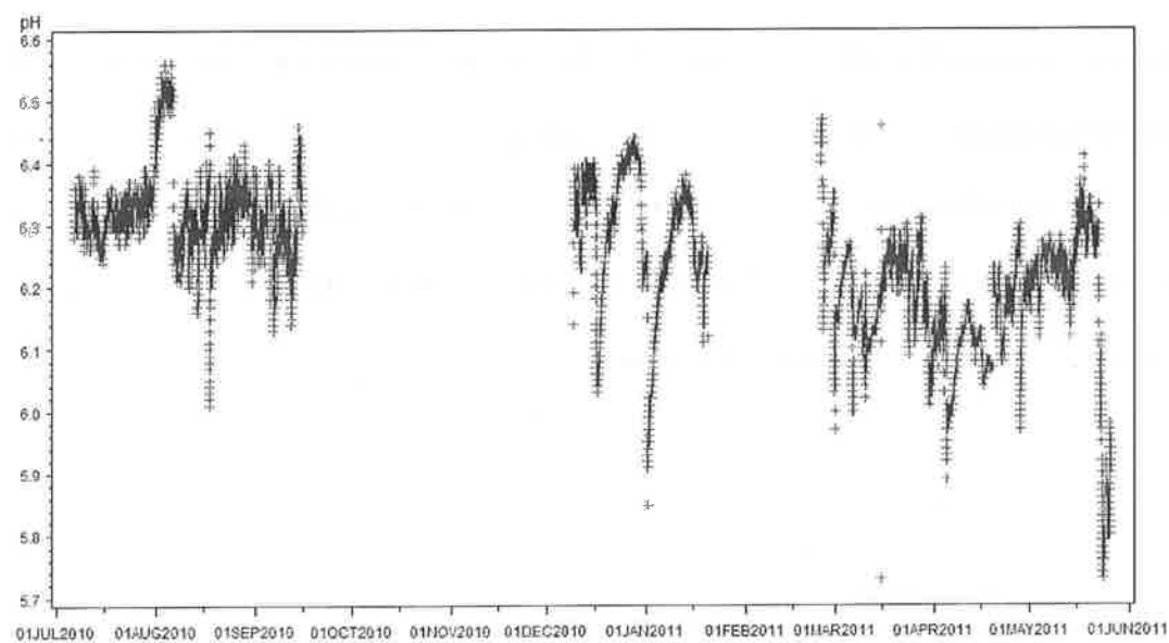
Figure 4.9: Annual pH fluctuations for DH.
