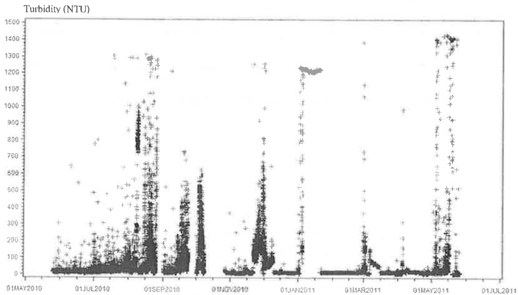
Figure 4.2: Annual turbidity fluctuations for HH.
