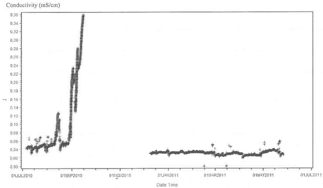
Figure 4.1: RH conductivity plot showing incorrect data readings.
