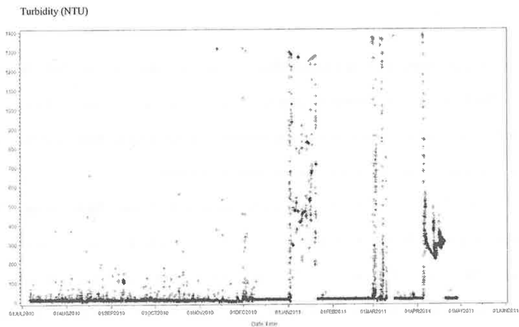
Figure 4.3: Annual turbidity fluctuations for DH.
