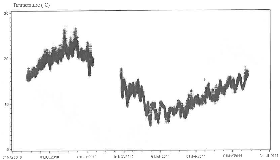
Figure 4.14: Annual stream temperature fluctuations for HH.
