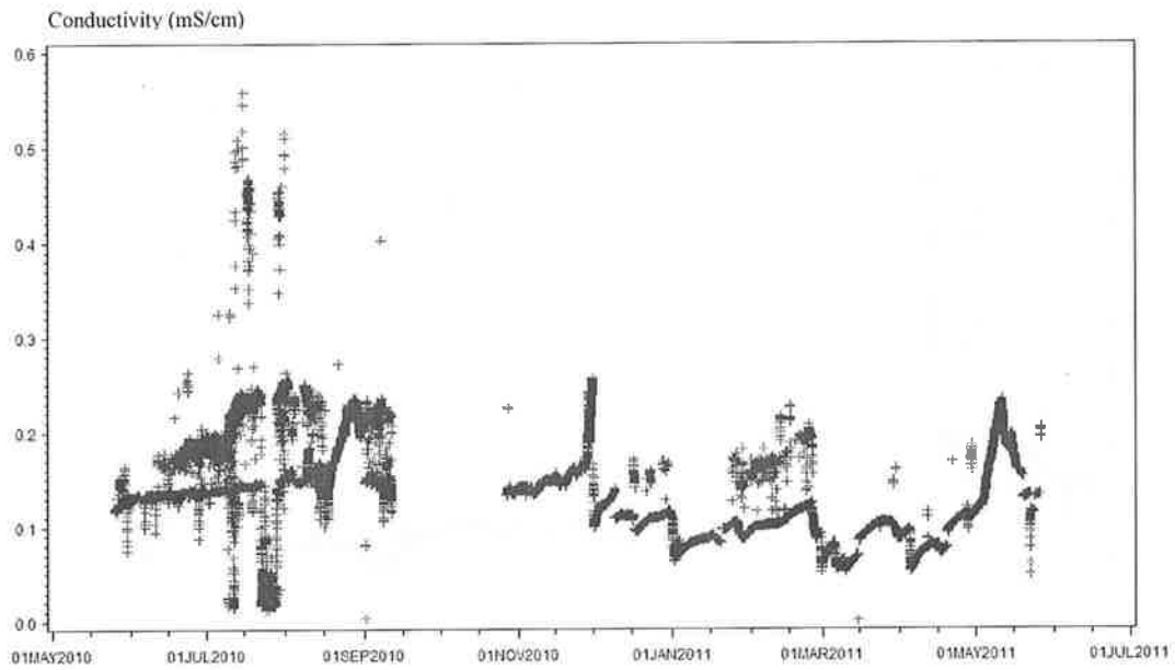
Figure 4.11: Annual conductivity fluctuations for HH.
