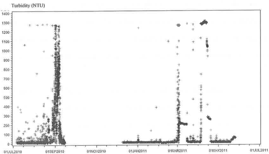
Figure 4.4: Annual turbidity fluctuations for RH.
