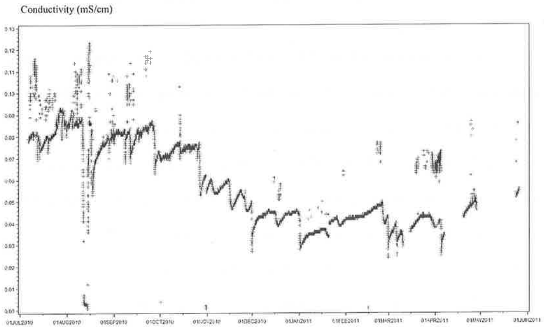
Figure 4.12: Annual conductivity fluctuations for DH.
