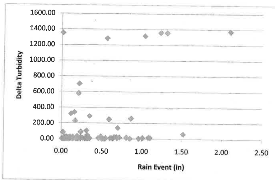
Figure 4.19: Change in turbidity vs rain for DH before removing outliers.
