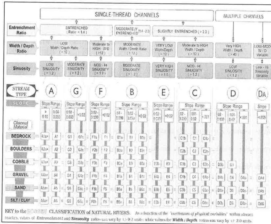
Figure 3.8: Rosgen stream classification system (Rosgen, 1996).
