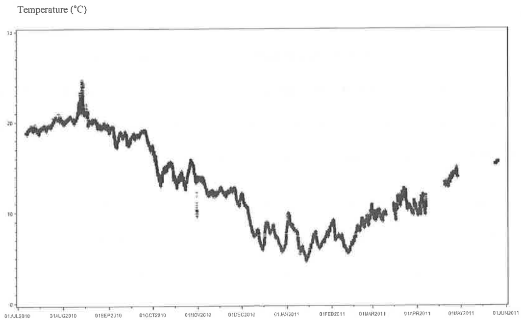
Figure 4.15: Annual stream temperature fluctuations for DH.
