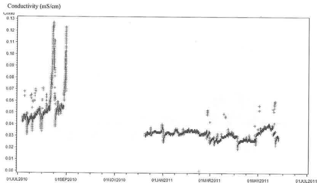
Figure 4.13: Annual conductivity fluctuations for RH.
