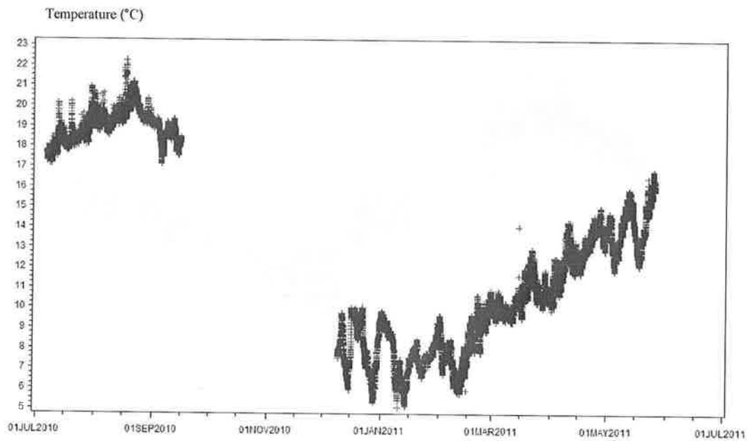
Figure 4.16: Annual stream temperature fluctuations for RH.
