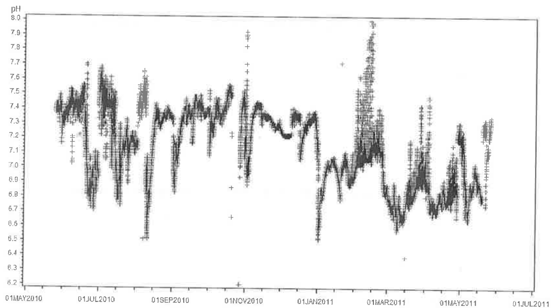
Figure 4.8: Annual pH fluctuations for HH.
