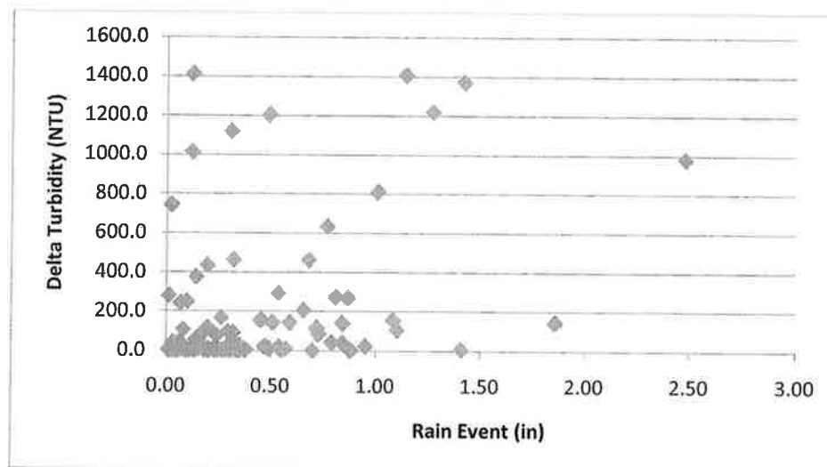
Figure 4.17: Change in turbidity vs rain for HH before removing outliers.
