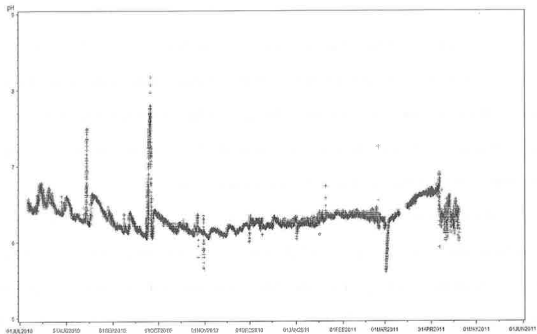
Figure 4.9: Annual pH fluctuations for DH.
