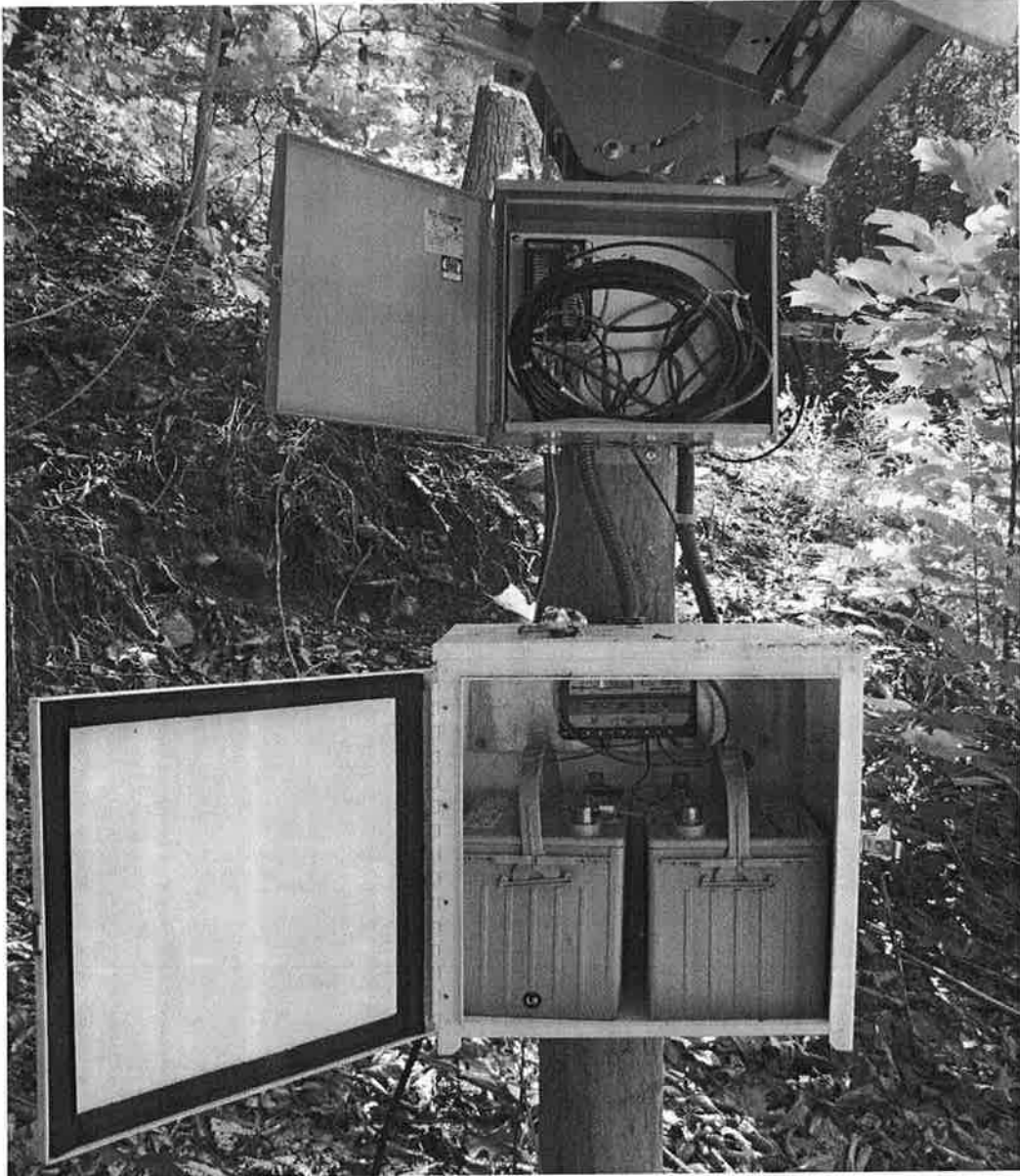
Figure 3.10: Wireless communication, datalogging, and power equipment at HH.
