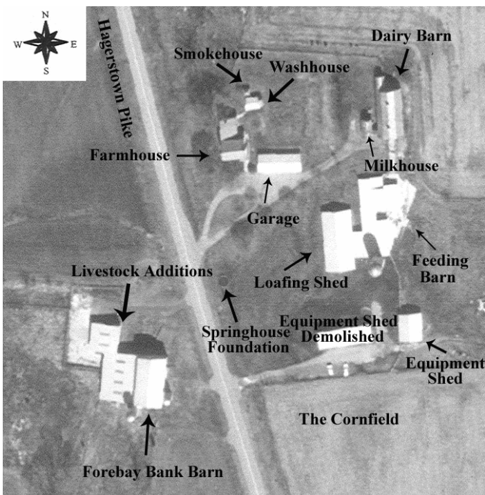
Site plan of D. R. Miller Farmstead, showing relationship between domestic and agricultural outbuildings. Aerial photograph dated 2000.
