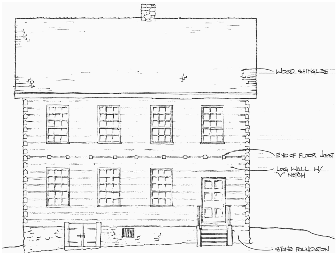
Conjectural elevation of the Miller farmhouse as it may have appeared when originally built. Reprinted from Oehrlein & Associates, Miller Farmstead Historic Structures Report (Washington, DC: Oehrlein & Associates, 1993), 86.
