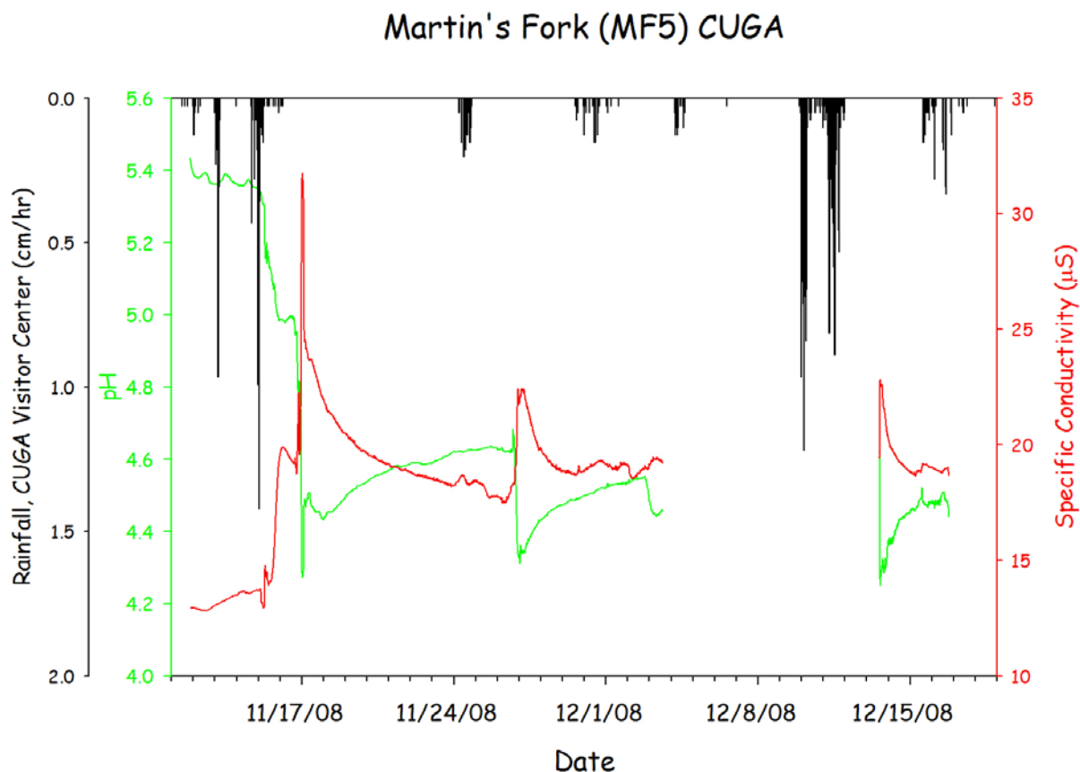
Figure 19. pH and SpC response to rainfall at Martin's Fork,
