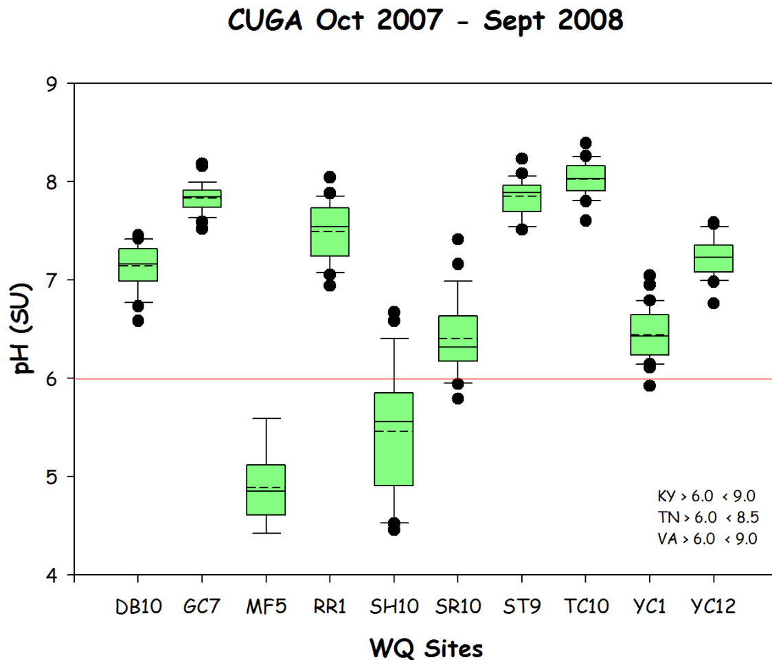
Figure 16. pH at CUGA
