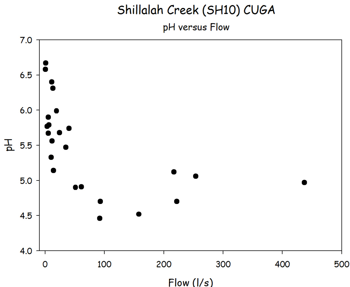
Figure 18. pH versus flow at Shillalah Creek.
