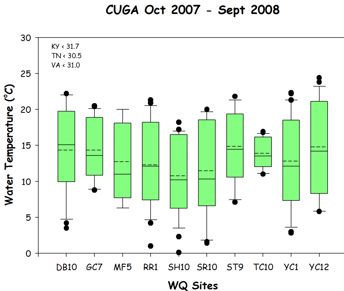
Figure 14. Water temperature at CUGA
