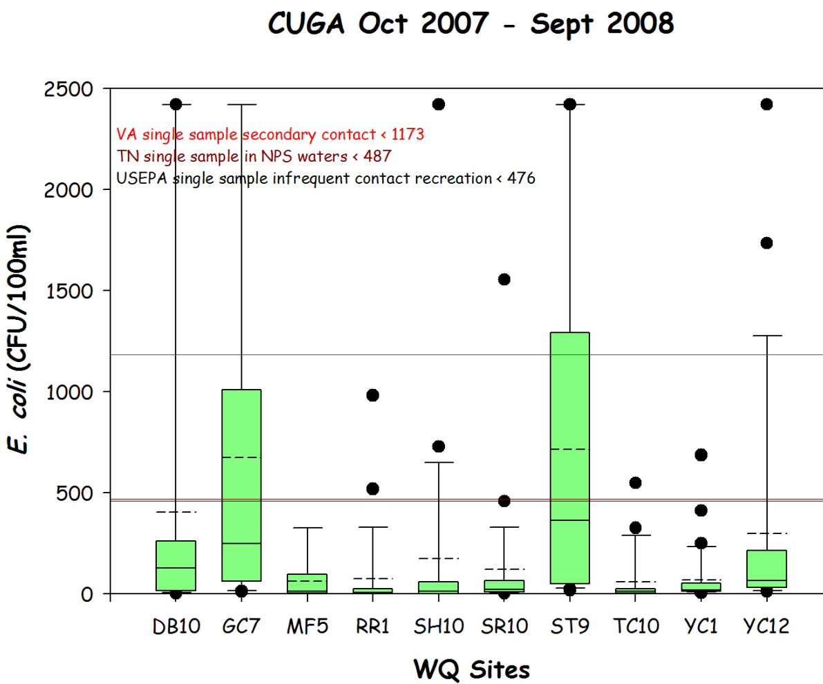
Figure 23. E. coli at CUGA
