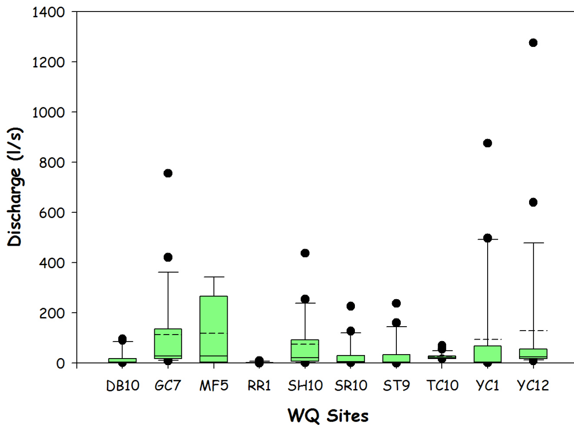
Figure 21. Discharge at CUGA
