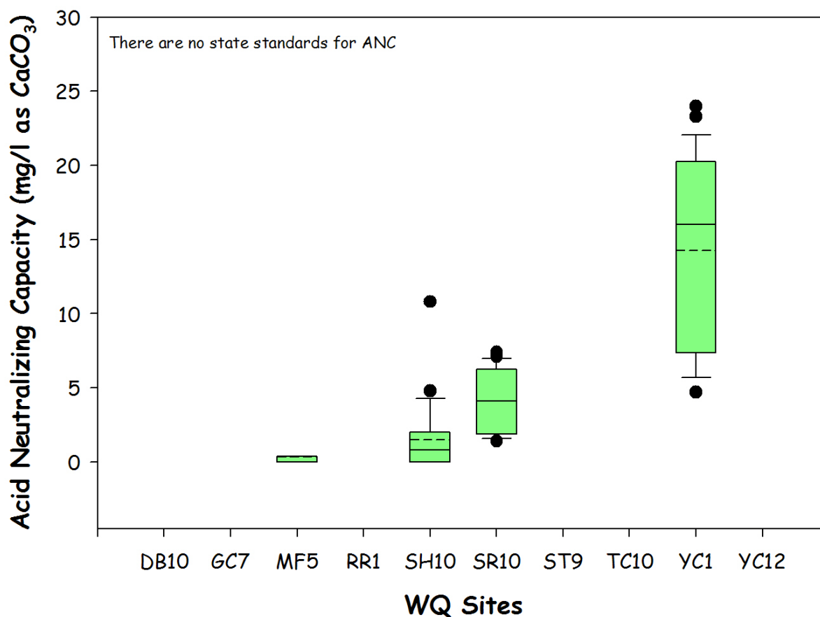
Figure 22. Acid Neutralizing Capacity at CUGA
