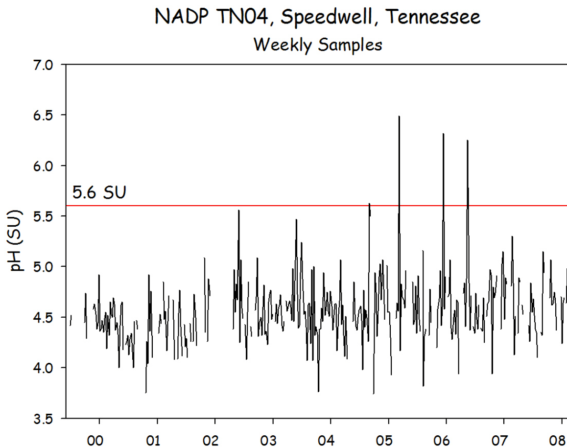
Figure 17. pH at NADP site in Speedwell Tennessee.
