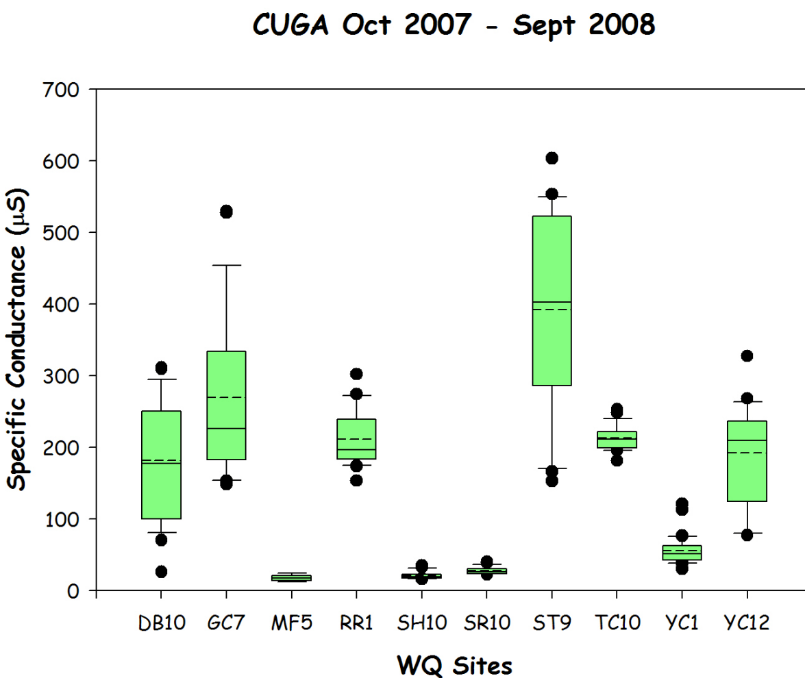
Figure 15. Specific Conductance at GUGA
