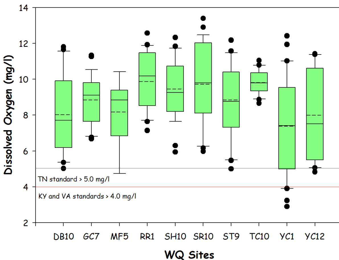
Figure 20. Dissolved Oxygen at CUGA
