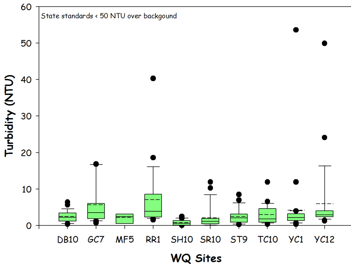
Figure 26. Turbidity at CUGA
