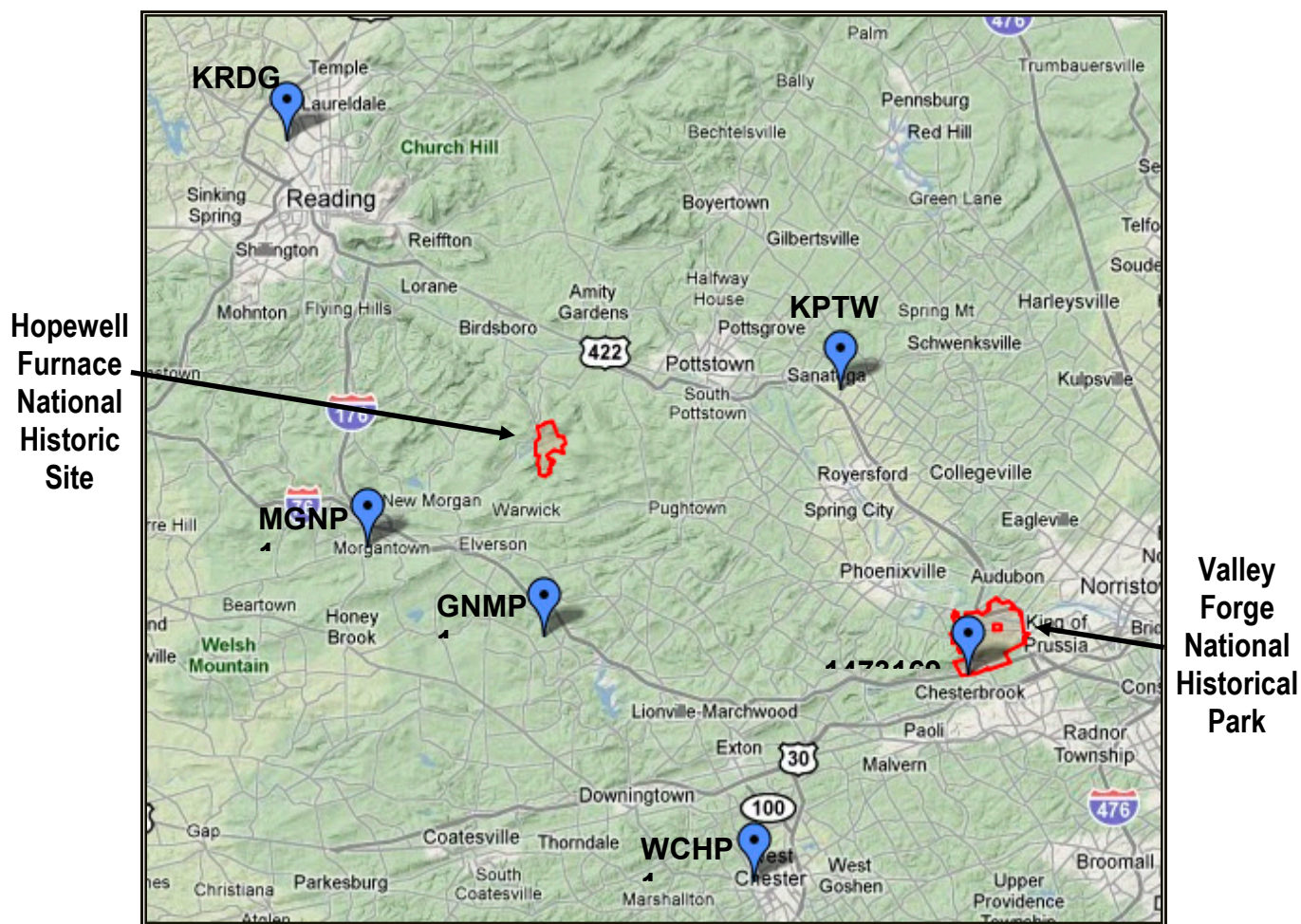
Figure 1. Location of weather observing stations around Hopewell Furnace National Historic Site and Valley Forge National Historical Park selected as most representative of the parks in 2011. See Table 1 for station names.
