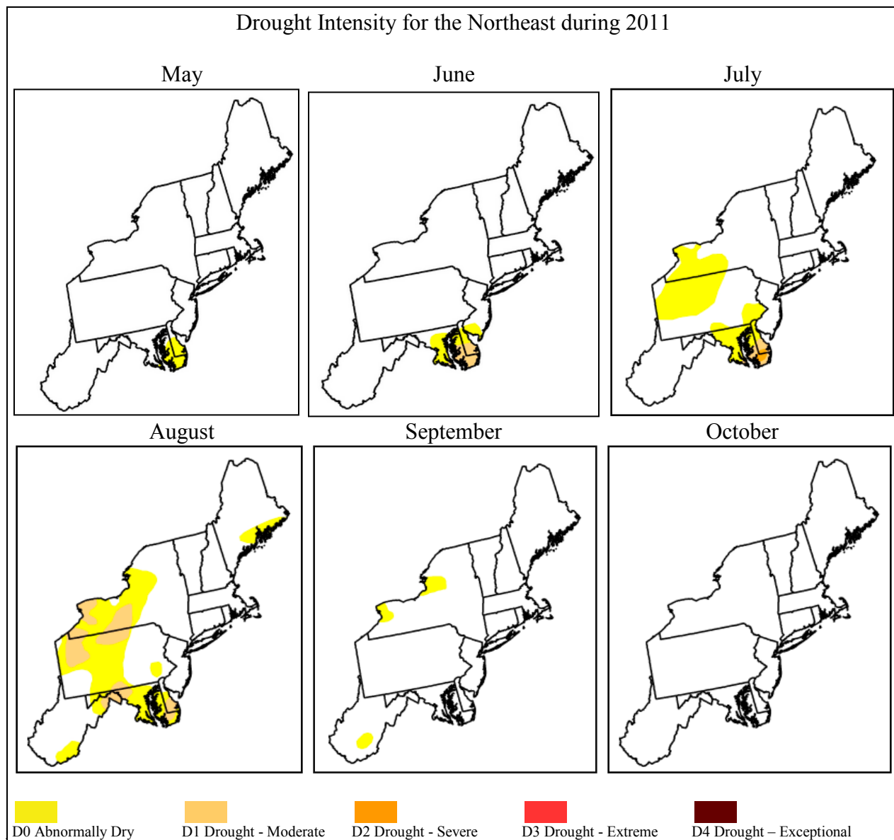
Figure 7. Mid-month values of the United States Drought Monitor (DM) – Drought Intensity Index for the Northeast in 2011.
