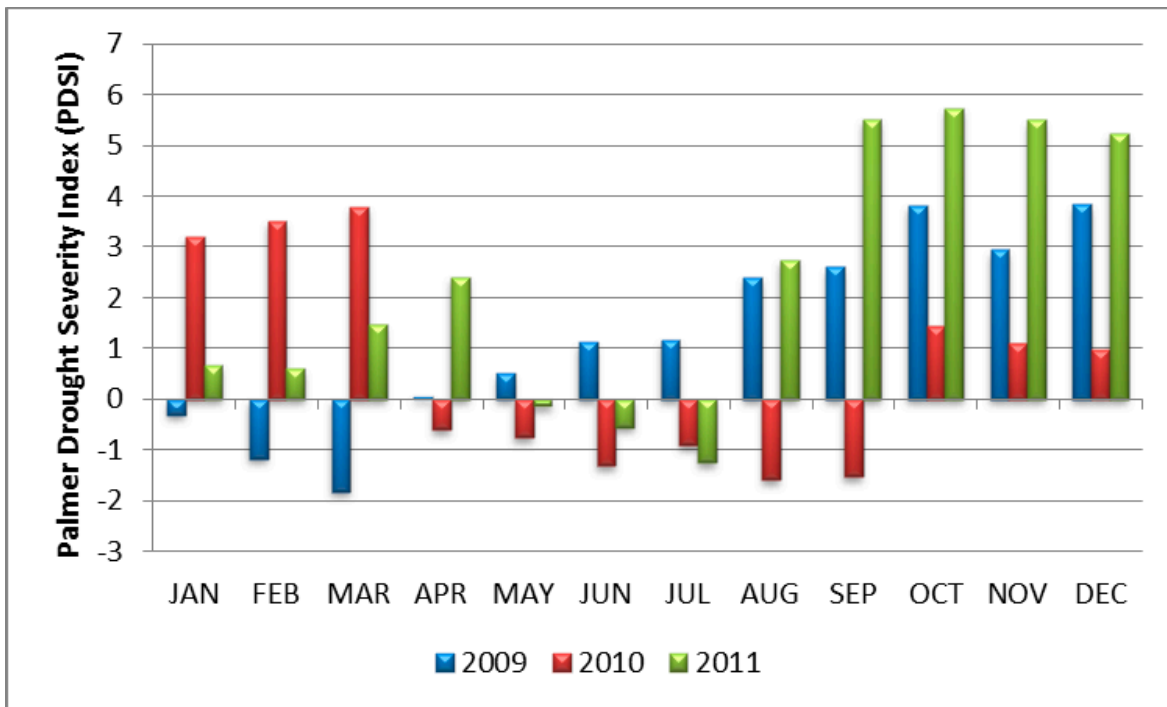
Figure 5. Palmer Drought Severity Index (PDSI) for the Southeastern Piedmont, 2009–2011.
