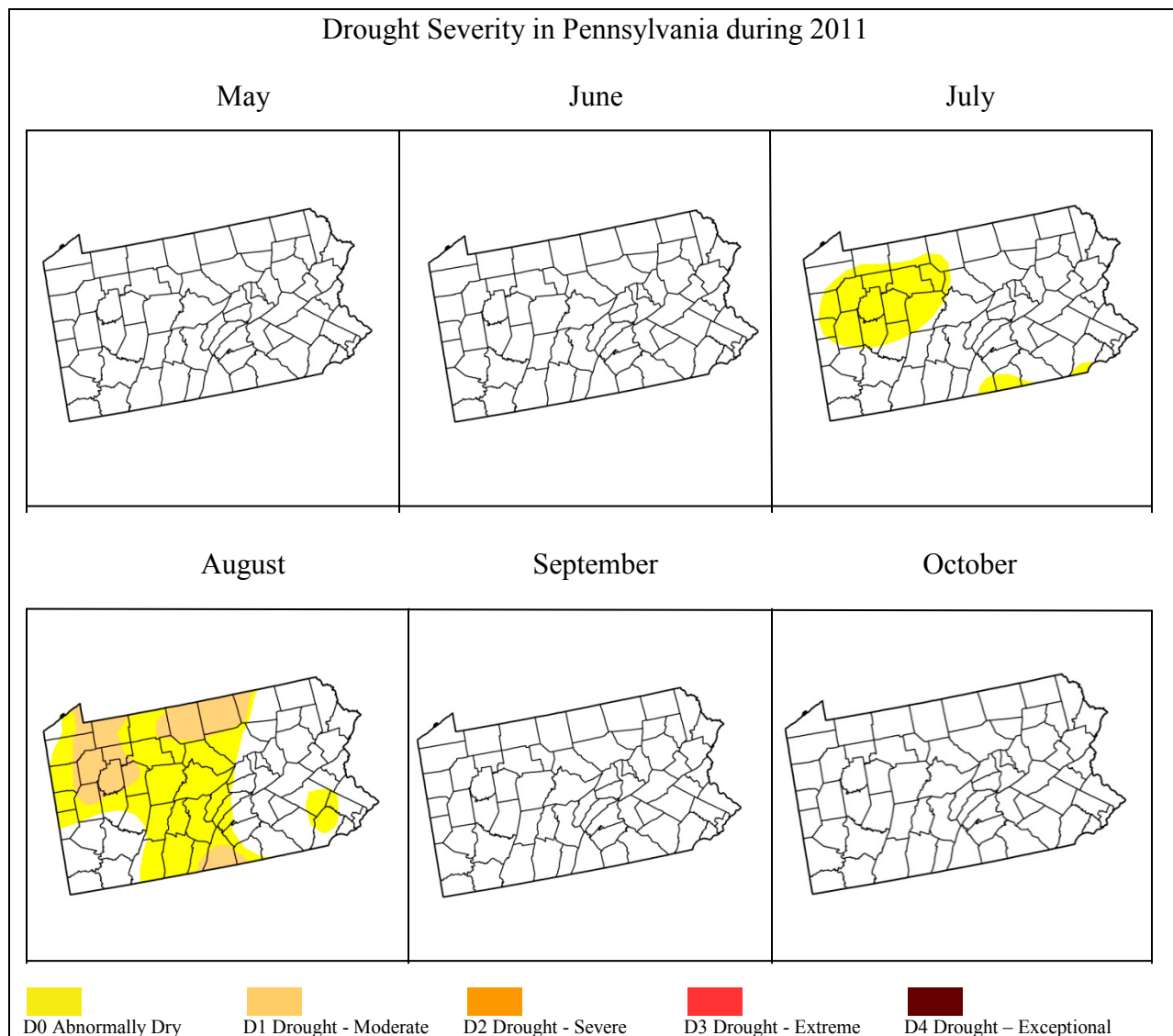
Figure 6. Mid-month values of the United States Drought Monitor (DM) – Drought Intensity Index for Pennsylvania in 2011.
