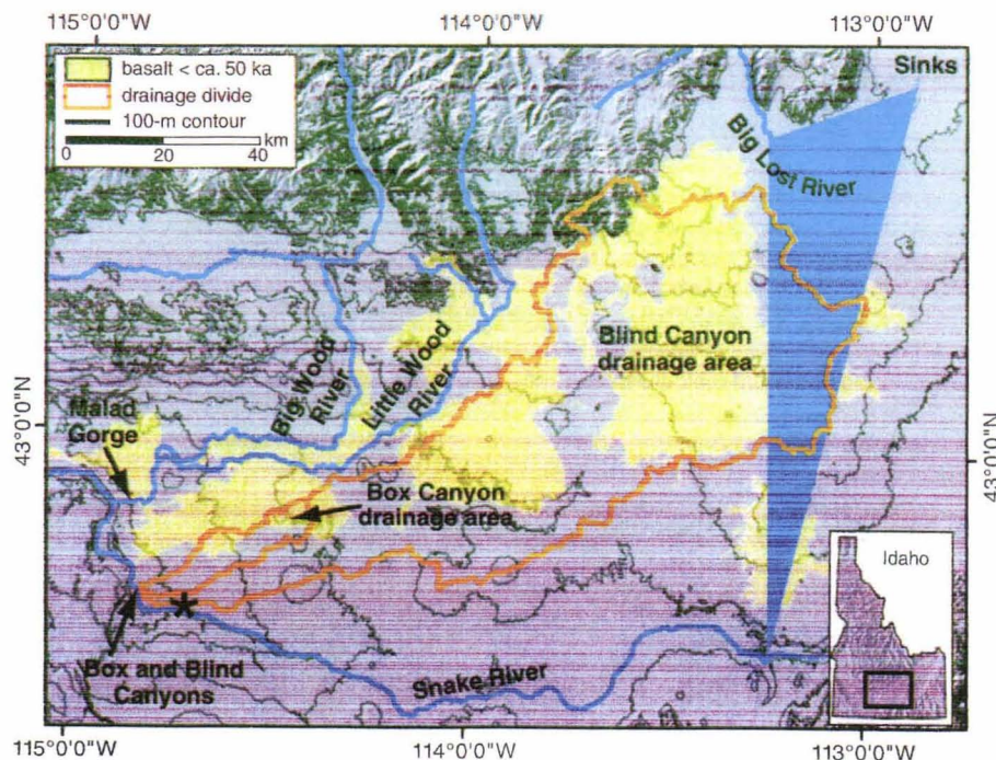
Fig. 2. Topographic map of the eastern Snake River Plain, the location of which is shown on the inset map of Idaho. The drainage areas feeding Box Canyon ( 228 \text{ km}^2 ) and Blind Canyon ( 4713 \text{ km}^2 ) are outlined, following the path of steepest descent. The yellow-shaded regions mark the locations of volcanism younger than \sim 50 \text{ ka} (15). The thin black lines are 100-m topographic contours. Topographic data are from the U.S. Geological Survey. This is a UTM zone 11 projection, NAD83 datum, at 25 m resolution.
