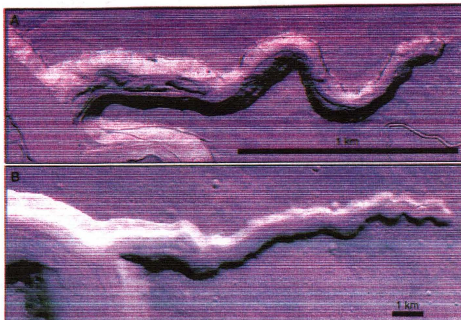
Fig. 1. (A) Shaded relief map of Box Canyon, Idaho. Airborne laser-swath mapping data were collected by the National Center for Airborne Laser Mapping. The data have been filtered to remove vegetation that exists along the creek banks. This is a Universal Transverse Mercator (UTM) zone 11 projection, North American Datum of 1983 (NAD83) datum, at 1 m resolution. (B) Thermal Emission Imaging System (32) infrared daytime image of Marners Vallis, Mars, image V19470014, at 19 m resolution.
