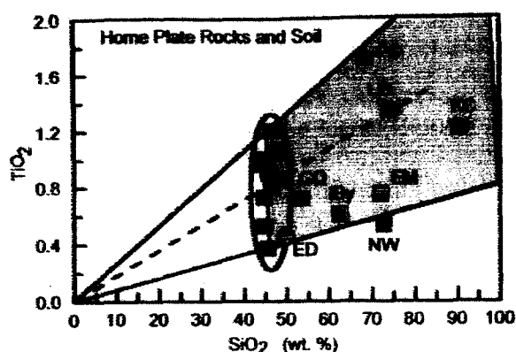
Fig. 5. Plot of titanium dioxide and silica contents for APXS measurements acquired since arriving at Home Plate and including observations from the Eastern Valley, Low Ridge, Mitchelltree Ridge, and the Tyrone areas. Red squares, silica-rich rocks; red circles, silica-rich soils; blue squares, basaltic rocks in the vicinity of Home Plate; and green triangle, typical local soil. The light blue region represents the compositions that can be obtained by acid-sulfate leaching of Home Plate rocks, assuming no variation in the \text{TiO}_2/\text{SiO}_2 ratio. KC, Kenosha Comets; LG, Lefty Ganote; FS, Fuzzy Smith; EM, Elizabeth Mahon; NW, Nancy Warren; ED, Eileen Dean; Iby, Innocent Bystander; and GQ, Good Question. The dashed line represents a typical evolutionary trend for leaching that preserves \text{SiO}_2 and \text{TiO}_2 , and the blue oval indicates the range of basaltic rock compositions in the vicinity of Home Plate.
