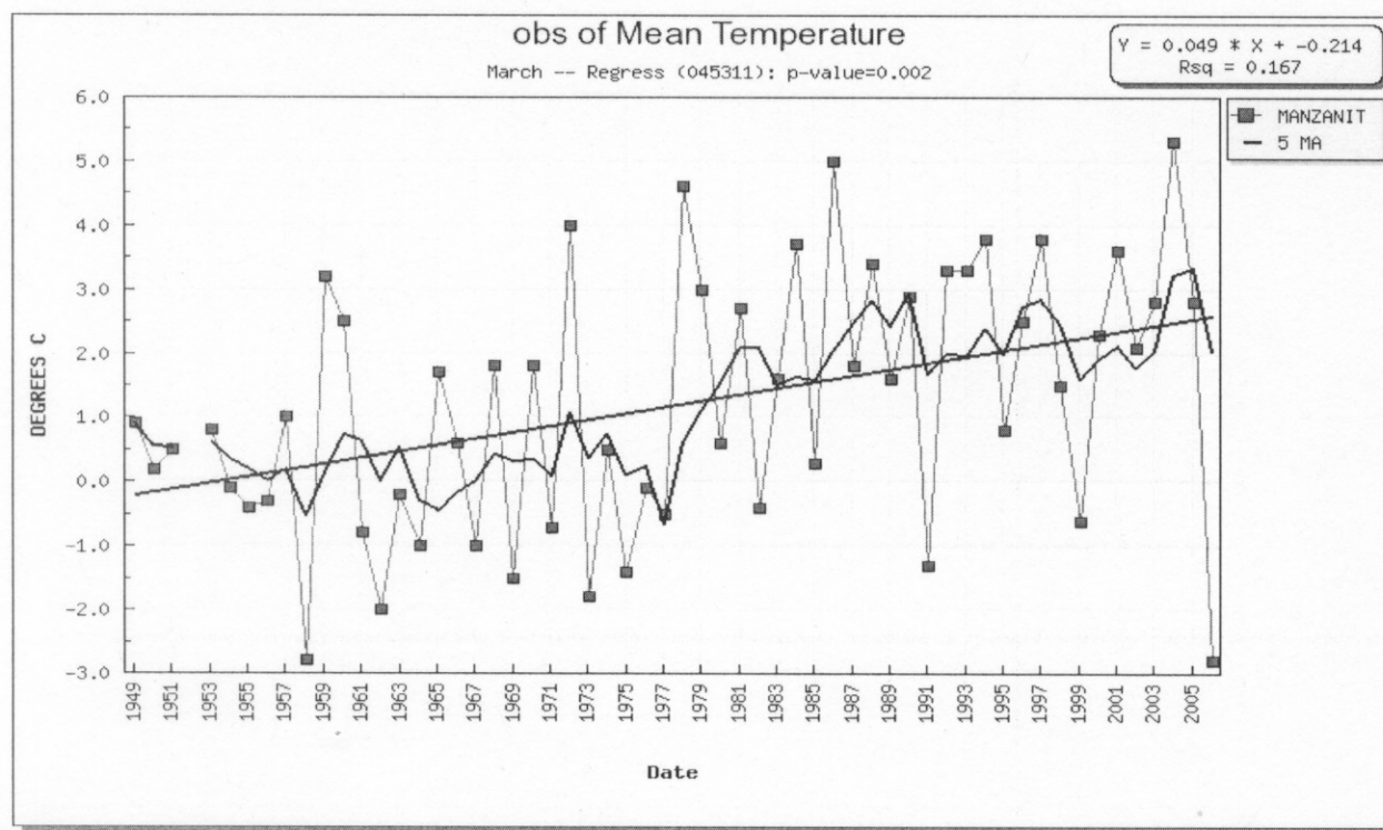
Figure 11. March mean temperature time series, 5 year moving average (black line), and least squares linear regression (blue line) for Manzanita Lake, 1949–2007 (045311). An increasing trend has occurred since the 1970s. March is the month leading up to the April 1 snow depth observations shown in Figure 10. (Date refers to year).
