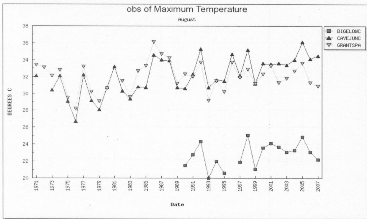
Figure 7. 1971–2007 August maximum temperature time series for Bigelow Camp, Cave Junction, and Grants Pass. Cave Junction has become increasingly warmer than Grants Pass since 1991. (Date refers to year).
