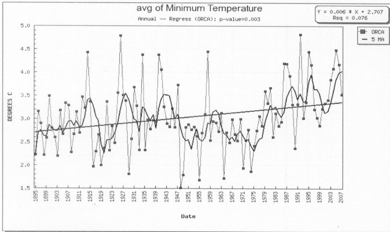
Figure 5. Mean annual minimum temperature time series, 5 year moving average (black line), and least squares linear regression (blue line) for Oregon Caves NM (ORCA) park average (PRISM modeled data). Strong warming has been occurring since the mid-1970s. (Date refers to year).
