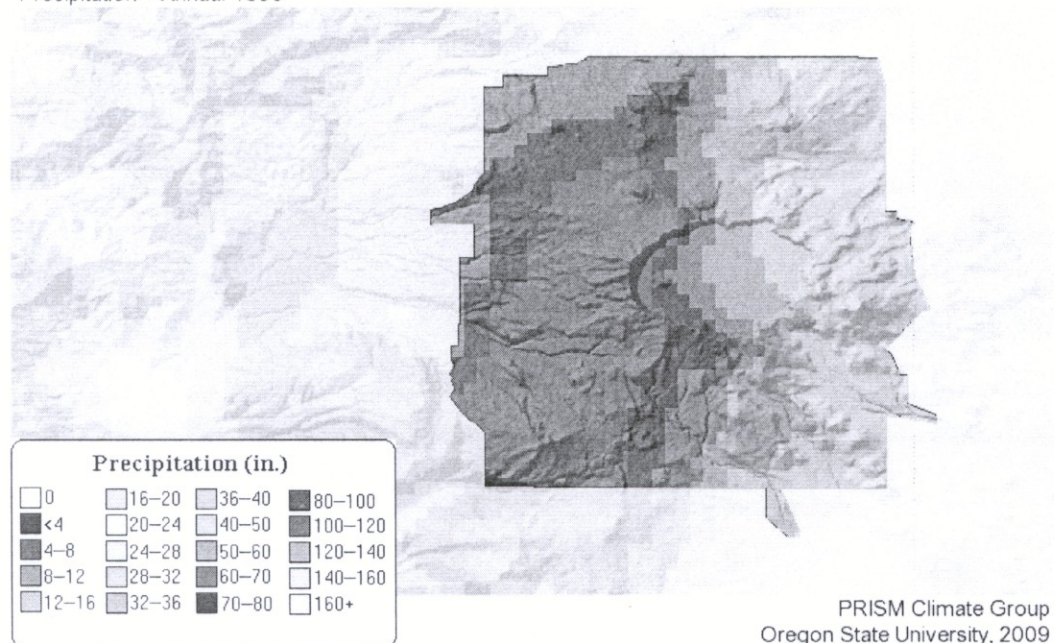
Figure 15. Screen capture of the Crater Lake annual precipitation map animation.
