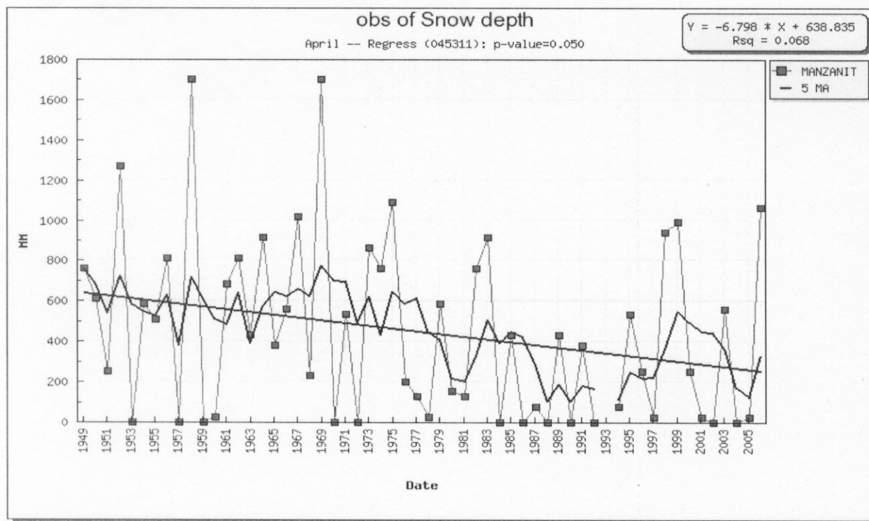
Figure 10. April 1 snow depth time series, 5 year moving average (black line), and least squares linear regression (blue line) for Manzanita Lake. A decreasing trend has occurred since the 1970s. See Figure 11 for related figure. (Date refers to year).
