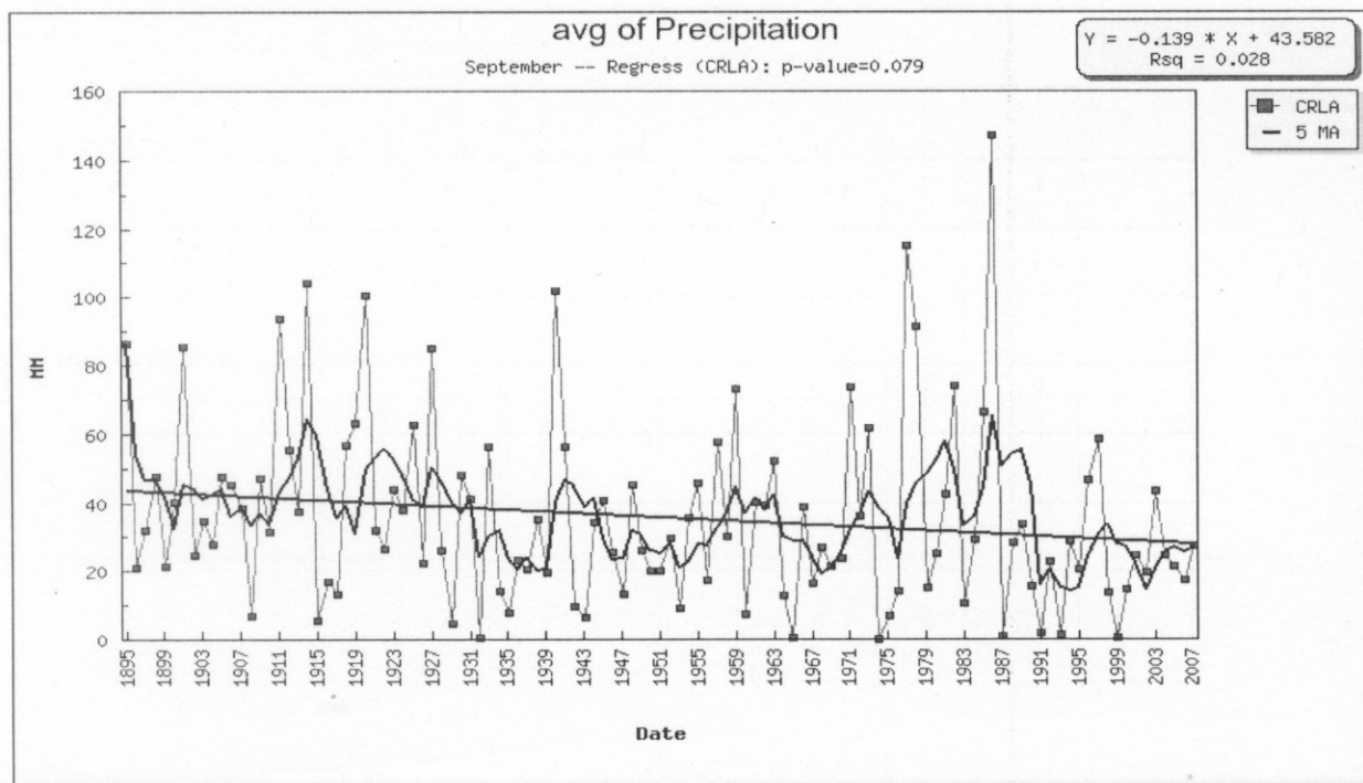
Figure 3. September precipitation time series, 5 year moving average (black line), and least squares linear regression (blue line) for Crater Lake (CRLA) park average (PRISM modeled data). Precipitation decreases markedly after 1986, and stays low through 2007. (Date refers to year).
