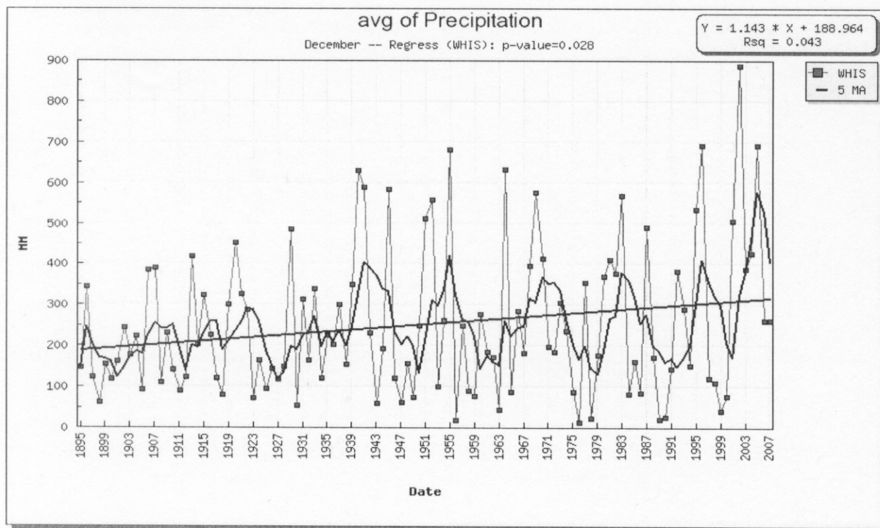
Figure 4. December precipitation time series, 5 year moving average (black line), and least squares linear regression (blue line) for Whiskeytown NRA (WHIS) park average (PRISM modeled data). Variations are cyclical, but precipitation has increased significantly in recent years. (Date refers to year).
