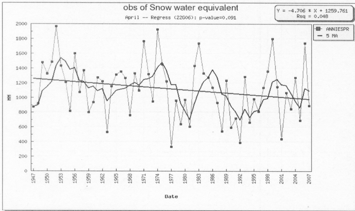
Figure 9. April 1 snow water equivalent time series, 5 year moving average (black line), and least squares linear regression (blue line) for Annie Spring snow course (1835 m), 4 km southwest of the Crater Lake Park HQ snow course. Despite close proximity and similar elevation, the decreasing trend conflicts with that of Park HQ (Figure 8). (Date refers to year).
