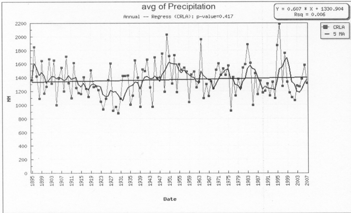
Figure 2. Mean annual precipitation time series, 5 year moving average (black line), and least squares linear regression (blue line) for Crater Lake (CRLA) park average (PRISM modeled data). There is little trend over the century. (Date refers to year).
