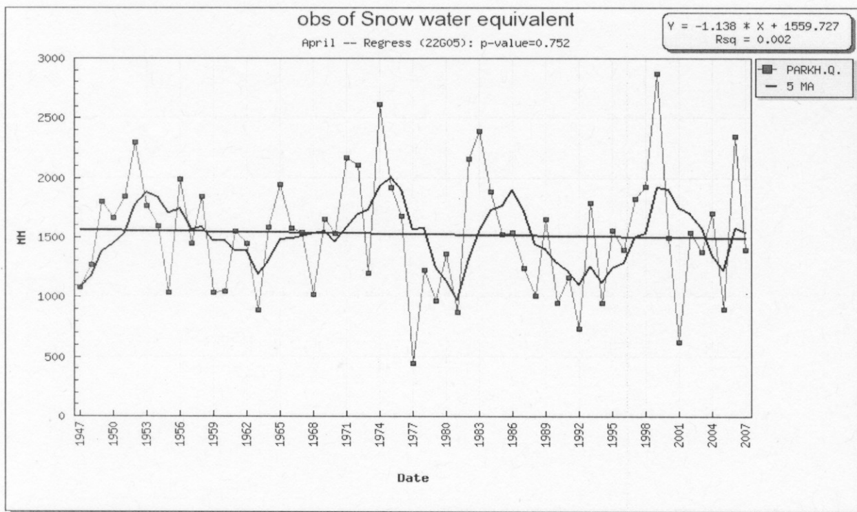
Figure 8. April 1 snow water equivalent time series, 5 year moving average (black line), and least squares linear regression (blue line) for Crater Lake Park HQ snow course (1996 m). Little overall trend is apparent. (Date refers to year).
