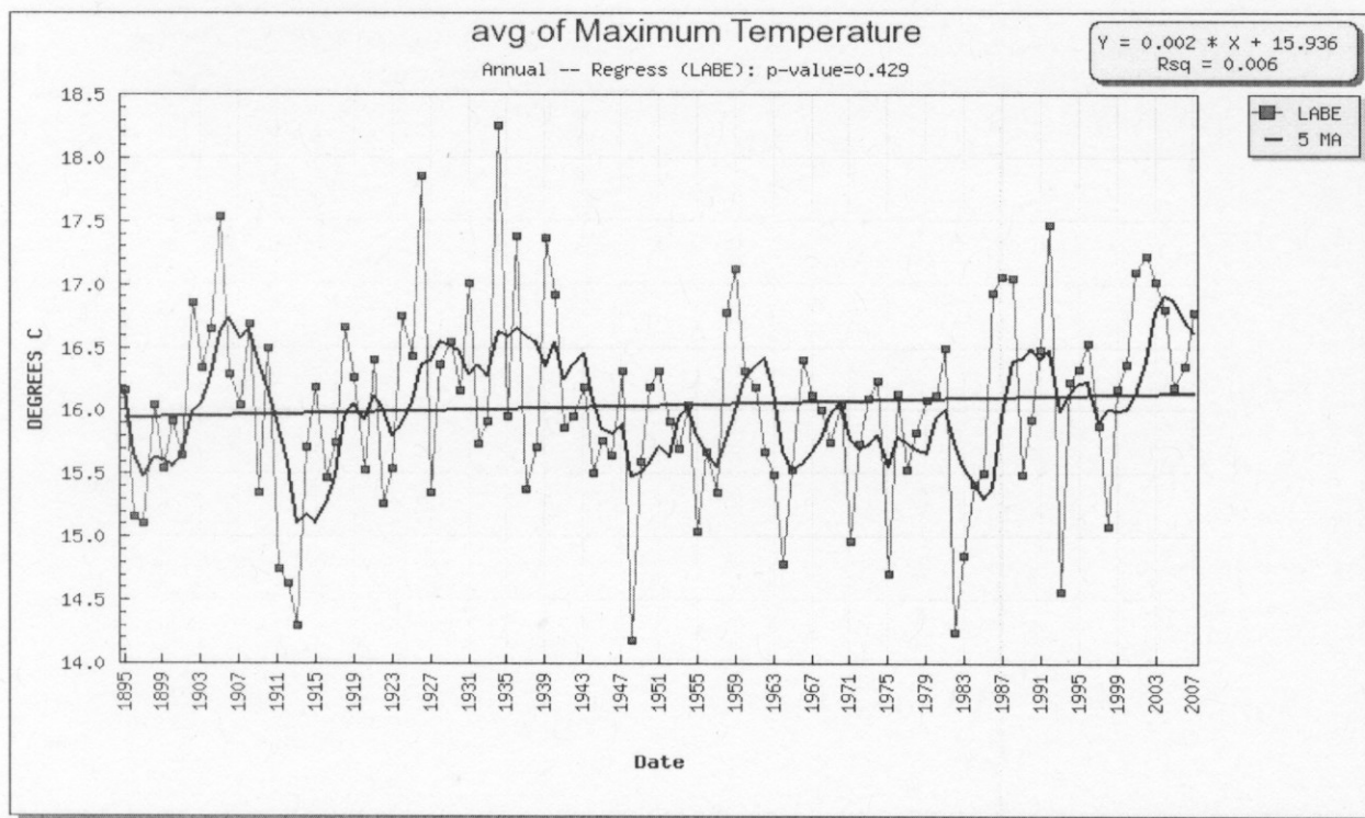
Figure 6. Mean annual maximum temperature time series, 5 year moving average (black line), and least squares linear regression (blue line) for Lava Beds NM (LABE) park average (PRISM modeled data). Little century-long trend is apparent. (Date refers to year).
