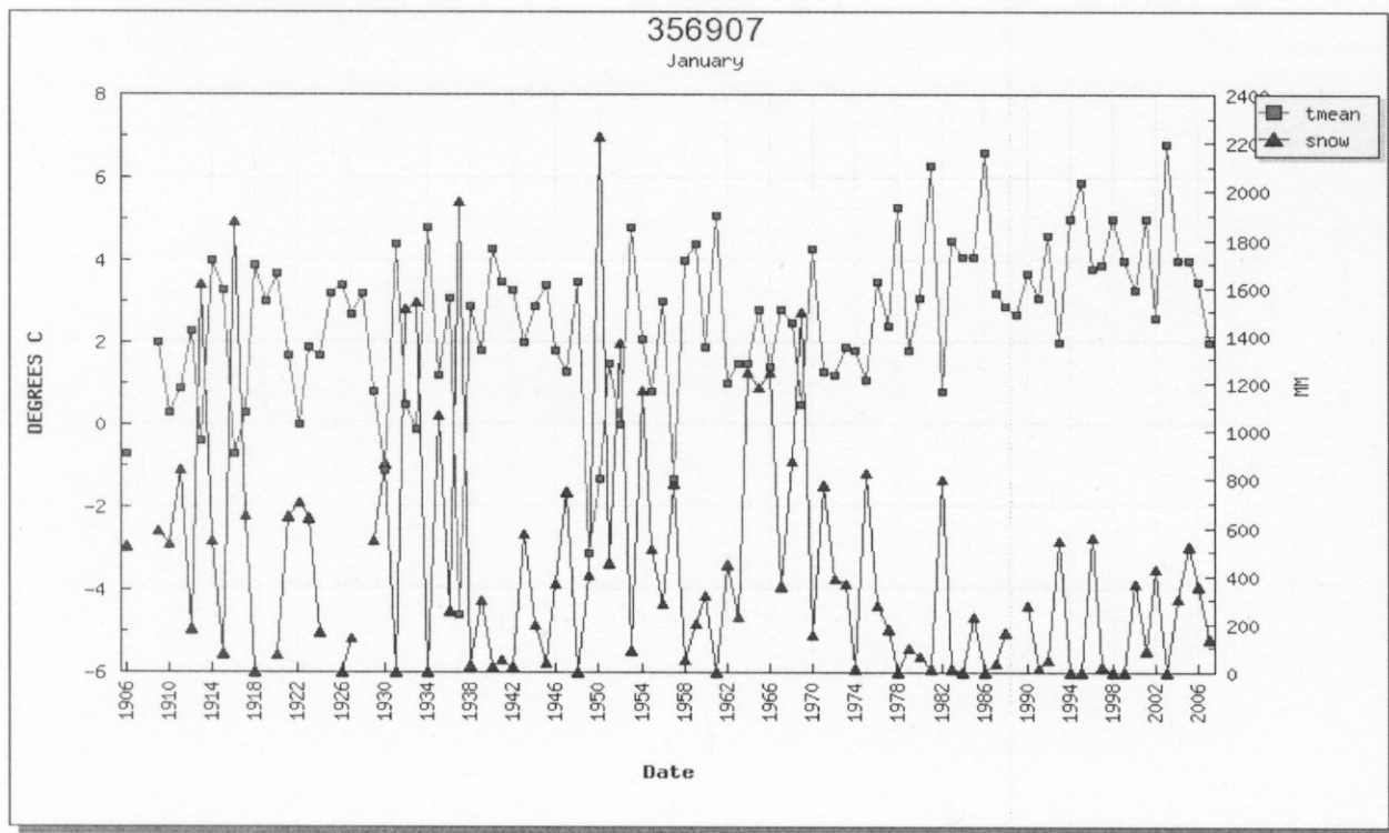
Figure 12. January mean temperature and snowfall for Prospect, OR (757 m), southwest of CRLA. Warming temperatures since 1970 correspond with a decrease in snowfall. (Date refers to year).
