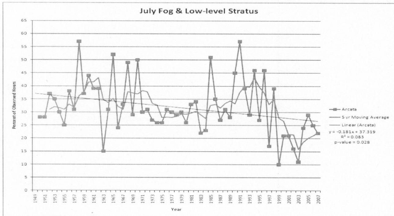
Figure 13. July observed fog & low-level stratus time series, 5 year moving average (blue line), and least squares linear regression (black line) for Arcata. Fog and low stratus has been decreasing over the past 20 years.
