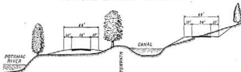
TYPICAL SINGLE ROADWAY
