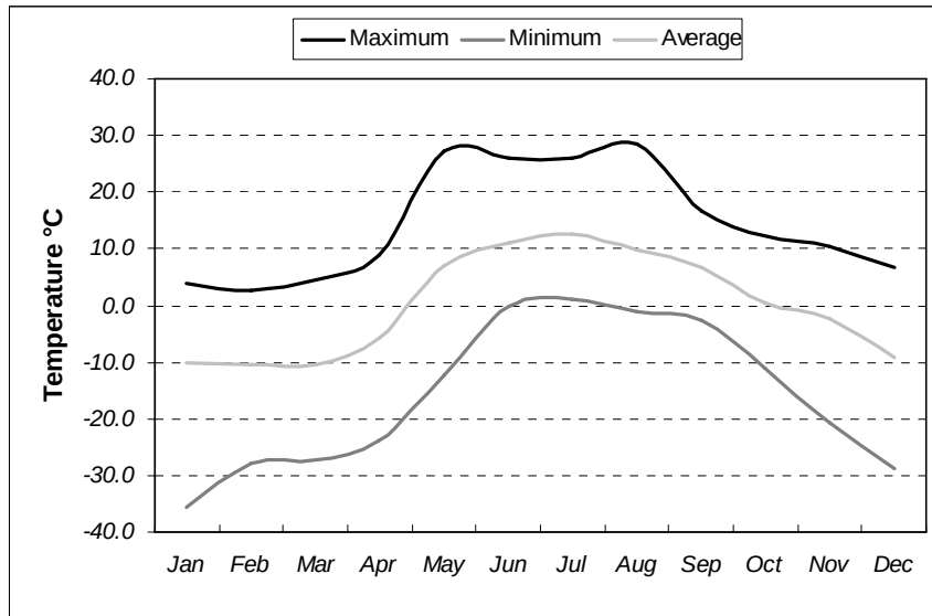
Figure 5 Air temperatures –headquarters
