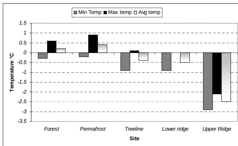
Figure 15 Yearly average minimum, average maximum and average temperatures
