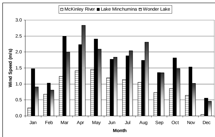
Figure 13 Mean monthly wind speeds at three north side RAWS sites
