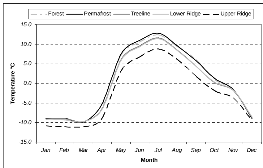
Figure 14 Mean monthly temperatures Rock Creek sites
