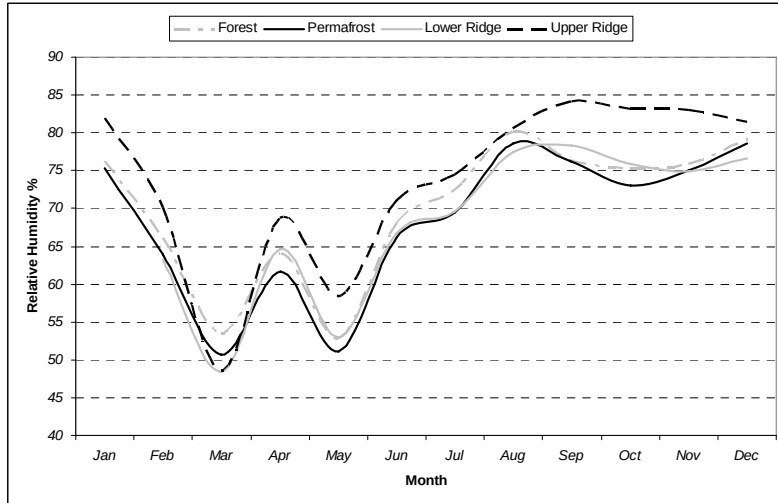
Figure 16 Mean monthly relative humidity values for the Rock Creek sites
