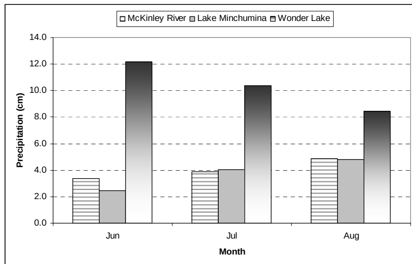
Figure 12 Summer precipitation totals at the three north side RAWS sites
