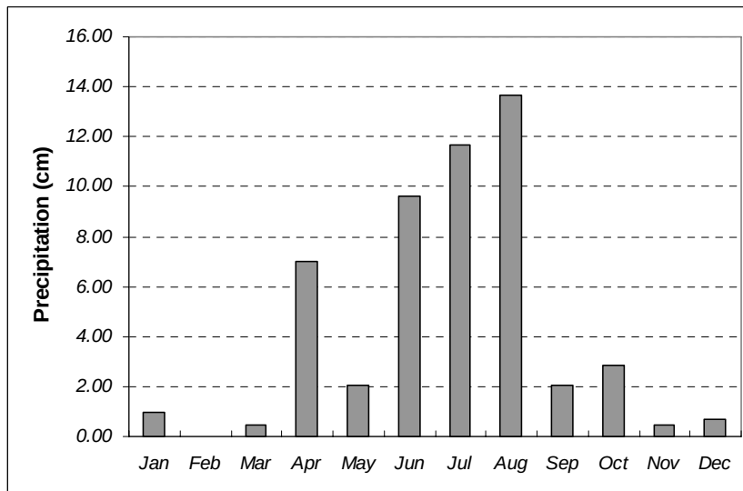
Figure 6 Monthly precipitation totals - Park headquarters
