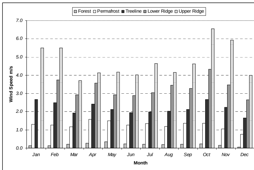
Figure 17 Mean monthly wind speeds - Rock Creek sites
