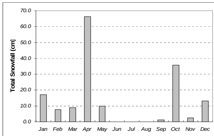
Figure 7 Monthly snowfall totals - Park headquarters
