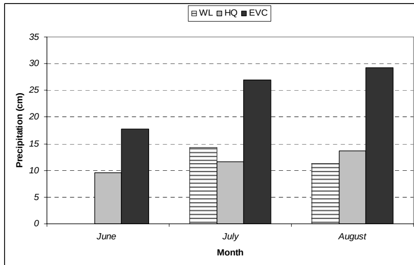
Figure 9 Summer precipitation totals for Wonder Lake, Eielson Visitor Center, and Park headquarters
