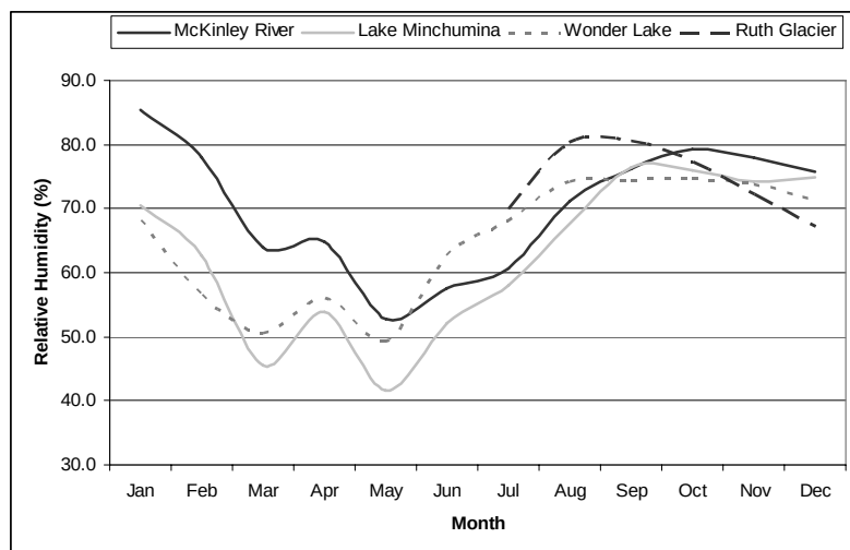
Figure 11 Mean monthly relative humidity at the RAWS sites.
