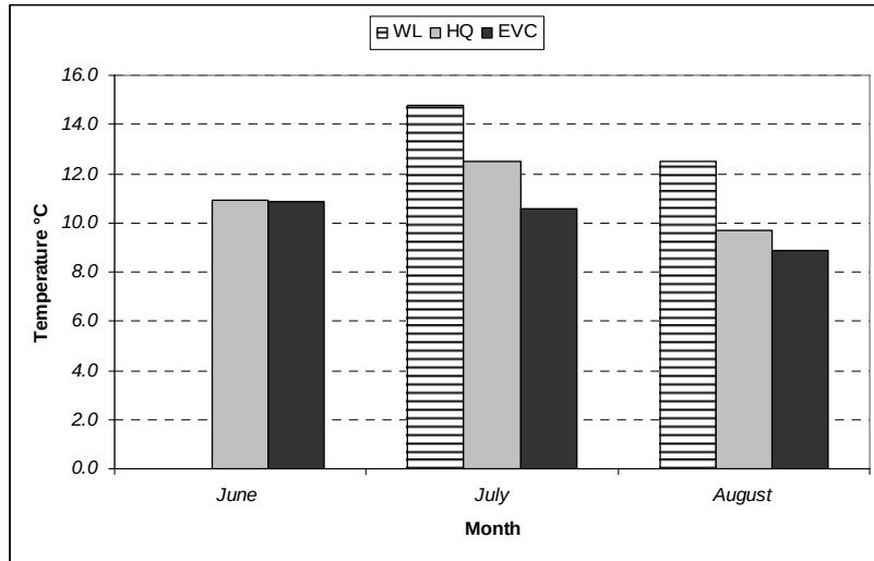
Figure 8 Summer temperatures at Wonder Lake, Eielson Visitor Center, and Park headquarters
