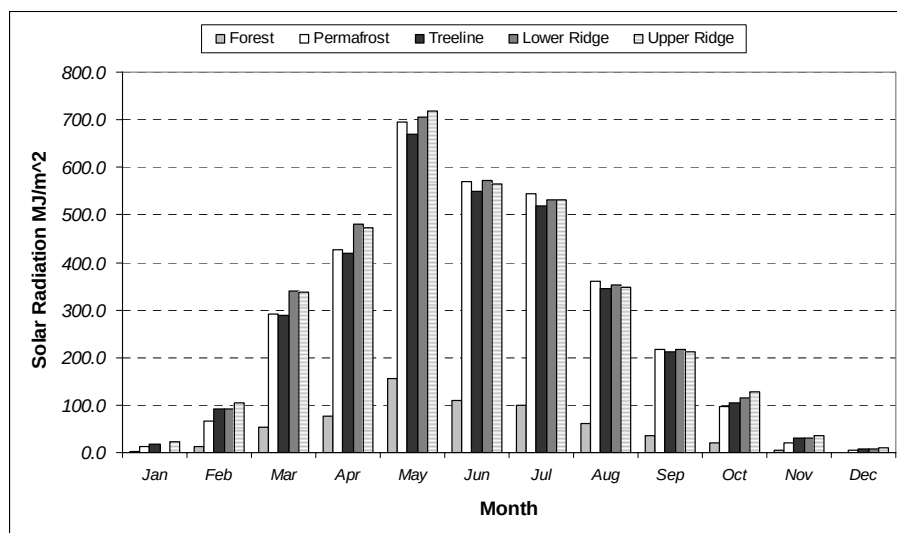
Figure 19 Monthly solar radiation values for Rock Creek Sites
