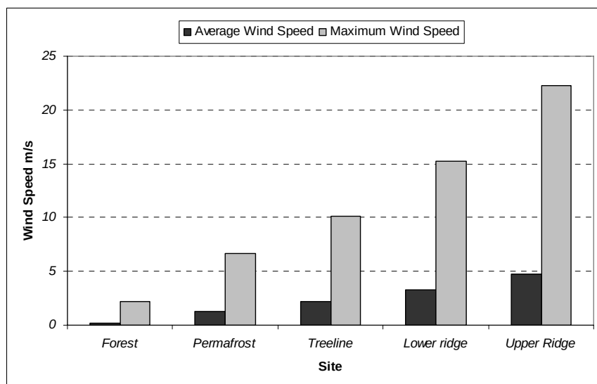
Figure 18 Average and peak wind speeds Rock Creek sites
