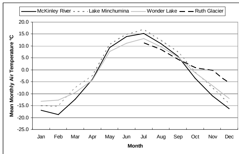
Figure 10 Mean monthly air temperatures (°C) for the 4 RAWS sites.
