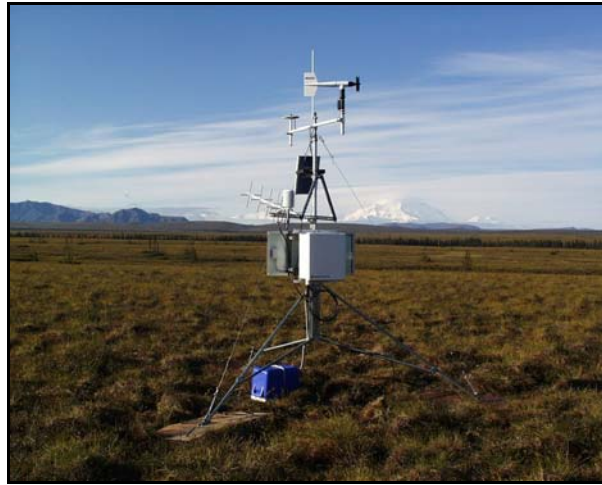
Figure 9. CAKN climate station, remote testing Denali National Park and Preserve
