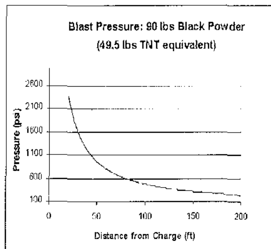
Figure 9.5. Blast pressure.
