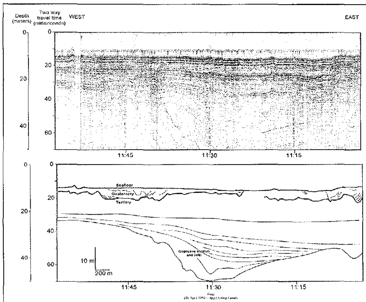
Figure 9.2. Deep penetrating sub-bottom profile of nearby sediments.
