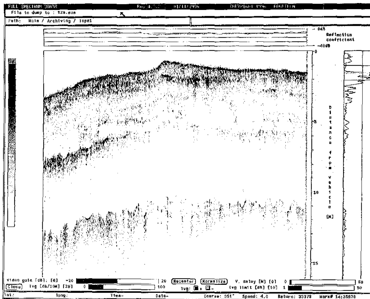
Figure 9.4. Data screen of EdgeTech sub-bottom profiler over Hunley site.
