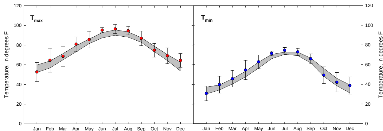
Figure 2. Average monthly air temperature during 2011 and the 30-year (1981 – 2010) average for Columbia Metro Airport station. Units = °F. Points indicate the 2011 average monthly maximum and minimum temperatures. Error bars indicate +/- standard deviation. The dual solid lines bound the standard deviation around the 30-year (1981-2010) mean monthly temperature.
