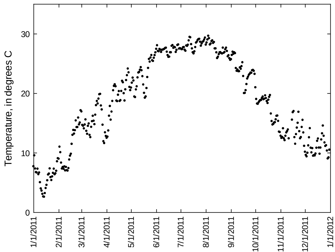
Figure 6. Mean daily water temperature on Cedar Creek (CONGccbr) in Congaree National Park during 2011.
