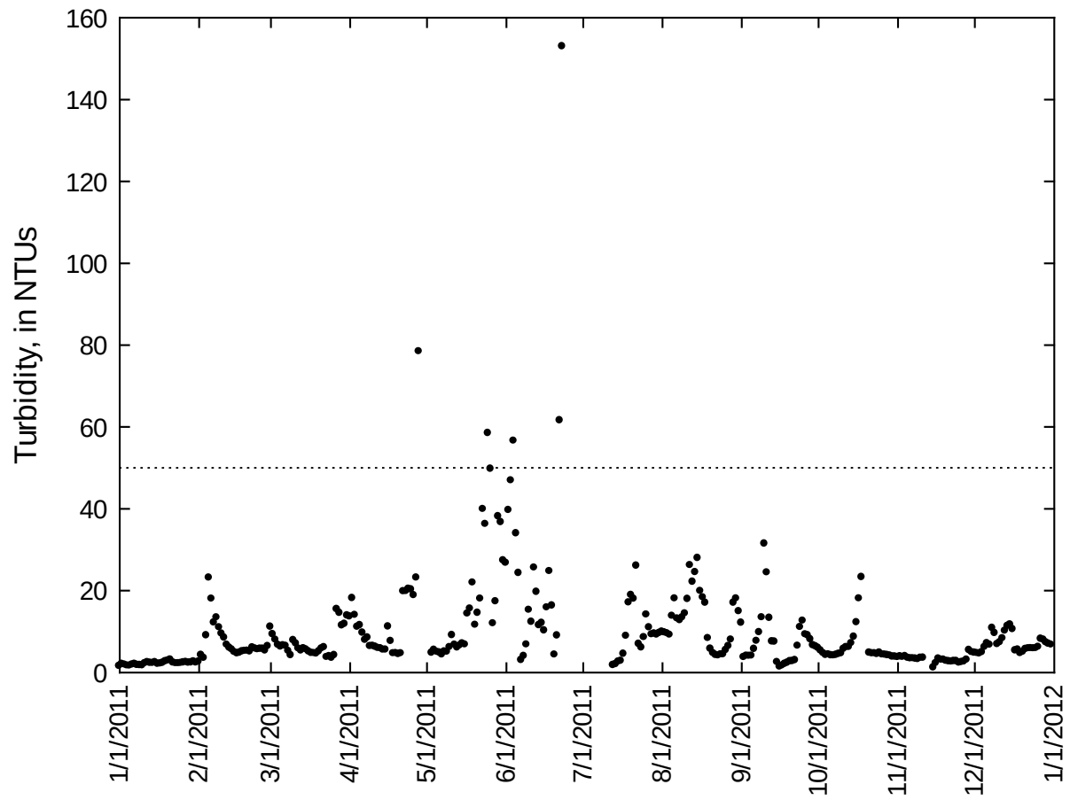
Figure 10. Mean daily turbidity on Cedar Creek in Congaree National Park during 2011. Dotted line indicates the South Carolina standard of 50 NTUs for maximum turbidity levels in freshwater.
