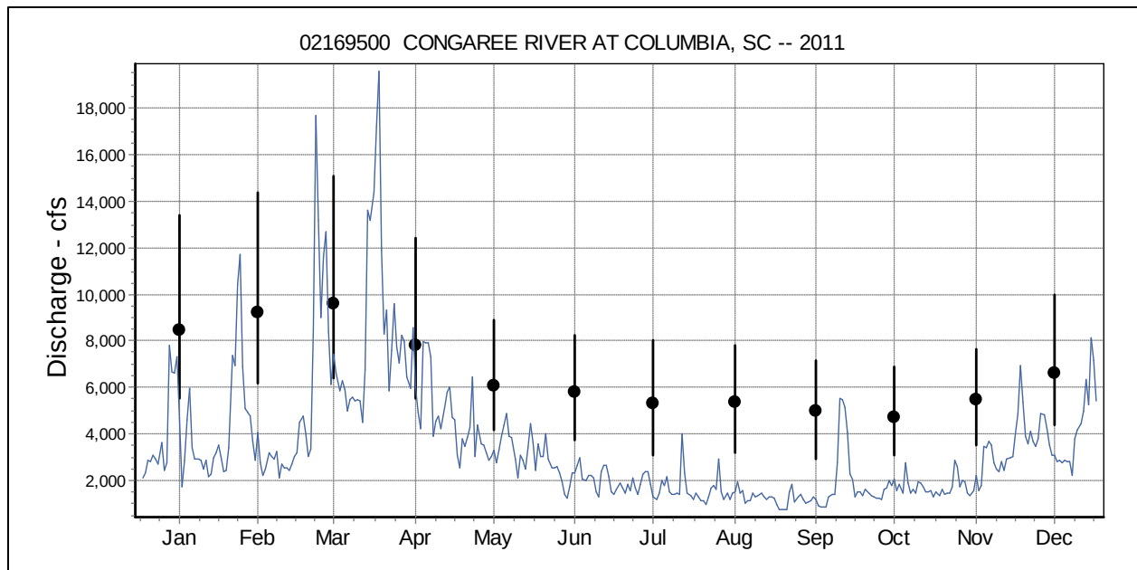
Figure 4. Daily flow (blue line), historical median monthly flow (dots), and interquartile range (error bars) for the Congaree River at Columbia, SC (USGS 02169500) in 2011 (from Jones and Gregory 2012).
