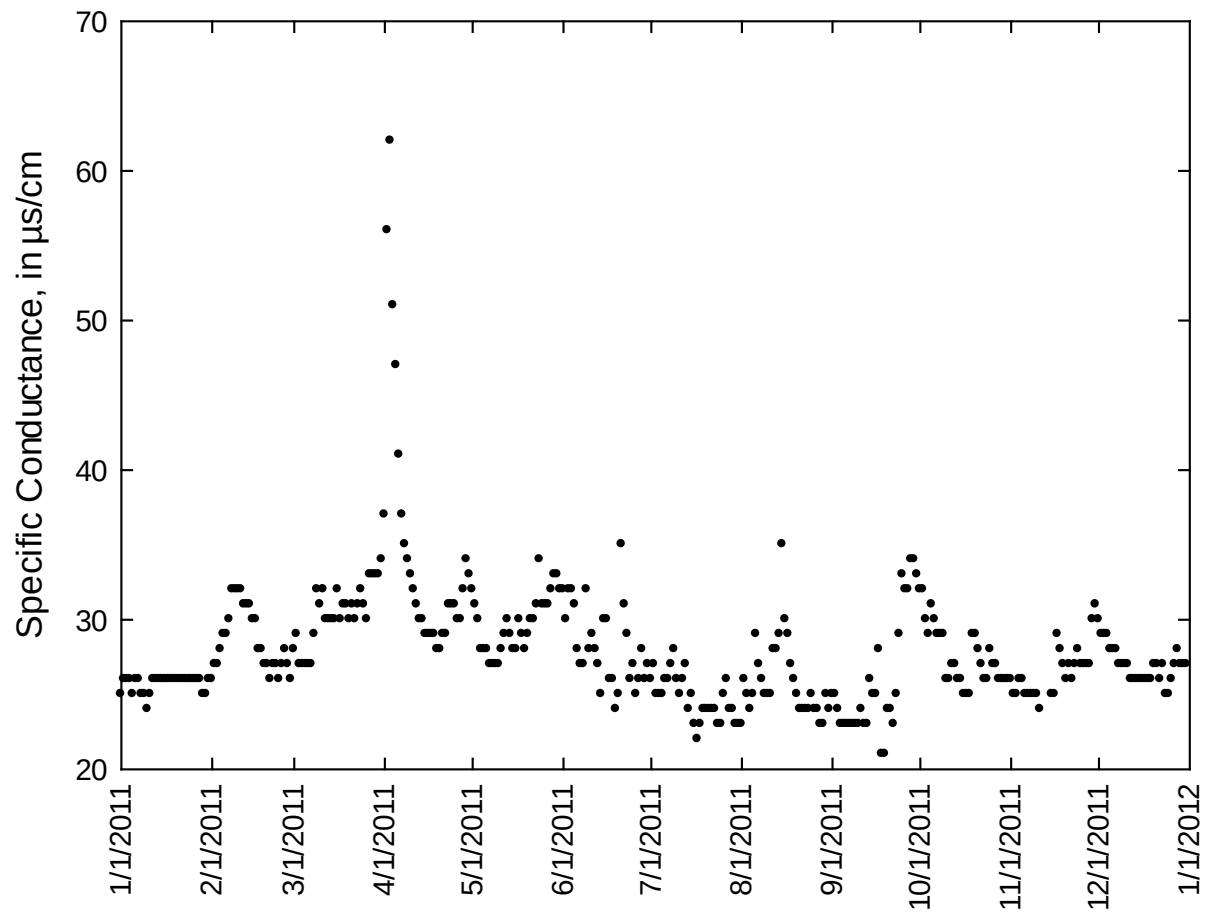
Figure 7. Mean daily specific conductance on Cedar Creek (CONGccbr) in Congaree National Park during 2011.
