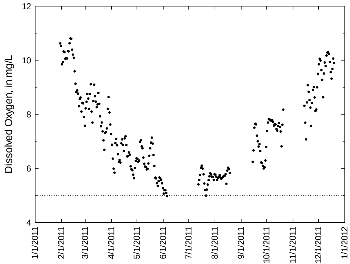
Figure 8. Mean daily dissolved oxygen on Cedar Creek (CONGccbr) in Congaree National Park during 2011. Dotted line indicates the South Carolina standard of 5 mg/L for minimum average daily dissolved oxygen concentrations in freshwater.
