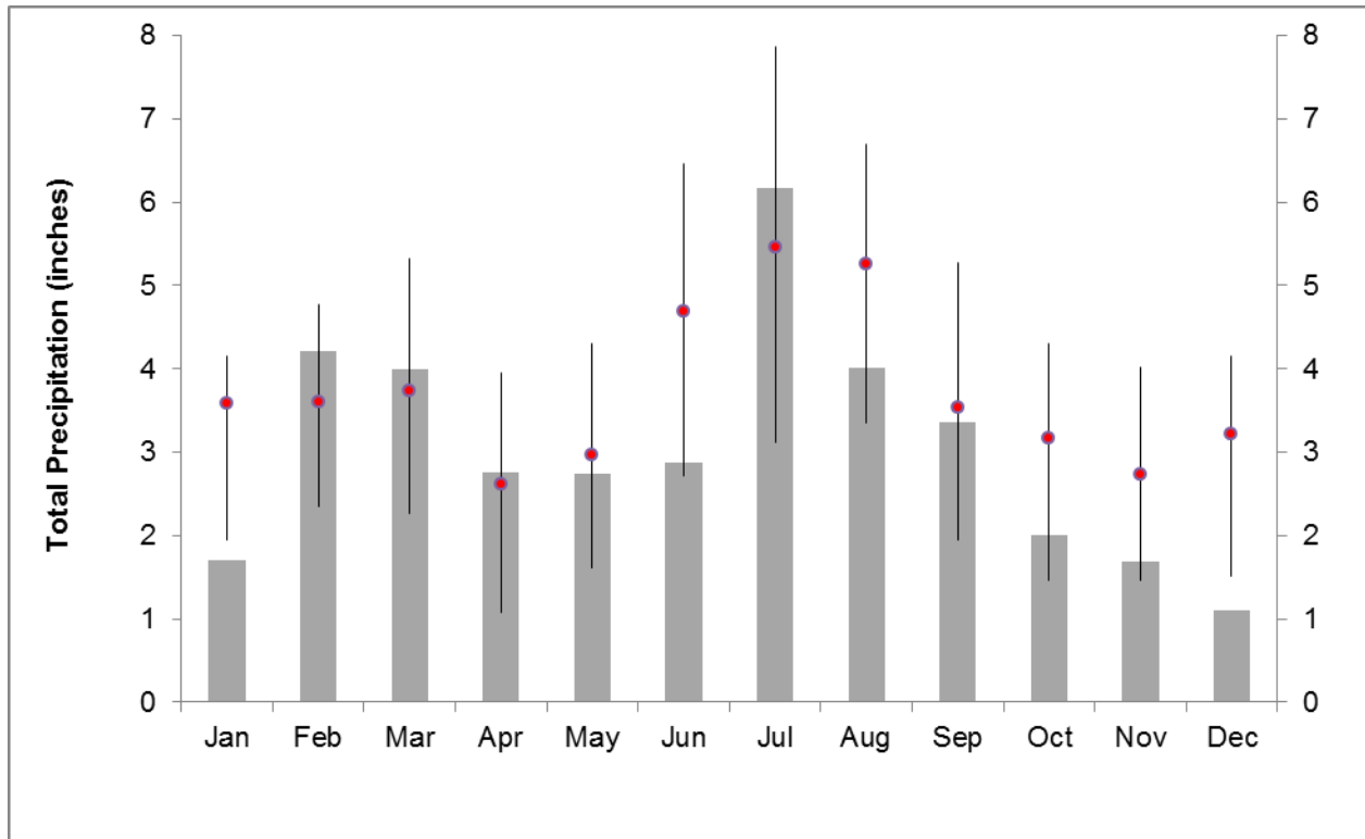
Figure 3. Total monthly precipitation during 2011 and the 30-year (1981 - 2010) monthly averages for Columbia Metro Airport station. The gray columns represent 2011 total monthly precipitation. The red circles represent the 30-year average; the lines indicate the 25th and 75th percentile of the 30-year normal data for each month.
