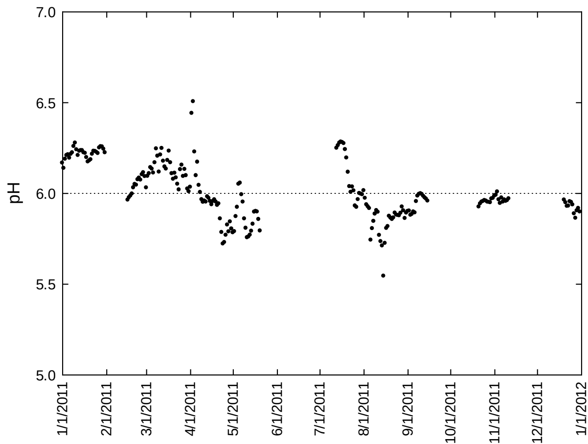
Figure 9. Mean daily pH on Cedar Creek (CONGccbr) in Congaree National Park during 2011. Dotted line indicates the South Carolina standard of 6 for minimum pH levels in freshwater.
