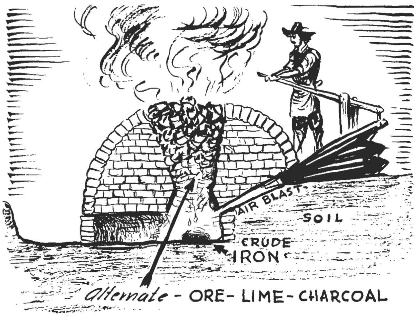
HOW AN IRONWORKING PIT WAS USED. ( From contemporary sources. )
