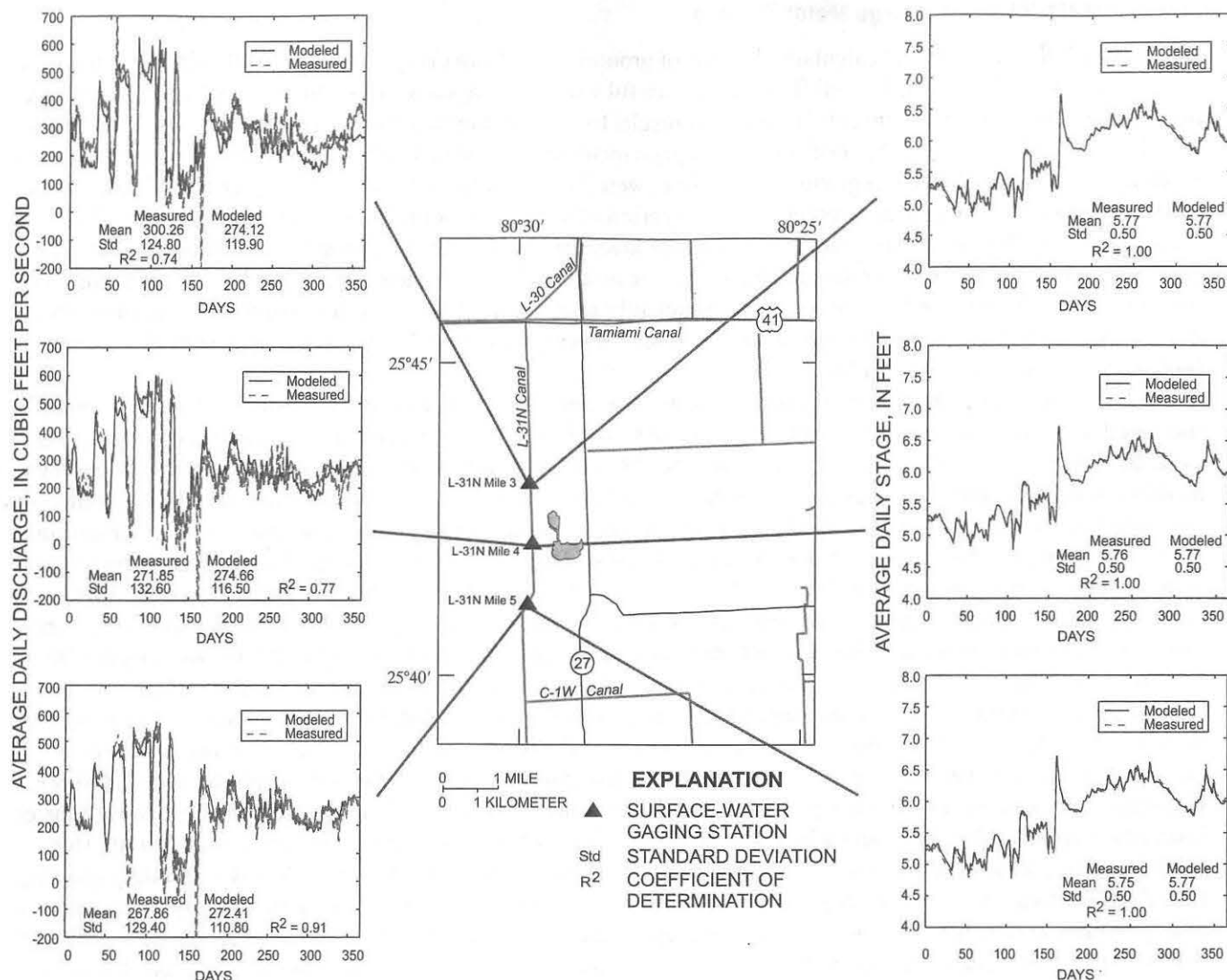
Figure 25. Measured and modeled canal stage and discharge obtained by the reach-transmissivity version of MODBRANCH for the verification run.
