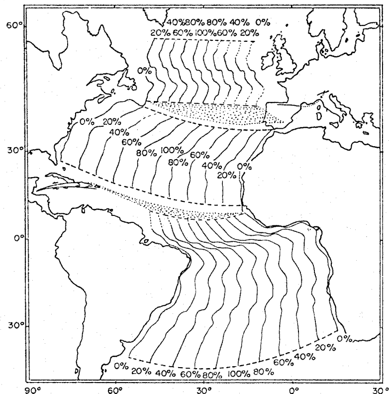
FIGURE 16. Successive positions of the three join-segments (from Figure 2 of Funnell & Smith, 1968) rotated by angular increments of 10 per cent between continents, representing limits of 20 per cent stages of opening. Limits of northern and southern transverse zones indicated by dashed lines, and amount of north-south extension by stipple. Principal fundamental and wrench faults indicated for Mediterranean and Caribbean orogenic belts. (Mercator projection.) (Adapted from Funnell & Smith, 1968.)
