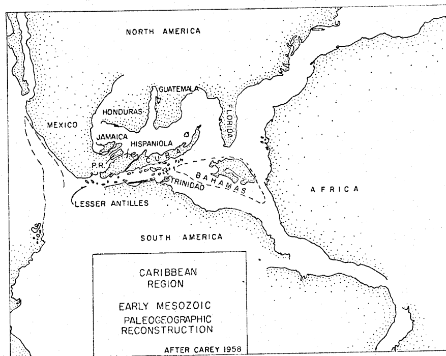
FIGURE 15. Early Mesozoic paleogeographic reconstruction of the Caribbean. (After Carey, 1958.)
