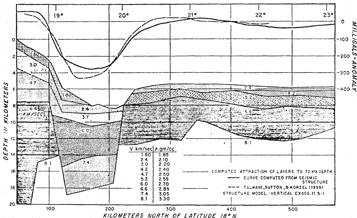
FIGURE 12. Upper, comparison of computed free-air anomaly (solid line) and measured anomaly (dashed line) for a cross section from Puerto Rico to Nares Basin (see Fig. 11). Lower, crustal layer model and assigned densities for computed total attraction (free-air anomaly). (From Bunce & Fahlquist, 1962.)
