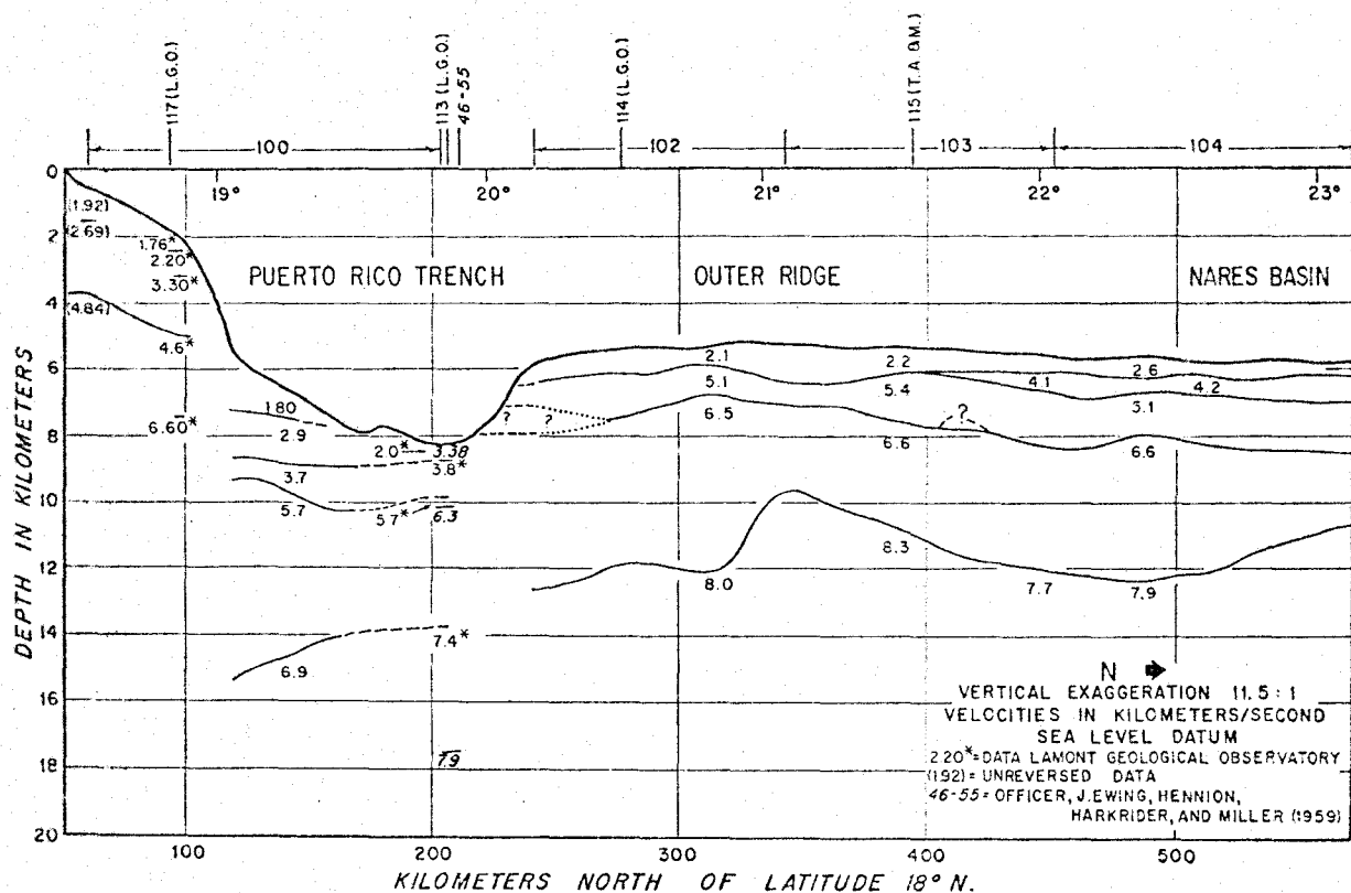
FIGURE 11. Structural section, Puerto Rico Trench to Nares Basin along longitude 66°33'W. (From Bunce & Fahlquist, 1962.)
