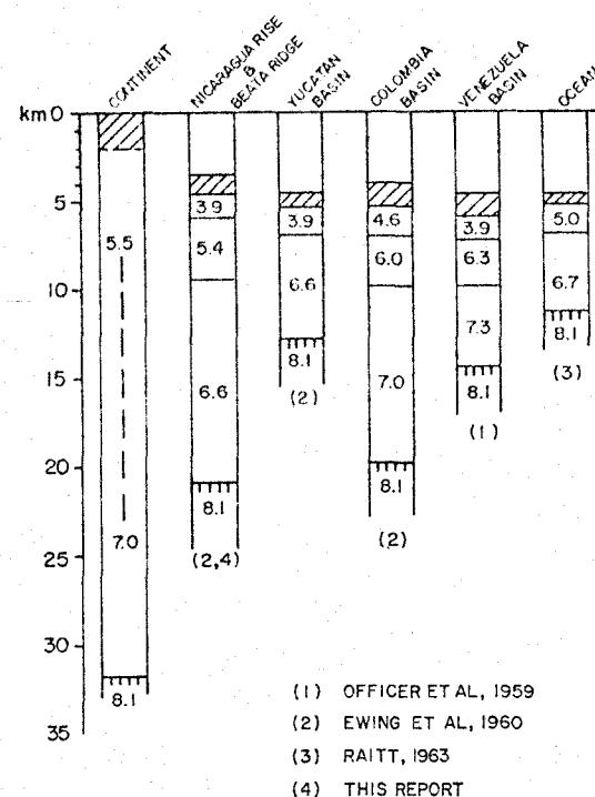
FIGURE 7. Crustal sections. (From Edgar, 1968.)
