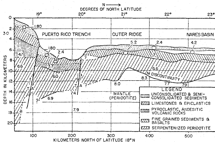
FIGURE 13. Structural section, Puerto Rico Trench to Nares Basin along longitude 66°33'W. Velocities are given in km/sec. Vertical exaggeration 11.5:1. (After Glover [1967], as adapted from Bunce & Fahlquist [1962], with modifications by Glover, based in large part upon observations and interpretations by Hersey [1962], Hess [1964], Bowin and others [1966].)
