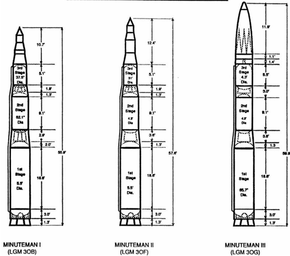
Plate 12. Line drawings showing the evolution of the Minuteman ICBM ( Lonnquest and Winkler, To Defend and Deter: The Legacy of the United States Cold War Missile Program , 243)
