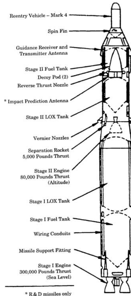
Plate 7. Drawing of Titan I, the United States' first two-stage ICBM ( Lonngquest and Winkler, To Defend and Deter: The Legacy of the United States Cold War Missile Program , 228)
