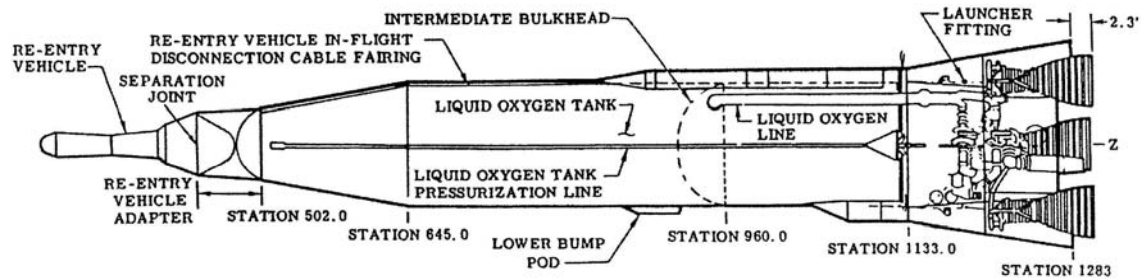
Plate 6. Cutaway drawing of an Atlas D ICBM. Later Atlas E and F missiles used the same airframe but added more powerful engines ( John C. Lonngquest and David F. Winkler, To Defend and Deter: The Legacy of the United States Cold War Missile Program (Washington, D.C.: Department of Defense, Legacy Resource Management Program, 1996), 210)
