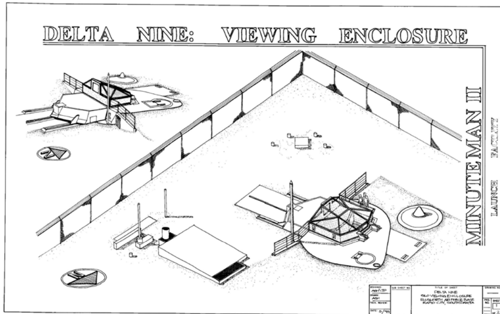
Plate 86. Line drawing of Delta-09 viewing enclosure (Courtesy of the 28 th Civil Engineer Squadron, Ellsworth Air Force Base)
