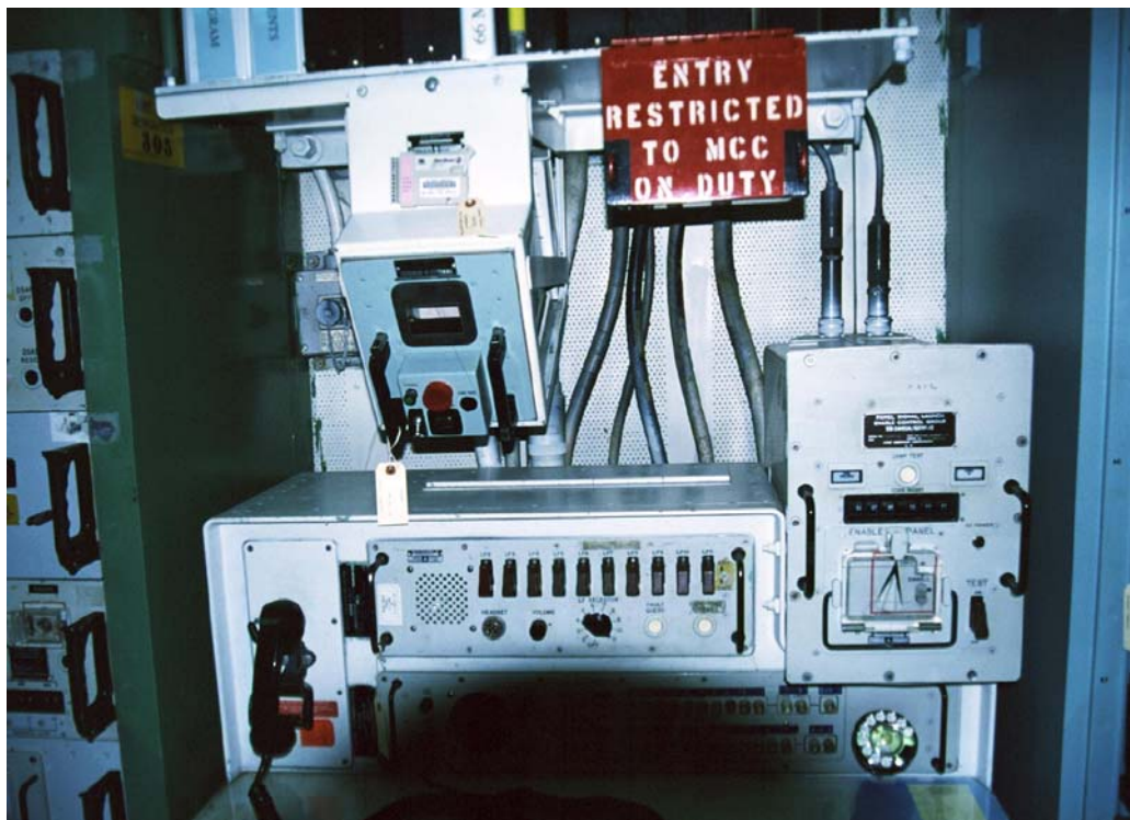
Plate 65. Deputy Commander Control Console, Launch Control Center, Delta-01 (Photograph by Mead & Hunt)
