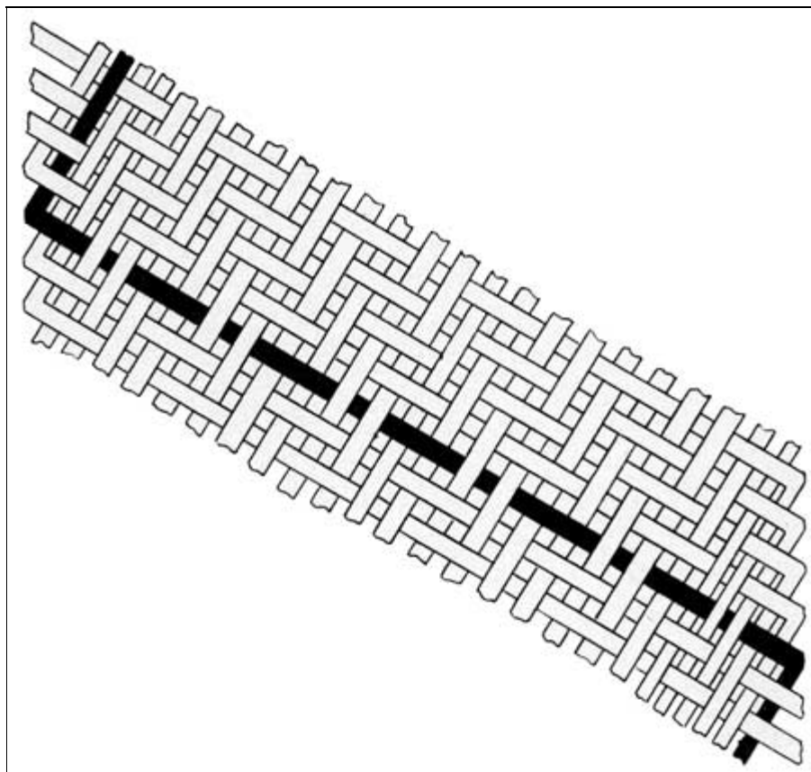
Figure 27. Detail of braid, Sandal, No. 45
