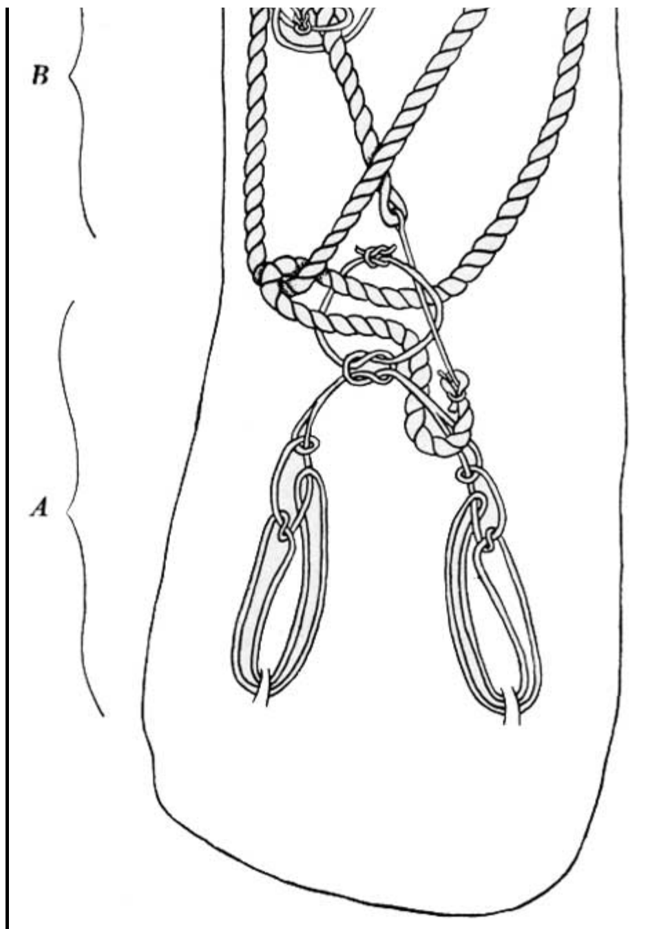
Figure 28. Specimen No. 27, showing toe and heel tie attachment
