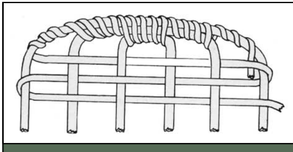
Figure 28. Specimen No. 27, showing toe and heel tie attachment
