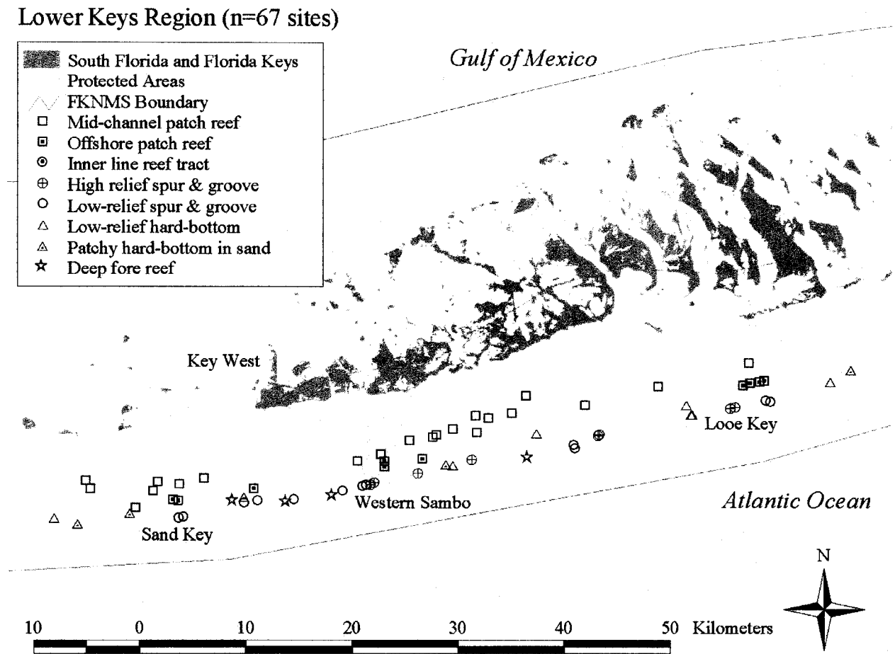
Figure 2. Survey locations in the lower Florida Keys region by habitat type.
