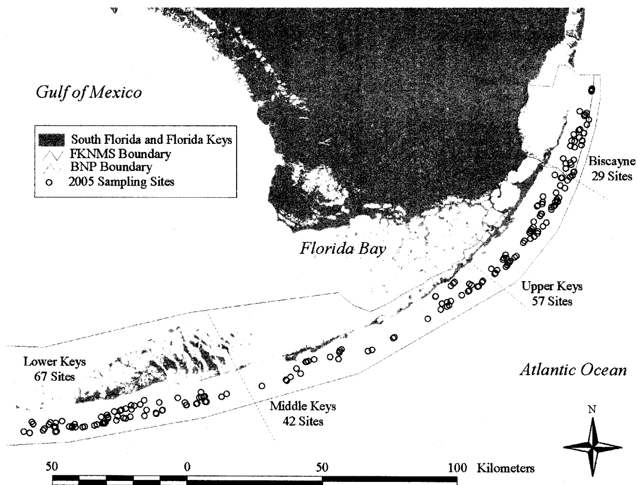
Figure 1. Survey locations in the southeast Florida region from northern Biscayne National Park to southwest of Key West.
