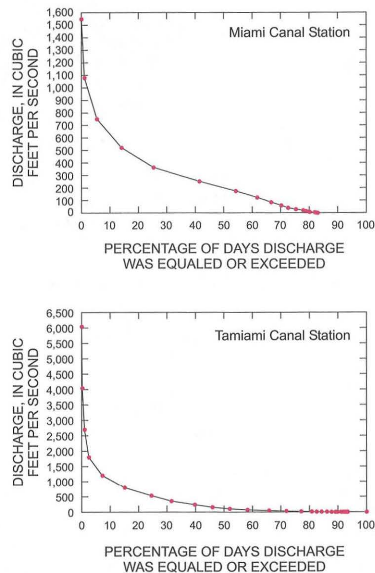
Figure 3. Flow-duration curves for the Miami and Tamiami Canal stations. Valid only for positive discharges.
