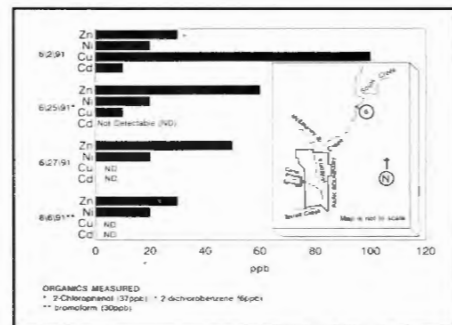
Figure 5. Location of biomonitoring site 6 with respect to Wilson's Creek National Battlefield Park, Missouri. In previous studies, site 6 was chronically toxic to daphnids. By using Toxicity Identification Evaluation (TIE) procedures, combinations of zinc (Zn), nickel (Ni), and copper (Cu) were judged to be responsible for the toxicity.
