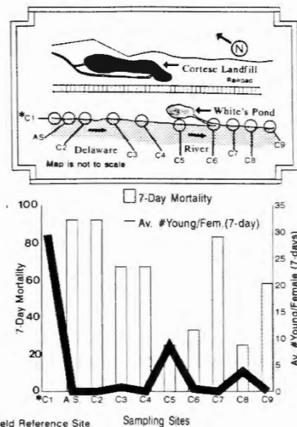
Figure 4. Biomonitoring sample sites of leachates entering the Delaware River (Upper Delaware Scenic and Recreational River, New York) below a Superfund landfill. Data shown in the bar graph represent the 7-day mortality of the test species, Ceriodaphnia dubia , and the line graph represents the average number of young produced per female dubia that survived the exposure after 7 days.
